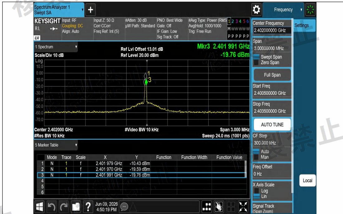
NTNV-3DH5-Ant1-2402-PASS
