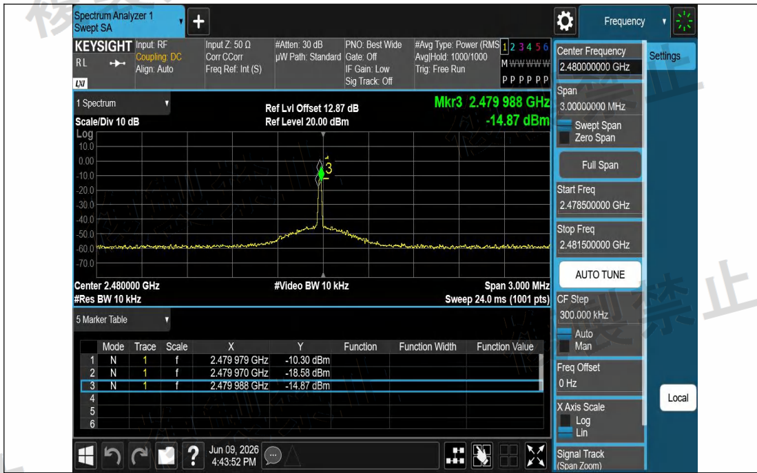
NTNV-DH5-Ant1-2480-PASS
