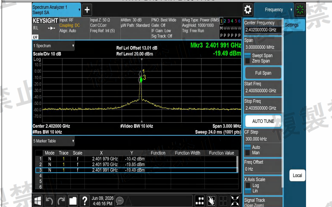
NTNV-2DH5-Ant1-2402-PASS
