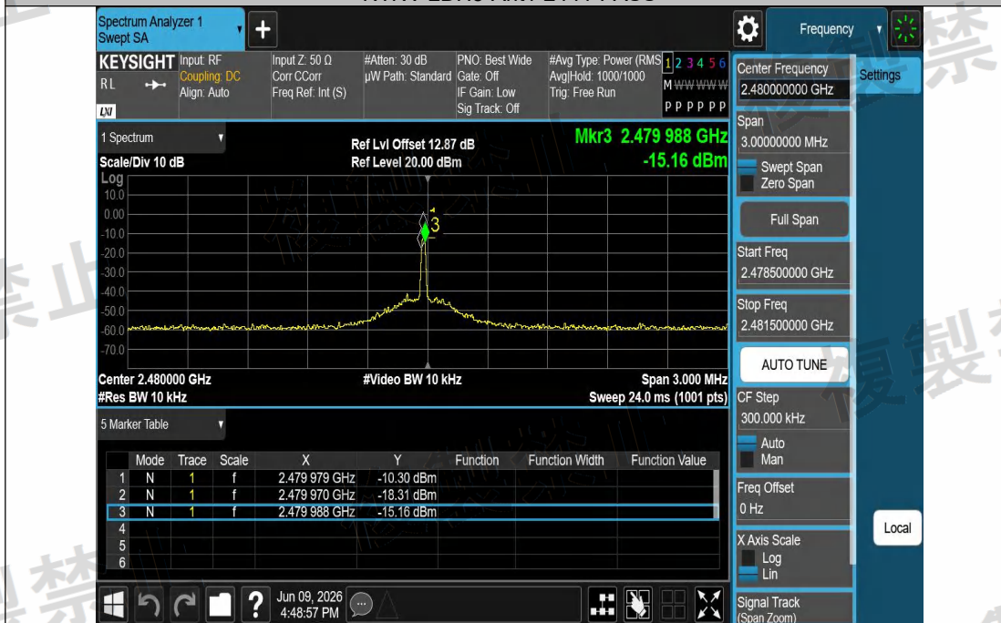
NTNV-2DH5-Ant1-2480-PASS
