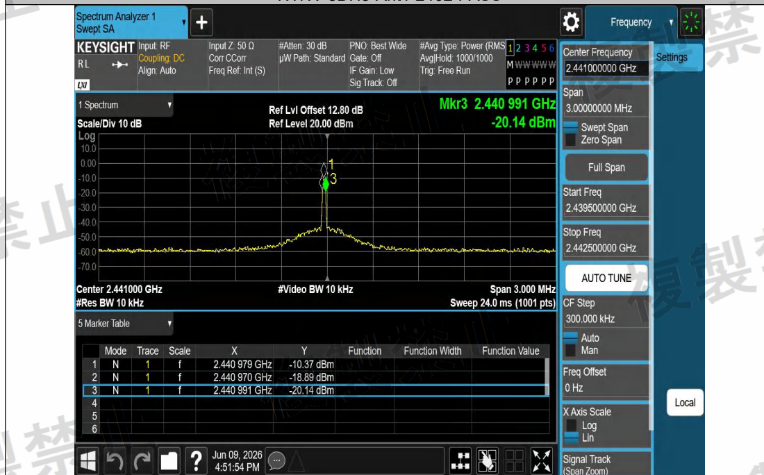
NTNV-3DH5-Ant1-2441-PASS
