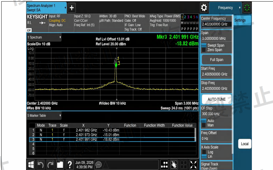
NTNV-DH5-Ant1-2402-PASS
