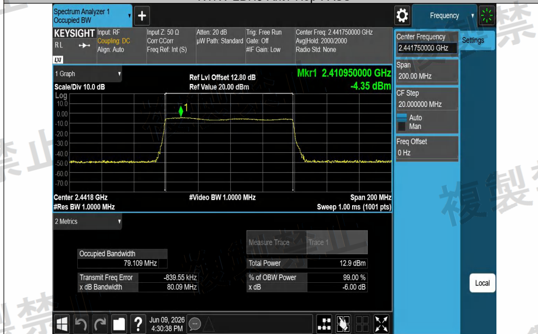
NTNV-3DH5-Ant1-Hop-PASS
