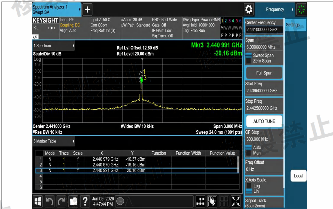
NTNV-2DH5-Ant1-2441-PASS
