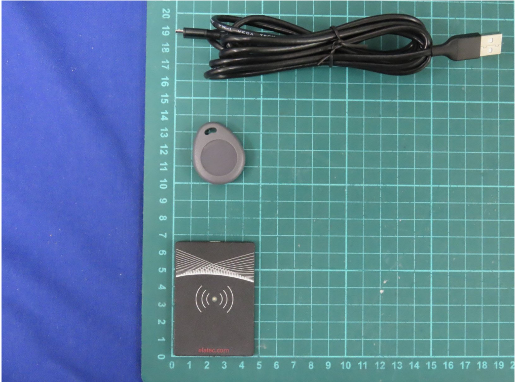
(1) EUT Photo – Trade Name: ELATEC, M/N: TWN4 Slim LEGIC
