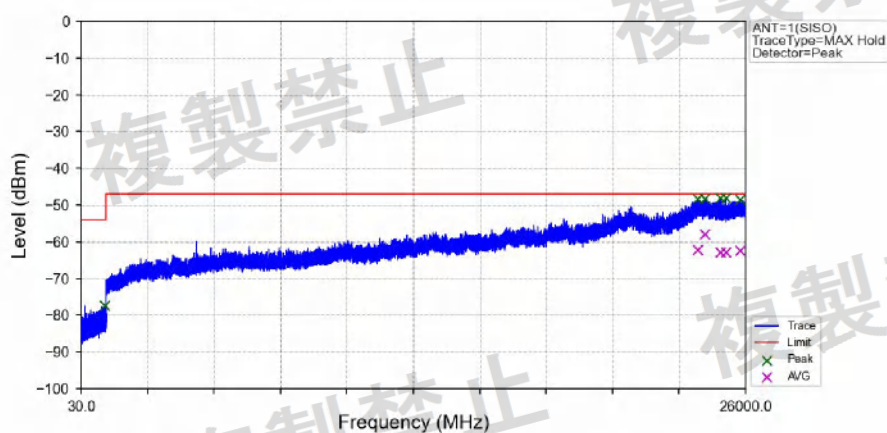
802.11ac(VHT40)_MCH_5590MHz_Ant1_NTNV
