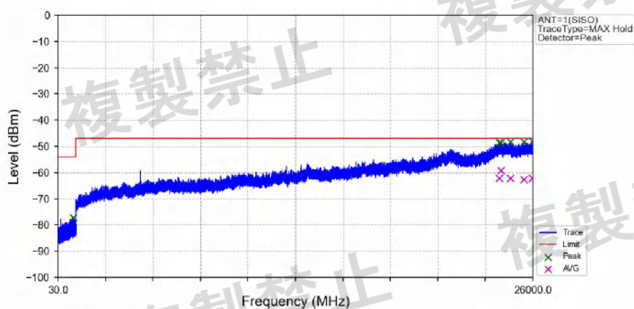
802.11ac(VHT20)_MCH_5300MHz_Ant1_NTNV
