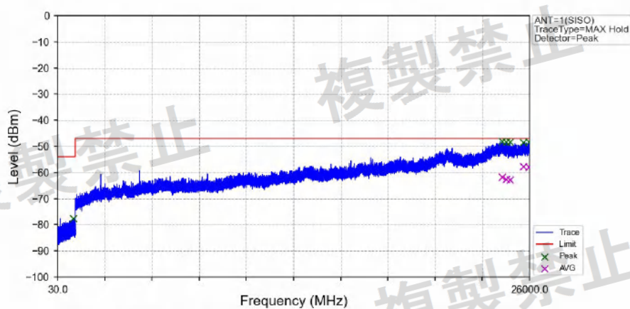
802.11ax(HEW40)_HCH_5670MHz_SU_/_Ant1_NTNV
