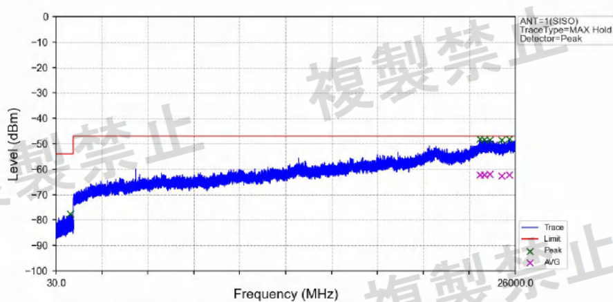
802.11n(HT20)_MCH_5200MHz_Ant1_NTNV
