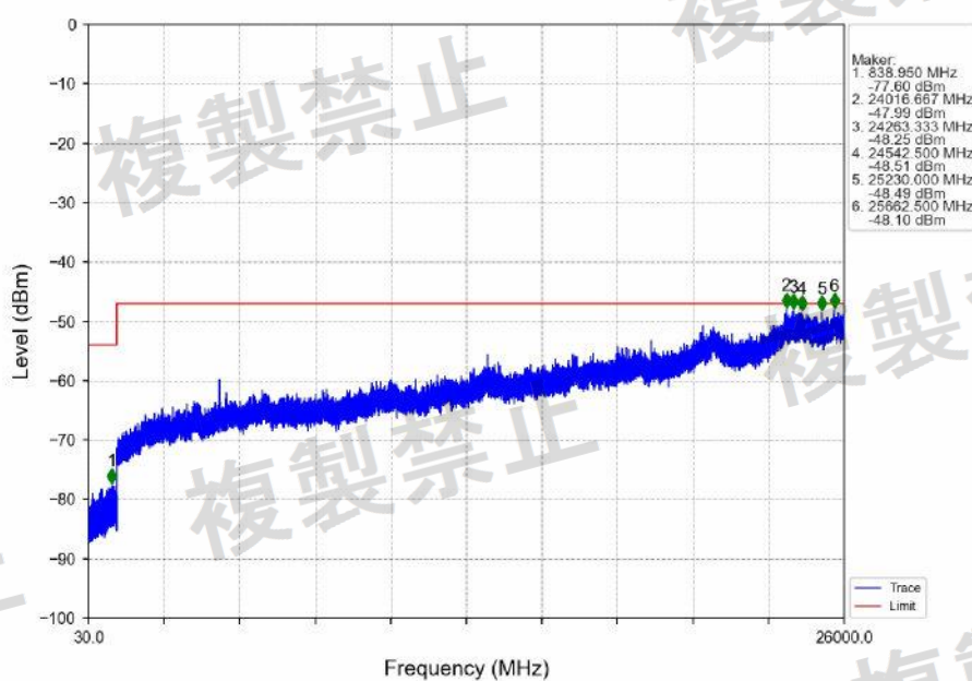
802.11n(HT20)_MCH_5200MHz_Ant1_NTNV
