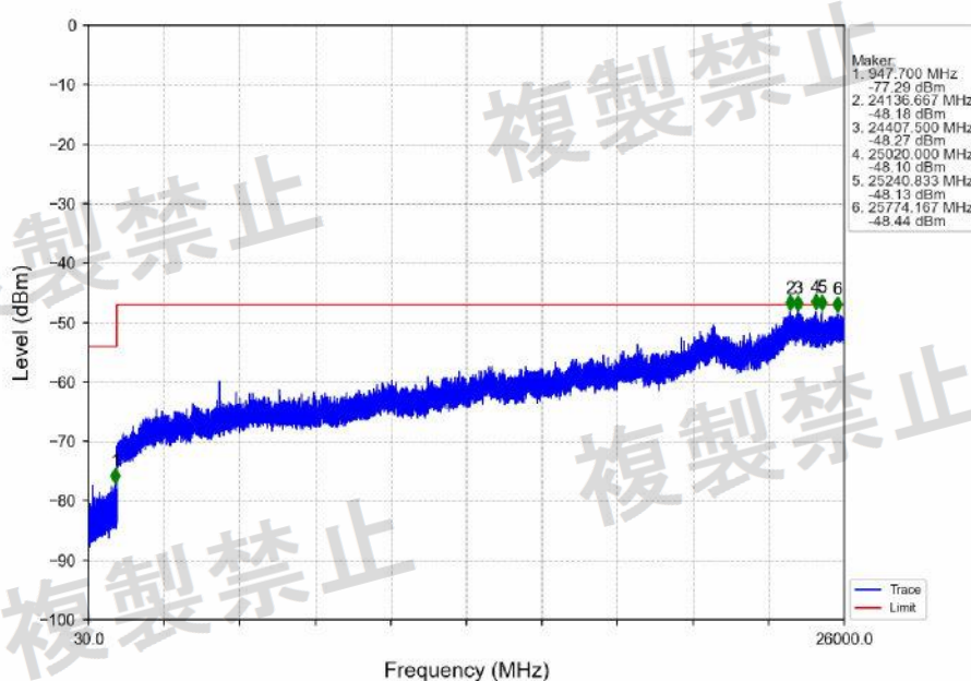
802.11ac(VHT40)_MCH_5590MHz_Ant1_NTNV
