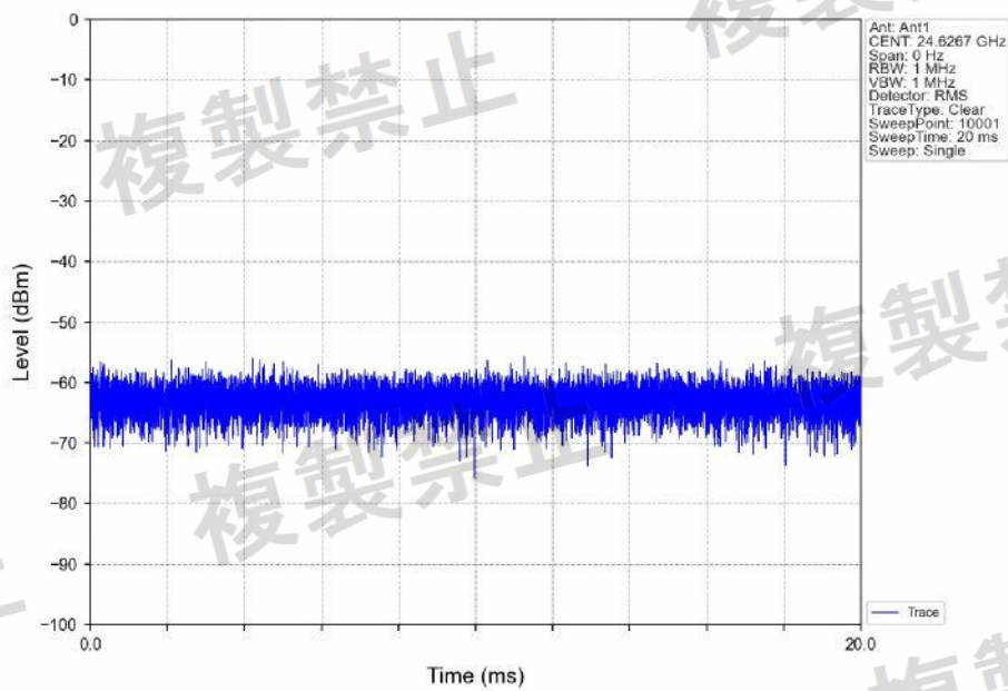
802.11ax(HEW20)_MCH_5200MHz_SU_ / _Ant1_NTNV
