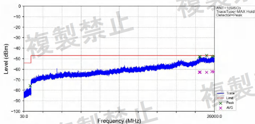
802.11a_MCH_5600MHz_Ant1_NTNV
