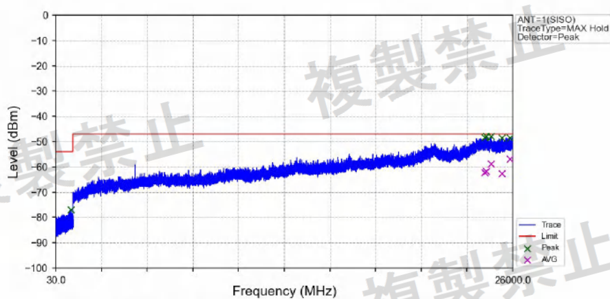
802.11ac(VHT20)_MCH_5600MHz_Ant1_NTNV
