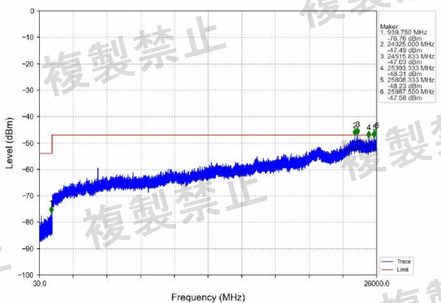
802.11ac(VHT20)_HCH_5320MHz_Ant1_NTNV
