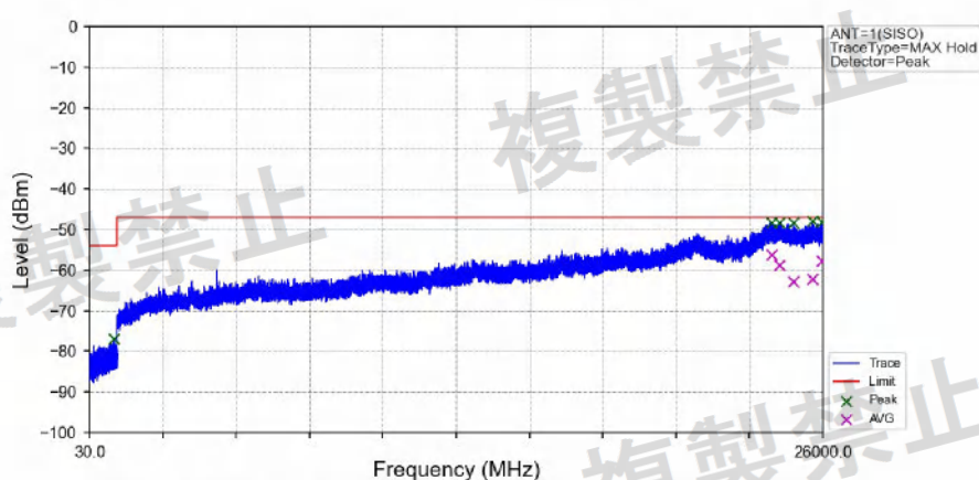
802.11ax(HEW40)_LCH_5510MHz_SU_ / _Ant1_NTNV
