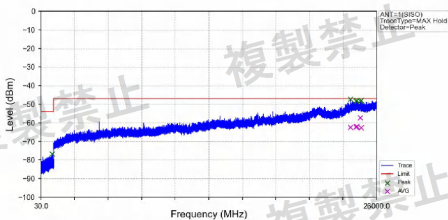
802.11ax(HEW20)_MCH_5600MHz_SU_/_Ant1_NTNV
