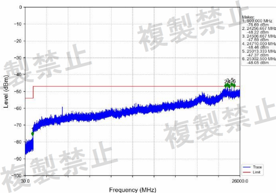
802.11ax(HEW40)_HCH_5230MHz_SU_/_Ant1_NTNV
