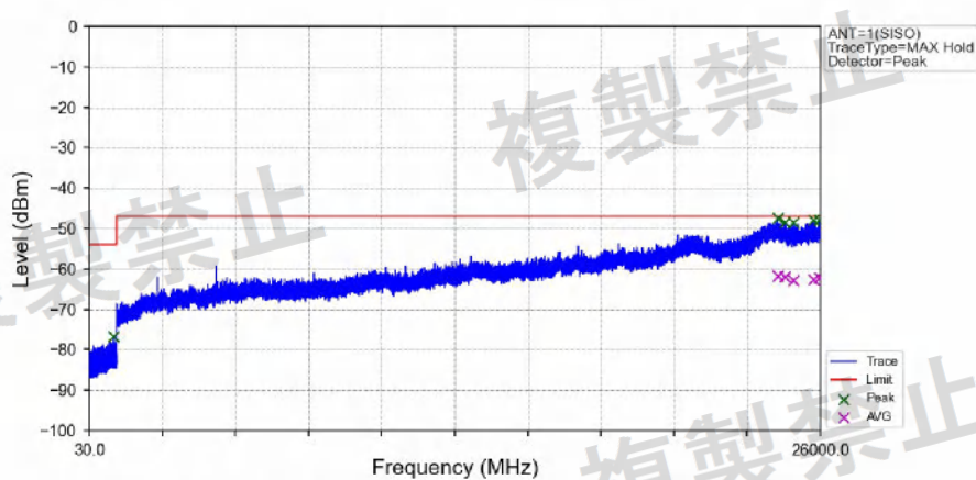
802.11ac(VHT40)_HCH_5670MHz_Ant1_NTNV
