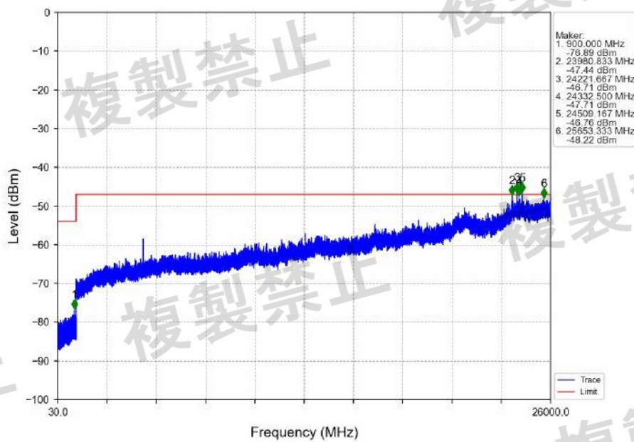
802.11ax(HEW20)_LCH_5260MHz_SU_/_Ant1_NTNV
