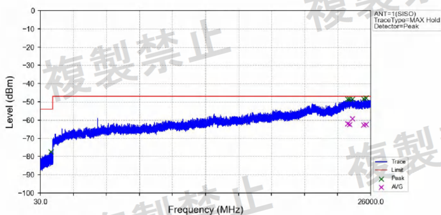
802.11a_HCH_5320MHz_Ant1_NTNV
