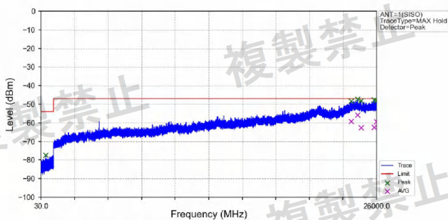
802.11ax(HEW20)_HCH_5320MHz_SU_/_Ant1_NTNV
