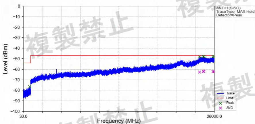
802.11ac(VHT20)_LCH_5180MHz_Ant1_NTNV
