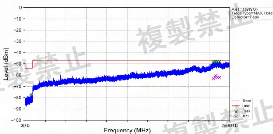
802.11ac(VHT20)_MCH_5200MHz_Ant1_NTNV
