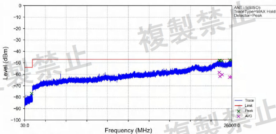
802.11a_HCH_5700MHz_Ant1_NTNV
