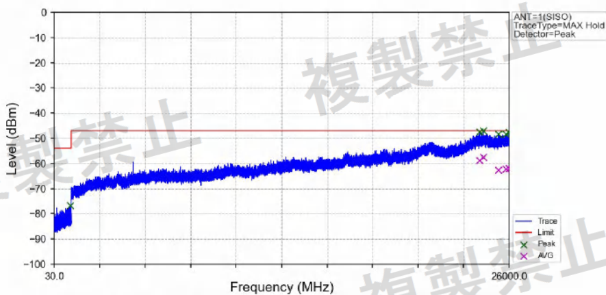
802.11ac(VHT20)_HCH_5320MHz_Ant1_NTNV
