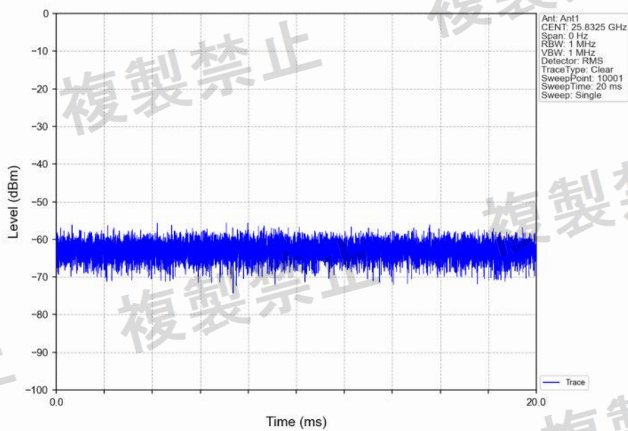
802.11ax(HEW20)_HCH_5700MHz_SU_/_Ant1_NTNV
