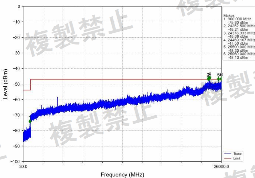
802.11n(HT20)_MCH_5600MHz_Ant1_NTNV
