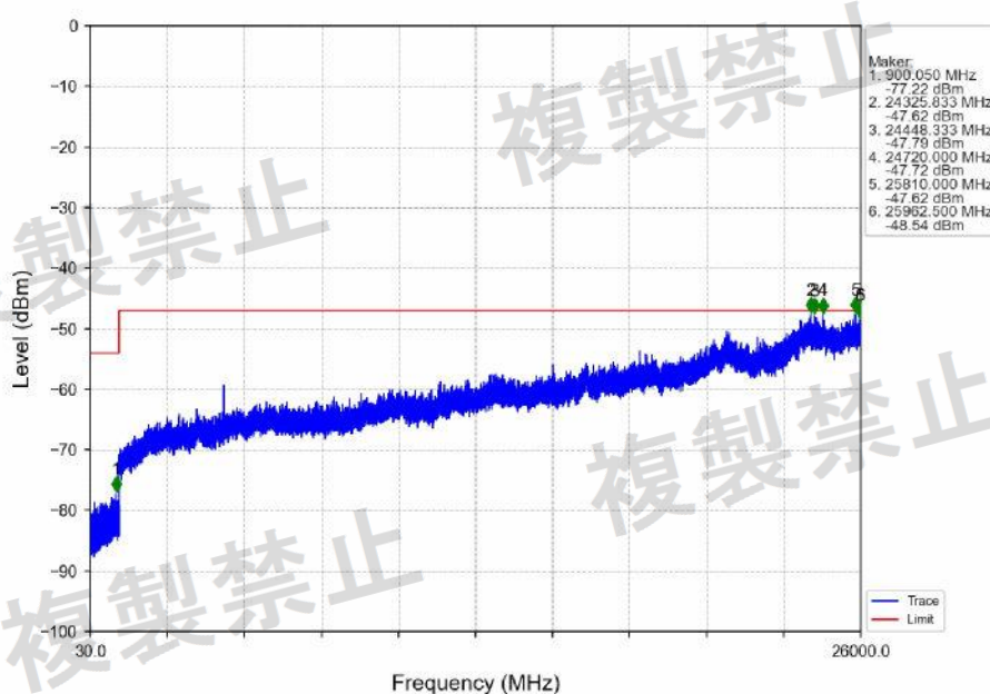
802.11ac(VHT40)_HCH_5310MHz_Ant1_NTNV
