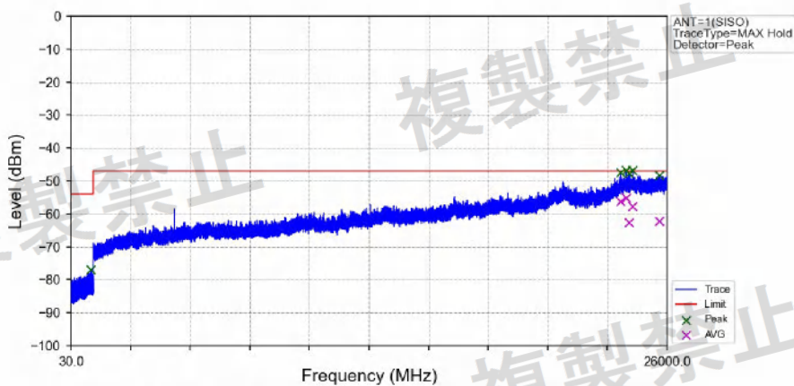
802.11ax(HEW20)_LCH_5260MHz_SU_/_Ant1_NTNV
