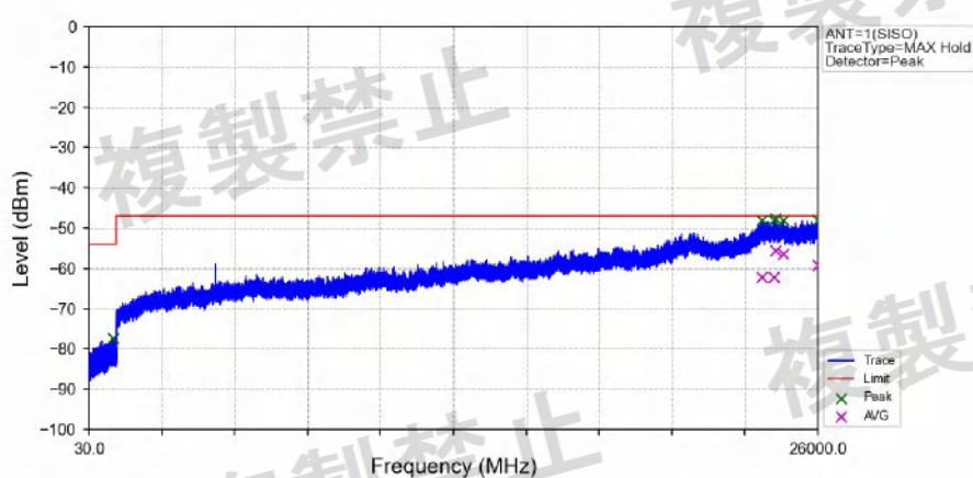
802.11ax(HEW20)_HCH_5240MHz_SU / _Ant1_NTNV
