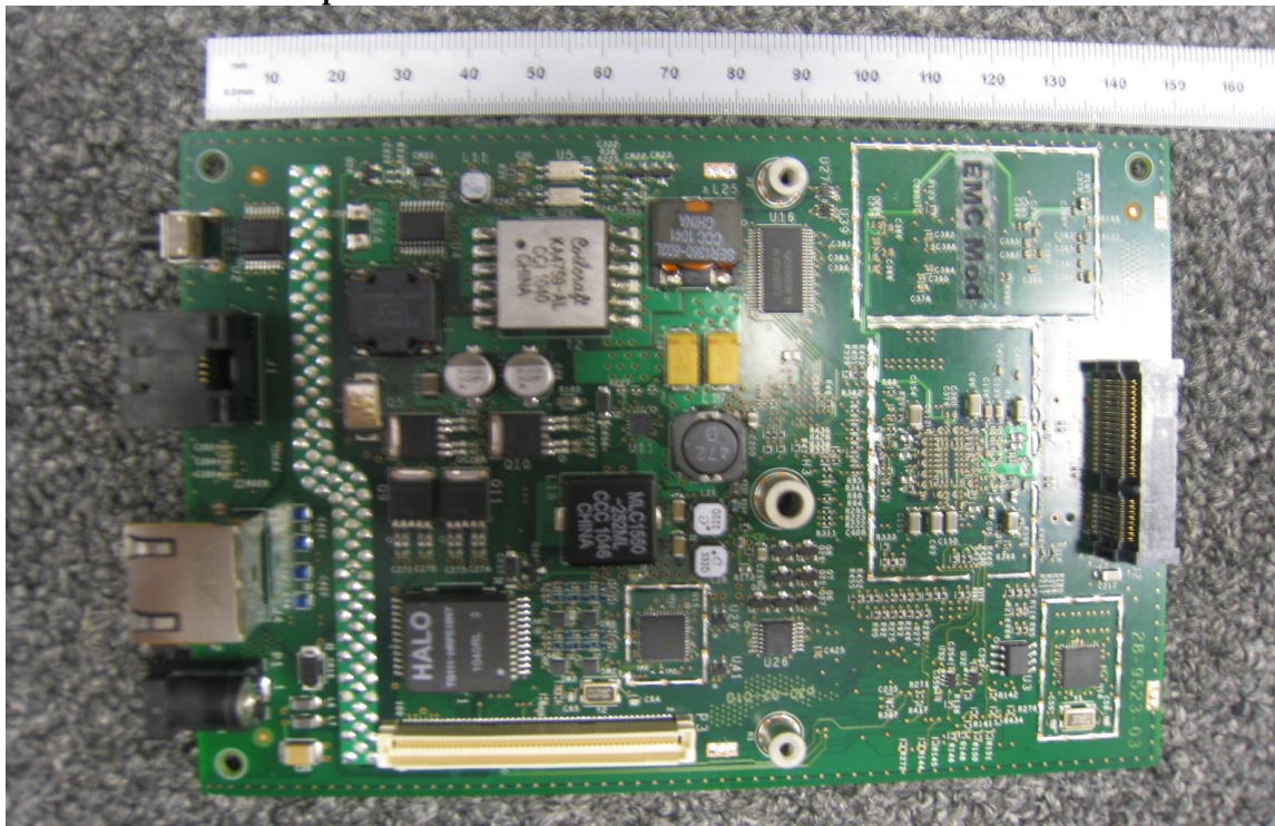
Main Control Board Top
