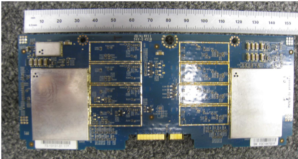
Radio Board Bottom
