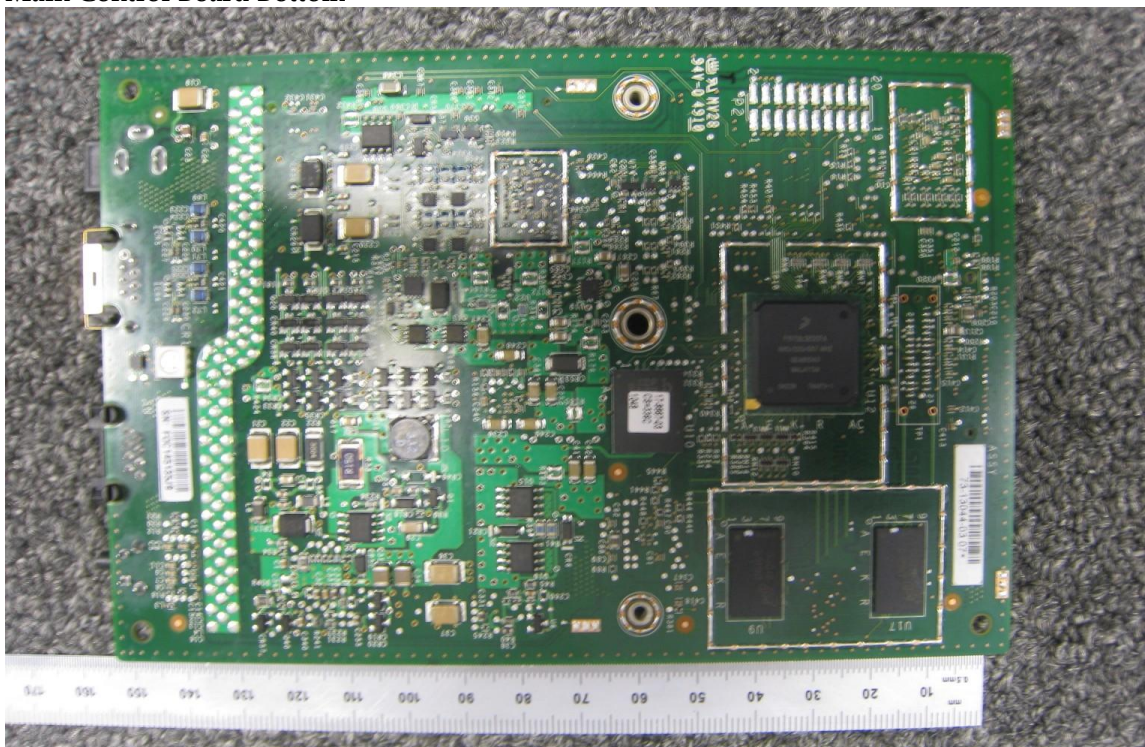
Main Control Board Bottom
