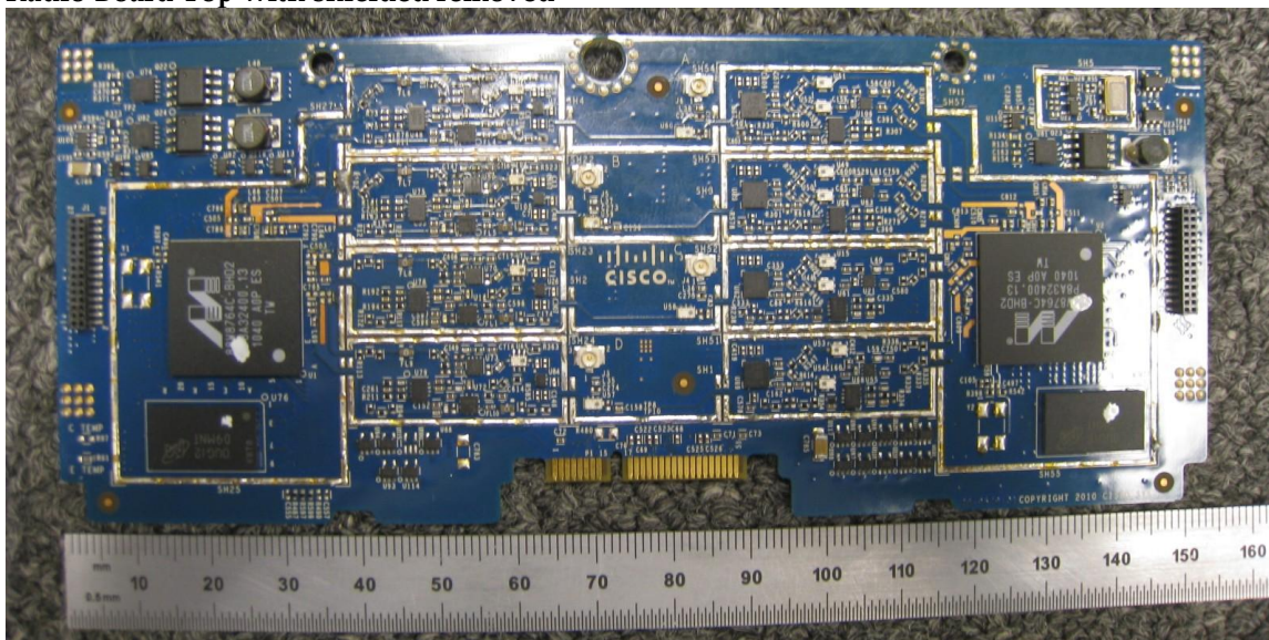
Radio Board Top with shielded removed
