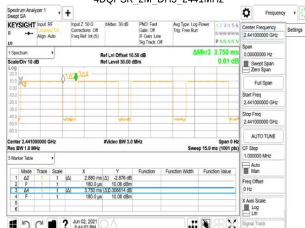
4DQPSK_2M_DH5_2441MHz
