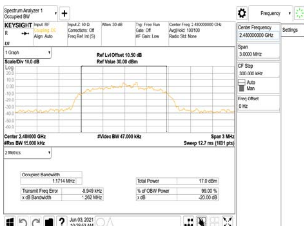
8DPSK_3M_DH5_2480MHz
