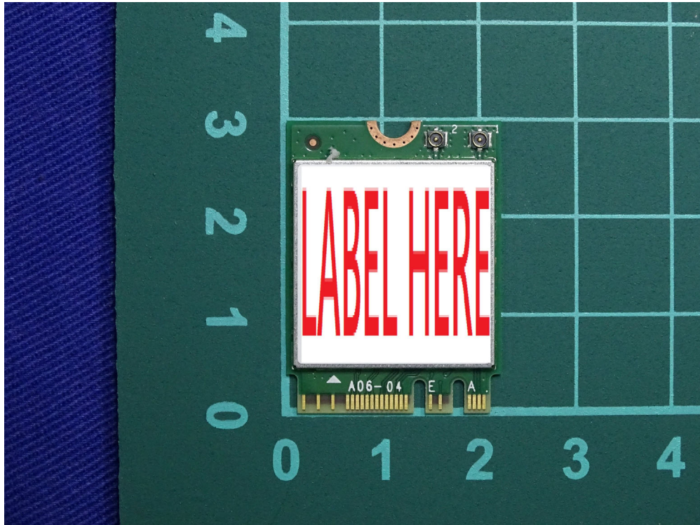
(7) EUT Photo - Trade Name: Intel, Model No.: AX210NGW
