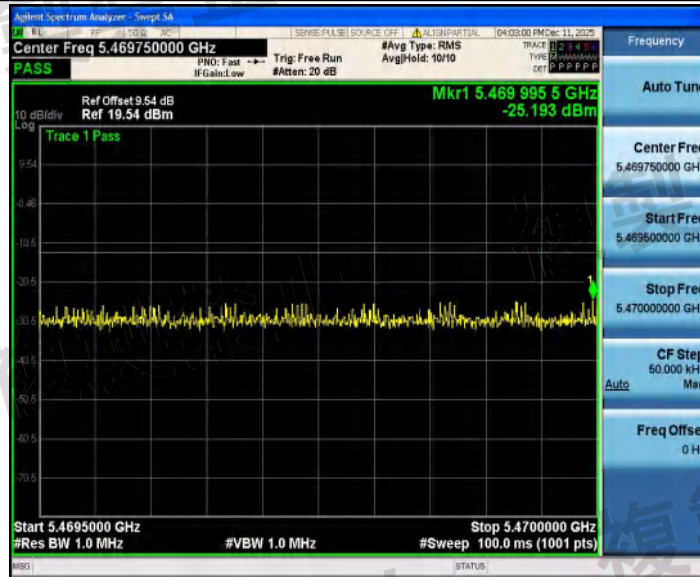
NTNV_11AX80SISO_Ant2_5530_5469.5~5470
