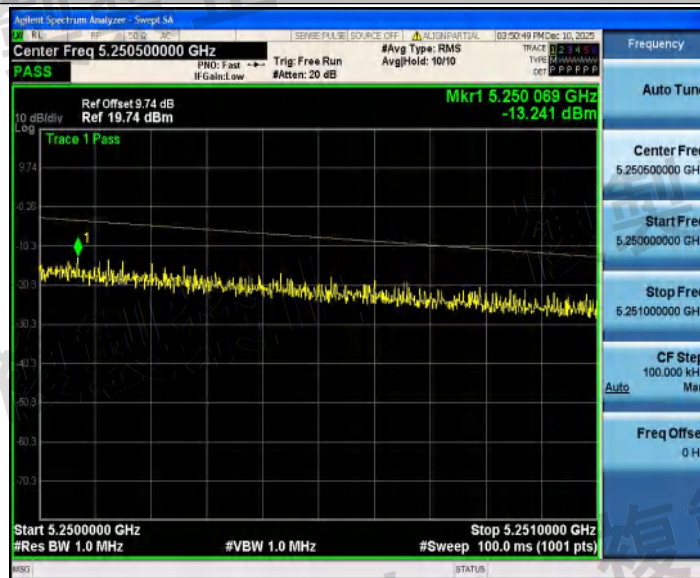
NTNV_11AX40SISO_Ant1_5230_5250~5251
