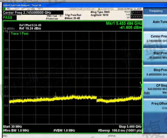
NTN_11AX20SISO_Ant2_5500_30~5460
