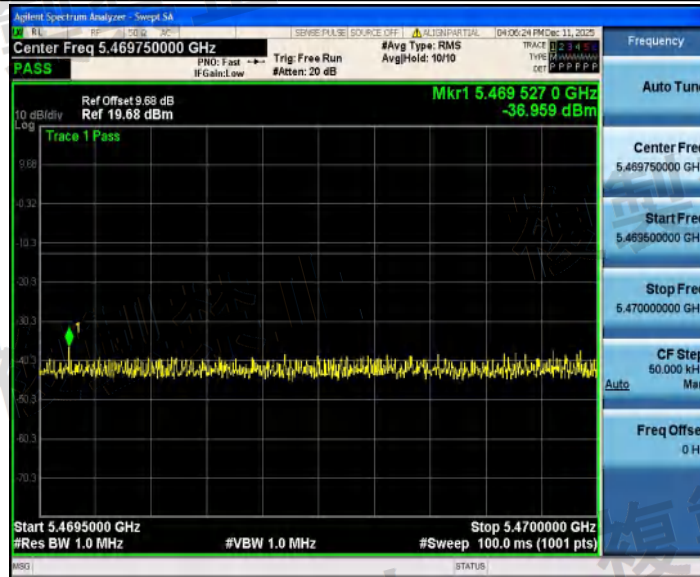
NTNV_11AX80SISO_Ant2_5610_5469.5~5470
