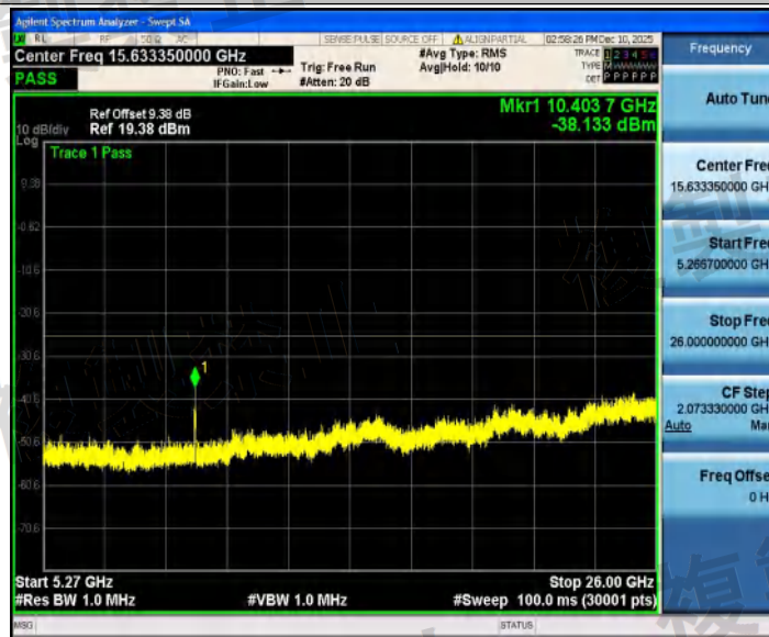
NTNV_11AX20SISO_Ant1_5200_5266.7~26000
