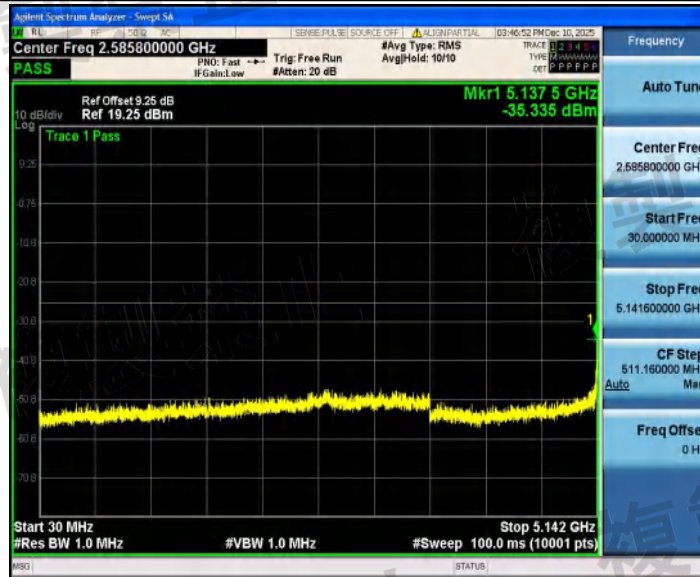
NTNV_11AX40SISO_Ant1_5190_30~5141.6
