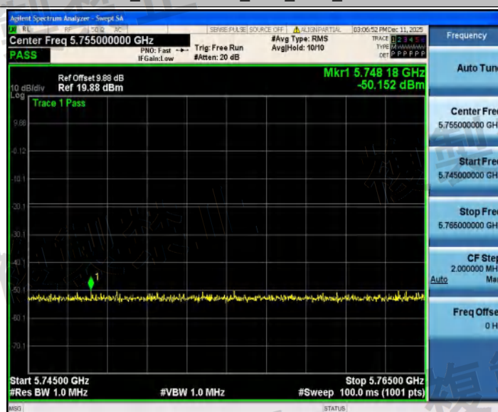
NTVN_11AX20SISO_Ant2_5600_5745~5765
