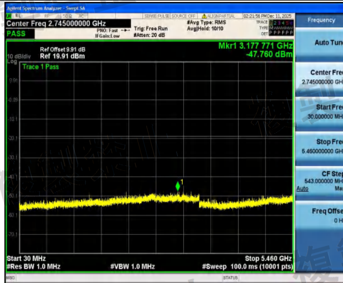
NTNV_11AC80SISO_Ant2_5690_30~5460
