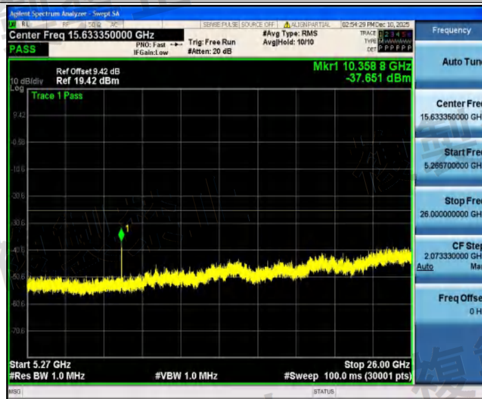
NTNV_11AX20SISO_Ant1_5180_5266.7~26000
