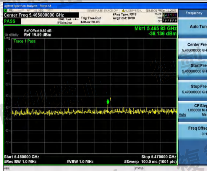
NTVN_11AX40SISO_Ant2_5550_5460~5470
