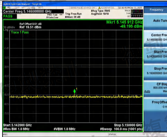
NTNV_11AX20SISO_Ant2_5240_5142~5150
