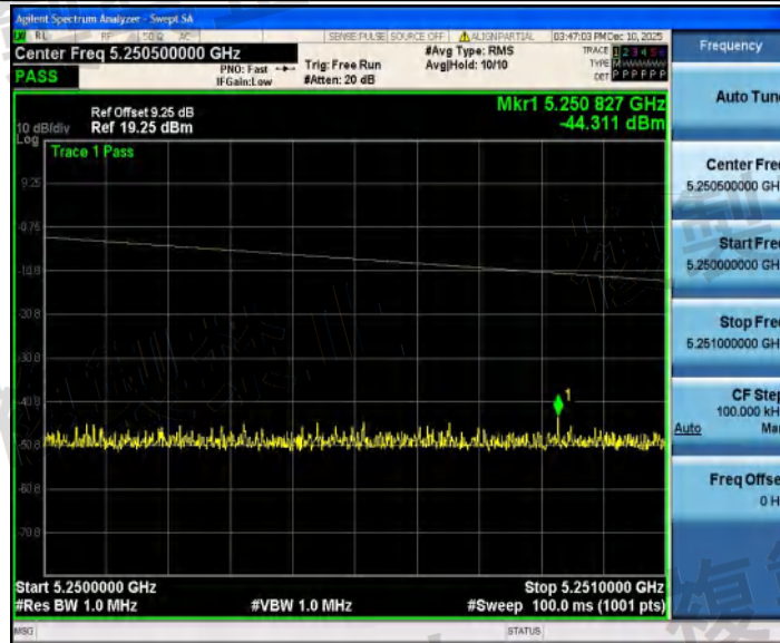
NTNV_11AX40SISO_Ant1_5190_5250~5251
