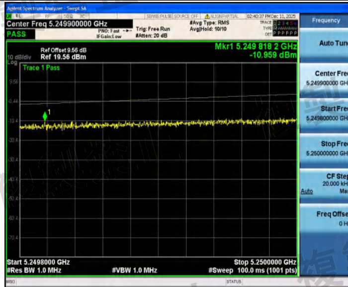
NTNV_11AX20SISO_Ant2_5260_5249.8~5250
