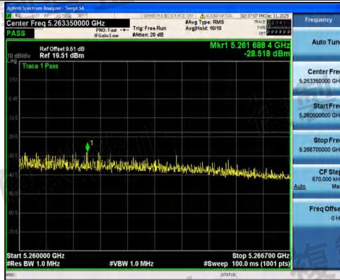
NTNV_11AX20SISO_Ant2_5240_5260~5266.7
