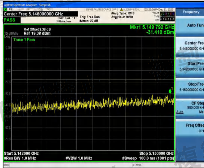
NTNV_11AX20SISO_Ant2_5180_5142~5150
