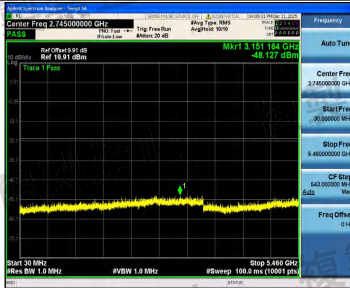
NTNV_11AX80SISO_Ant2_5690_30~5460
