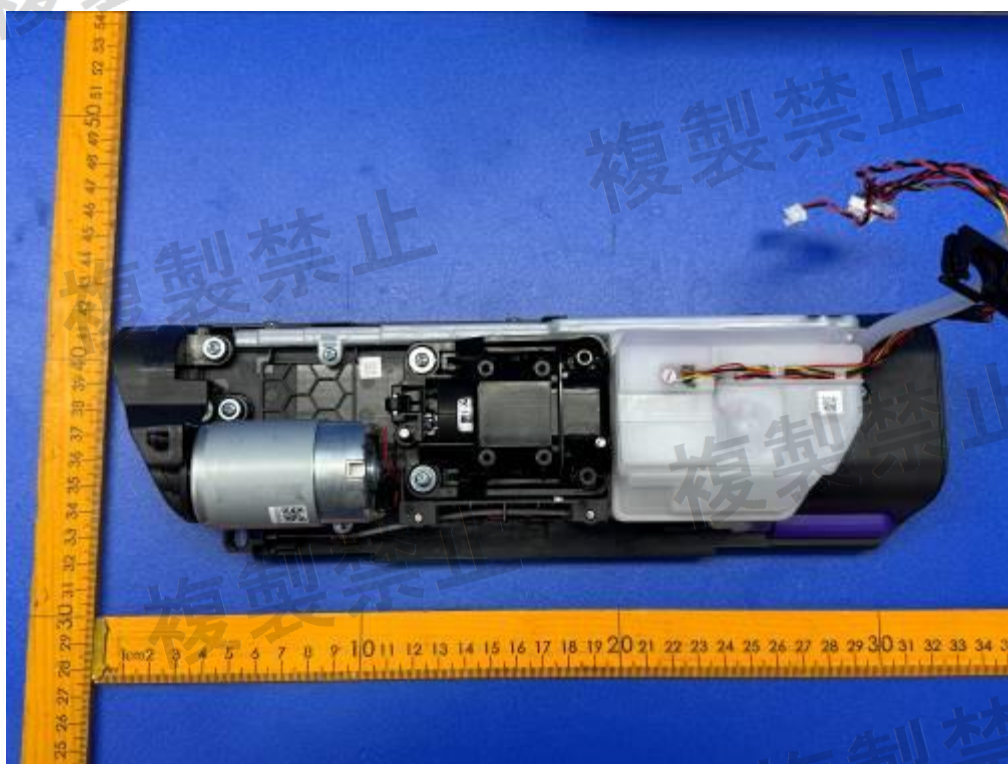
Figure 14. Mop motor module
