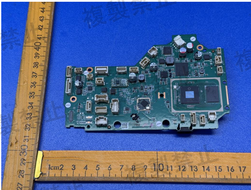
Figure 9. Main PCB
