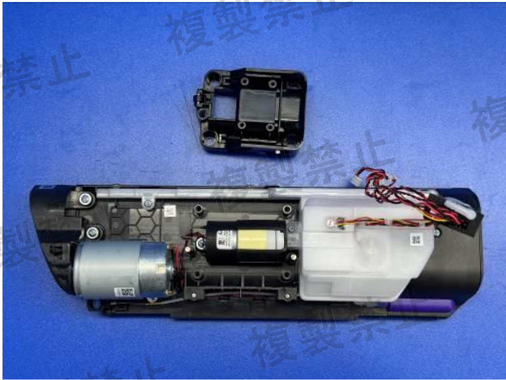
Figure 15. Mop motor module
