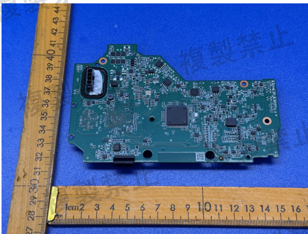
Figure 10. Main PCB
