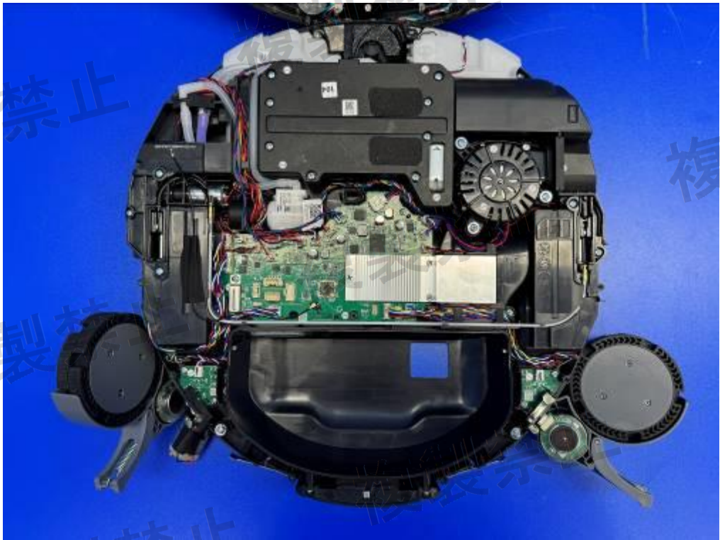
Figure 7. Internal view
