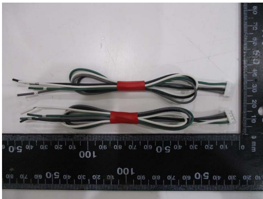
connection cable 4 pins(Wiegand input/output)
