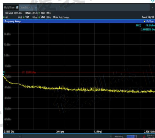
NTNV-11N40MIMO-Ant1-2462-2483.5~2496.5-PA
