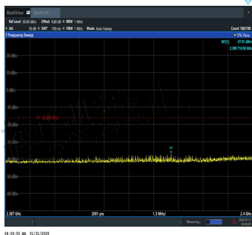
NTNV-11N40MIMO-Ant1-2462-2387~2400-PASS
