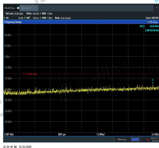
NTNV-11AX40SISO-Ant1-2462-2387~2400-PASS
