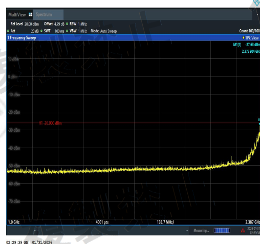
NTNV-11AX40SISO-Ant2-2462-1000~2387-See table below
