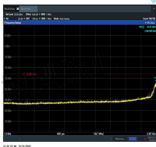
NTNV-11AX40SISO-Ant1-2462-1000~2387-PASS
