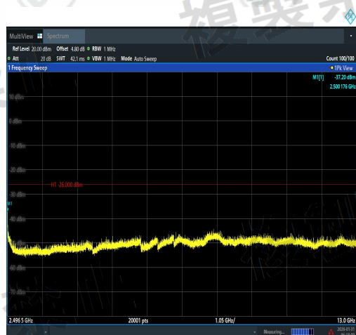
NTNV-11AX40MIMO-Ant1-2442-2483.5~2496.5-PASS
