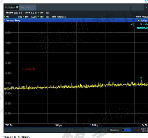
NTNV-11AX40SISO-Ant2-2462-2387~2400-PASS
