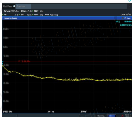
NTNV-11N40MIMO-Ant2-2462-2483.5~2496.5-PA
