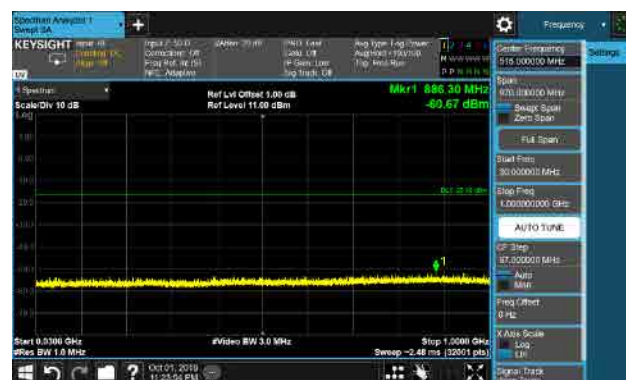
CH39 (2441MHz) 3-DH5(3Mbps)
