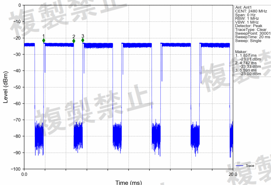
Pi/4DQPSK_2DH5_2480MHz_Ant1_NTNV
