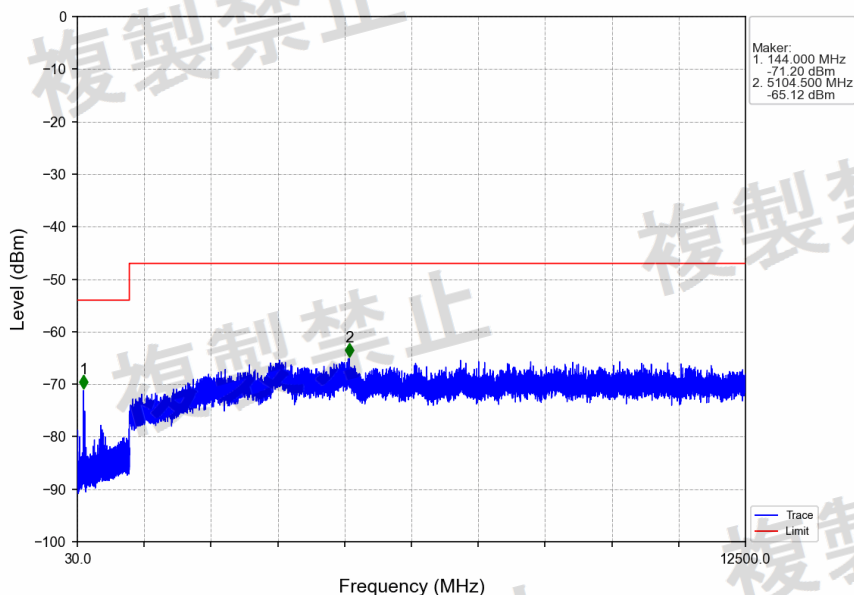
8DPSK_3DH5_2480MHz_Ant1_NTHV
