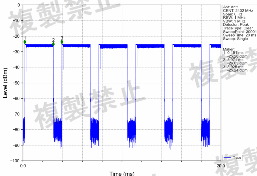
Pi/4DQPSK_2DH3_2402MHz_Ant1_NTNV
