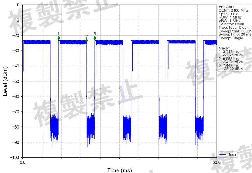
Pi/4DQPSK_2DH5_2480MHz_Ant1_NTHV
