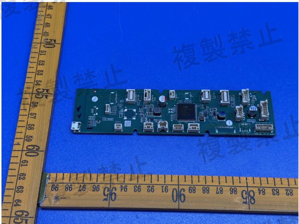
Figure 18. Control PCB view
