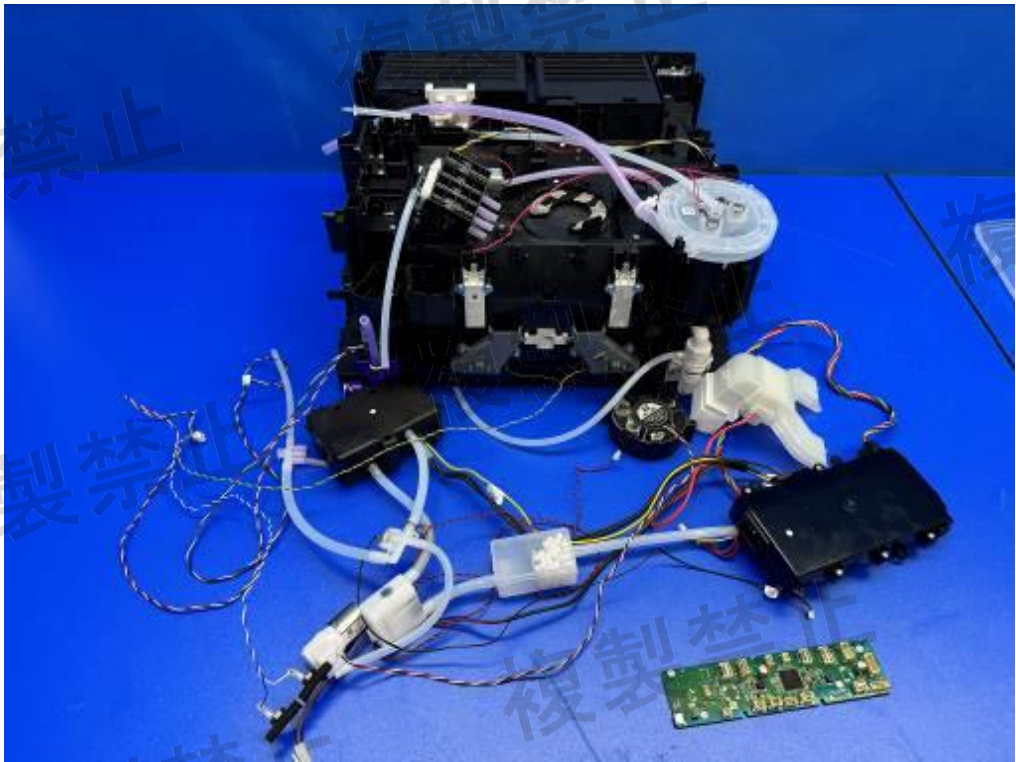
Figure 17. Internal view
