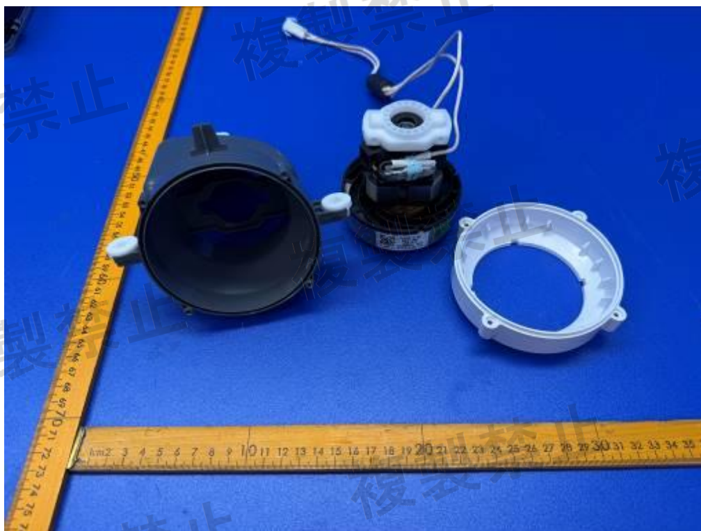
Figure 13. Series motor
