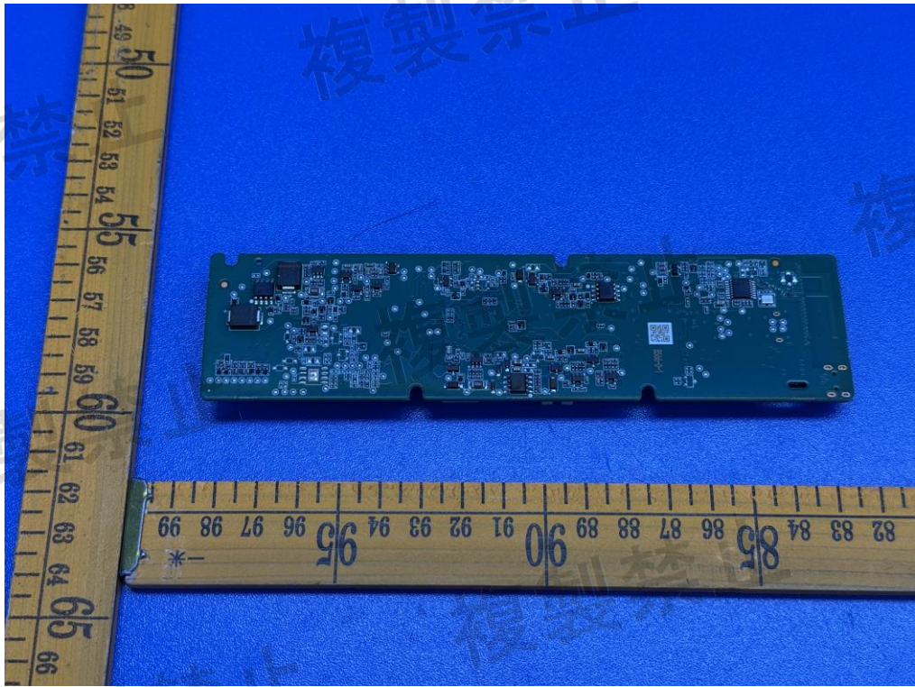
Figure 19. Control PCB view
