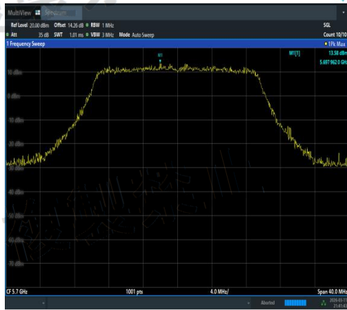
NTVN-11AX20MIMO-Ant1-5700-TPC_H-PASS
