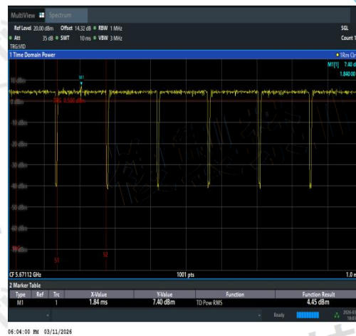
NTNV-11AX40SISO-Ant2-5670-TPC_H-PASS
