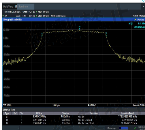
NTNV-11AC20SISO-Ant3-5500-PASS
