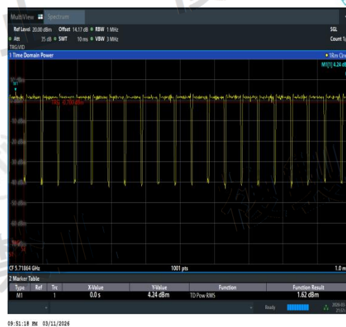
NTVN-11AX20MIMO-Ant3-5720-TPC_H-PASS
