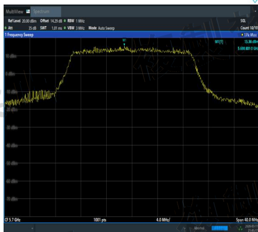
NTVN-11AX20MIMO-Ant3-5700-TPC_H-PASS
