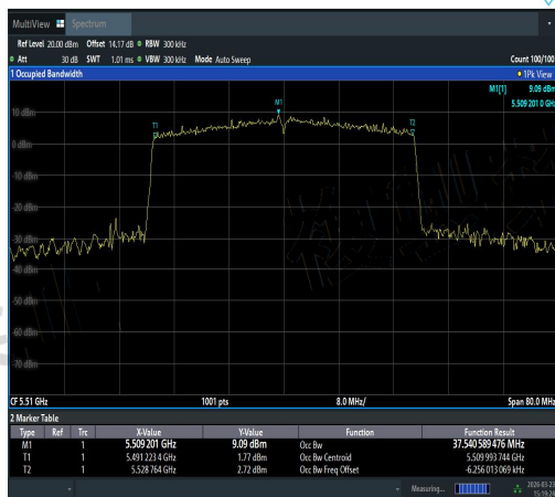
NTNV-11AX40SISO-Ant3-5510-PASS
