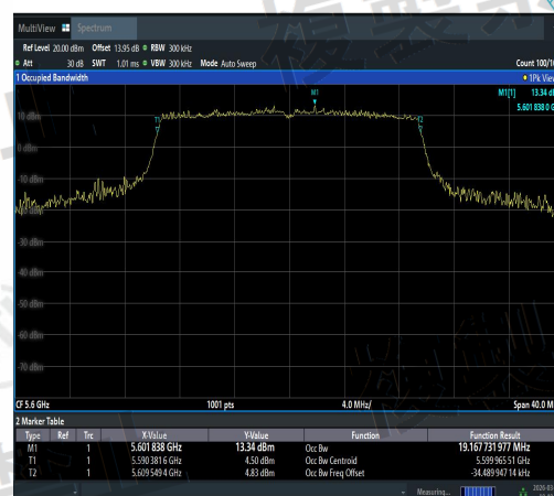
NTNV-11AX20SISO-Ant1-5600-PASS
