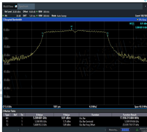
NTVN-11N20SISO-Ant2-5600-PASS
