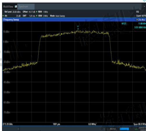
NTVN-11AX40MIMO-Ant3-5550-TPC_H-PASS
