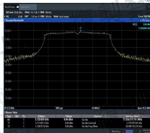
NTNV-11N20SISO-Ant3-5720-PASS
