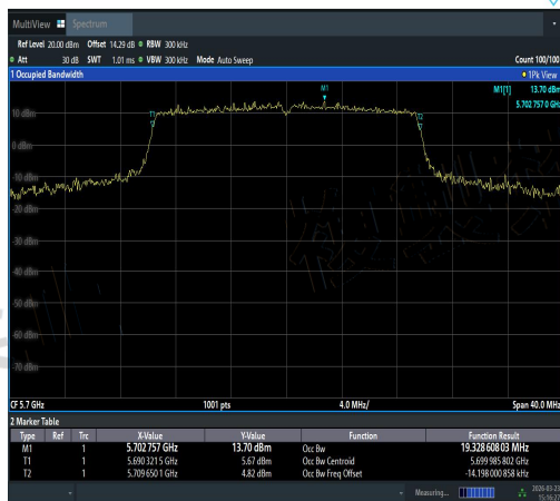
NTNV-11AX20SISO-Ant3-5700-PASS
