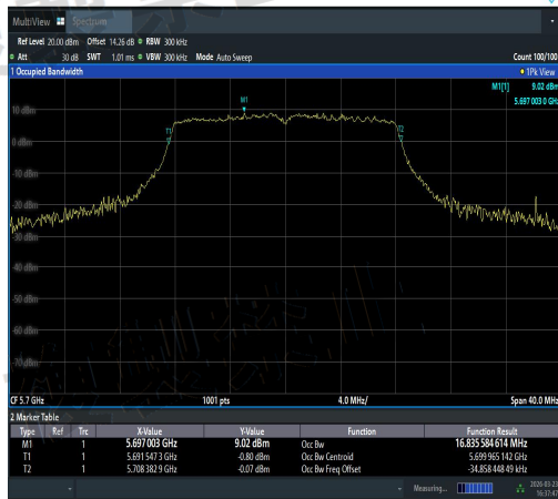
NTNV-11A-Ant1-5700-PASS
