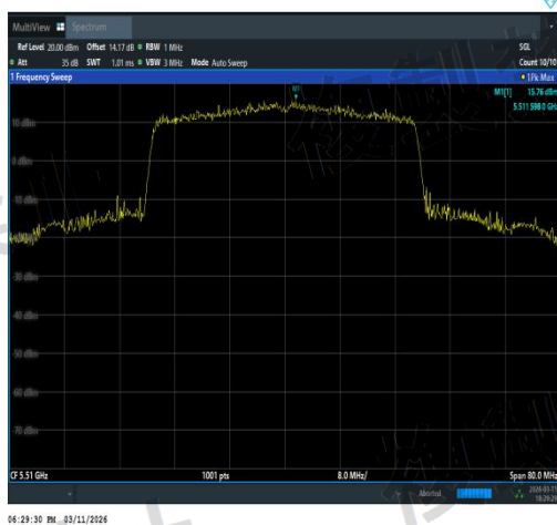
NTNV-11AX40SISO-Ant3-5510-TPC_H-PASS
