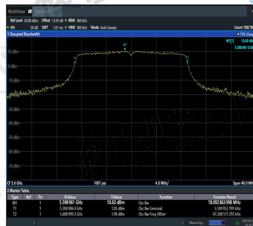
NTNV-11AC20SISO-Ant1-5600-PASS
