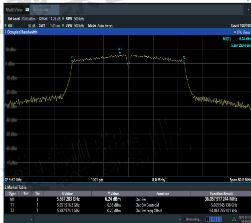
NTNV-11N40SISO-Ant1-5670-PASS
