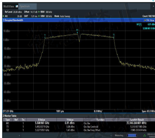
NTNV-11N40SISO-Ant3-5510-PASS
