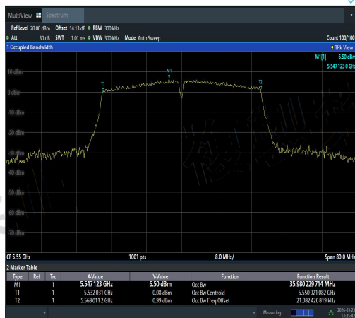
NTNV-11AC40SISO-Ant2-5550-PASS
