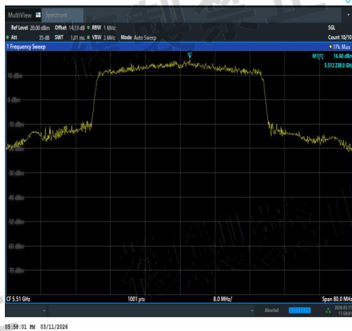
NTNV-11AX40SISO-Ant2-5510-TPC_H-PASS
