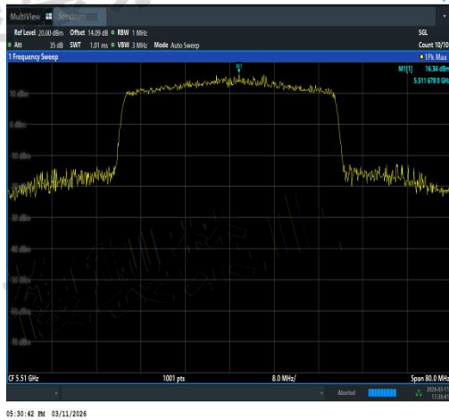
NTNV-11AX40SISO-Ant1-5510-TPC_H-PASS
