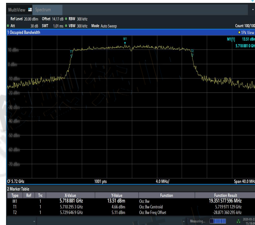
NTNV-11AX20SISO-Ant3-5720-PASS
