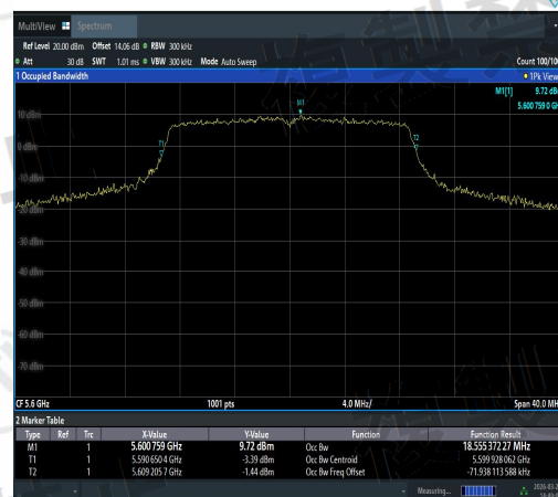
NTNV-11AC20SISO-Ant3-5600-PASS
