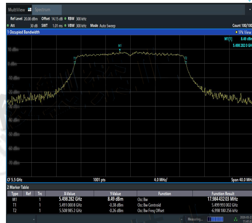
NTVN-11N20SISO-Ant2-5500-PASS
