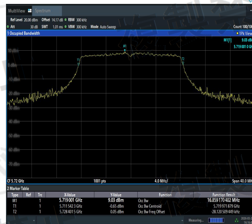
NTNV-11A-Ant3-5720-PASS
