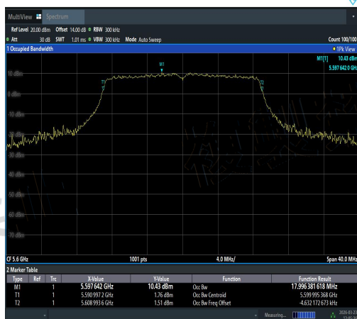
NTNV-11AC20SISO-Ant2-5600-PASS
