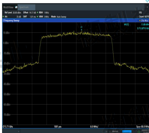
NTVN-11AX40MIMO-Ant3-5710-TPC_H-PASS
