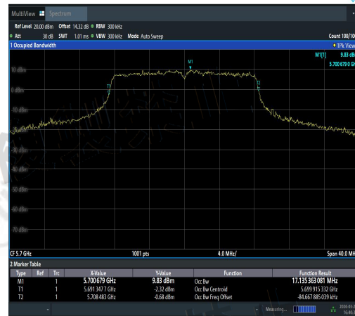
NTNV-11A-Ant2-5700-PASS
