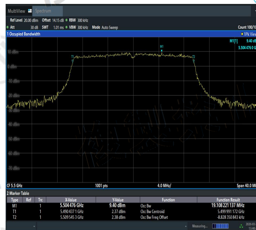
NTNV-11AX20SISO-Ant2-5500-PASS
