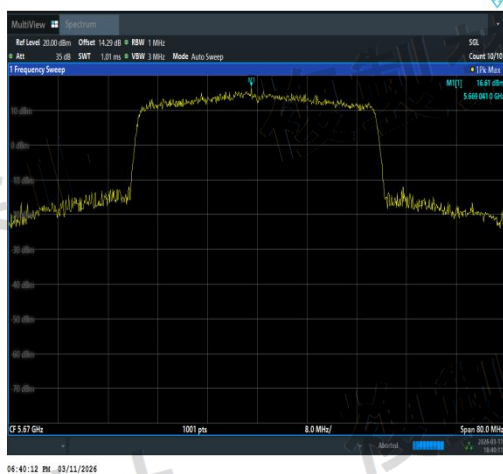
NTNV-11AX40SISO-Ant3-5670-TPC_H-PASS
