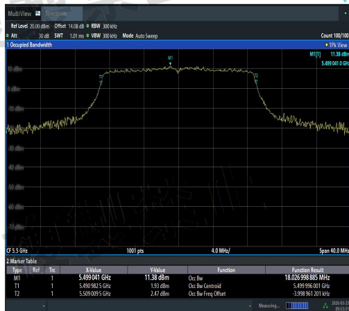
NTVN-11N20SISO-Ant1-5500-PASS
