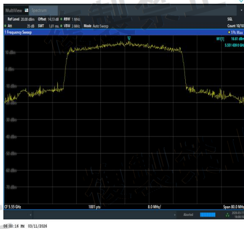
NTNV-11AX40SISO-Ant2-5550-TPC_H-PASS
