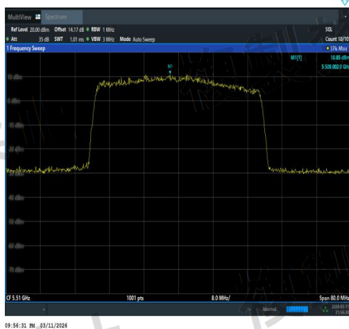
NTVN-11AX40MIMO-Ant3-5510-TPC_H-PASS
