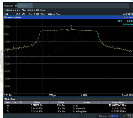
NTNV-11N20SISO-Ant2-5700-PASS
