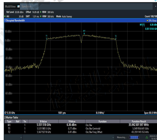
NTNV-11AC40SISO-Ant1-5550-PASS
