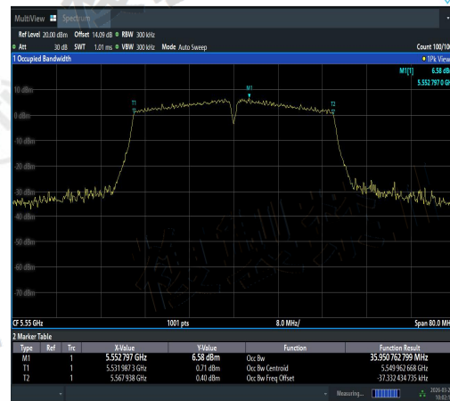
NTNV-11N40SISO-Ant1-5550-PASS
