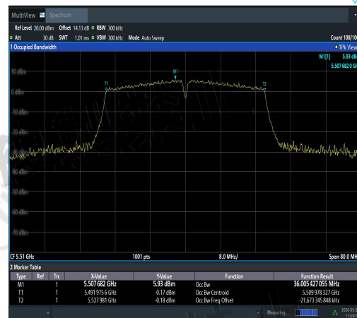
NTNV-11N40SISO-Ant2-5510-PASS
