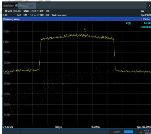
NTVN-11AX80MIMO-Ant1-5690-TPC_H-PASS
