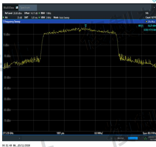
NTNV-11AX40SISO-Ant3-5550-TPC_H-PASS
