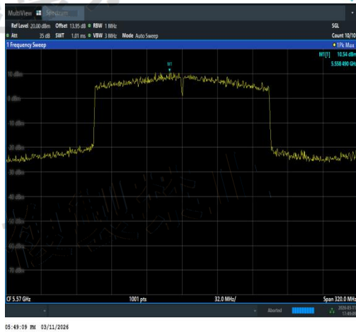
NTVN-11AX160SISO-Ant1-5570-TPC_H-PASS
