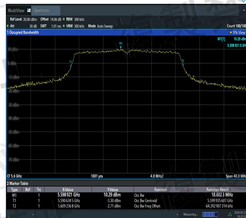
NTVN-11N20SISO-Ant3-5600-PASS
