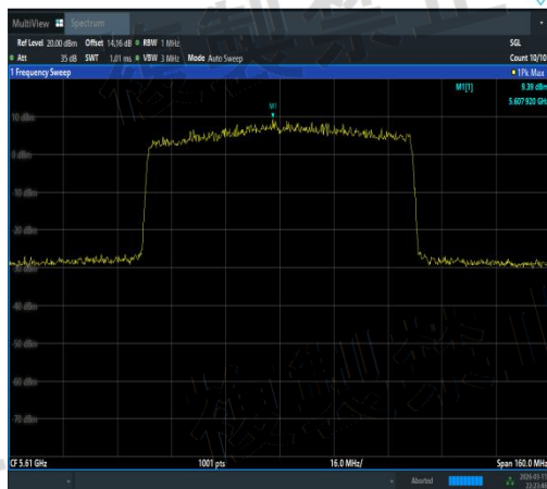
NTNV-11AX80MIMO-Ant2-5610-TPC_H-PASS
