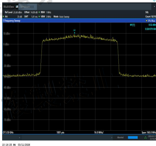
NTVN-11AX80MIMO-Ant1-5530-TPC_H-PASS
