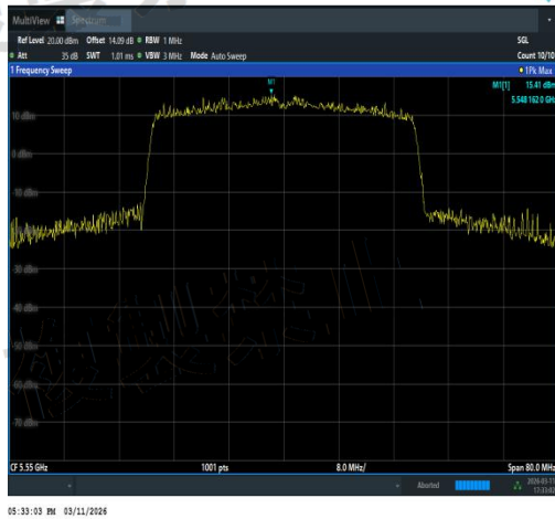
NTNV-11AX40SISO-Ant1-5550-TPC_H-PASS
