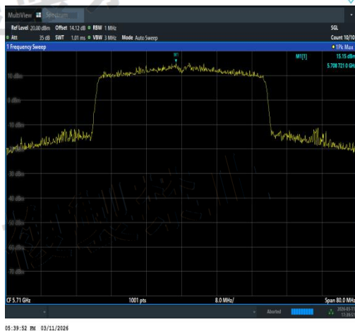
NTNV-11AX40SISO-Ant1-5710-TPC_H-PASS
