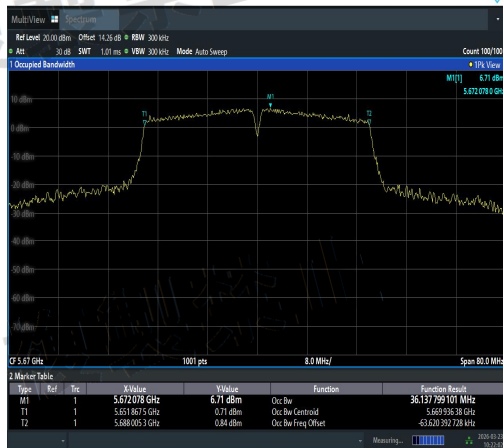
NTNV-11AC40SISO-Ant1-5670-PASS
