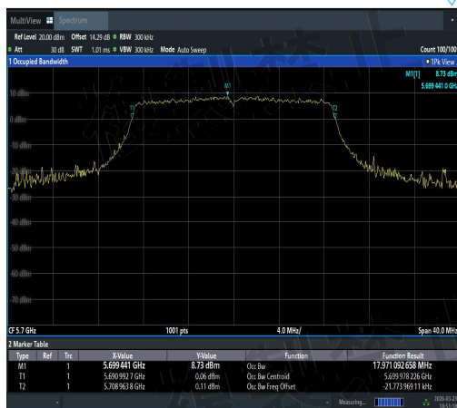
NTNV-11AC20SISO-Ant3-5700-PASS
