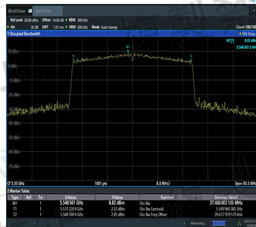
NTNV-11AX40SISO-Ant1-5550-PASS
