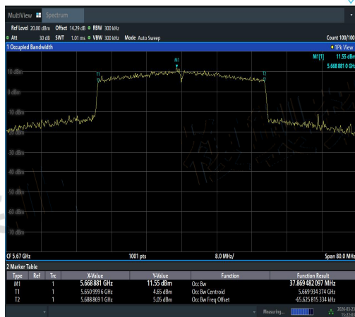
NTNV-11AX40SISO-Ant3-5670-PASS
