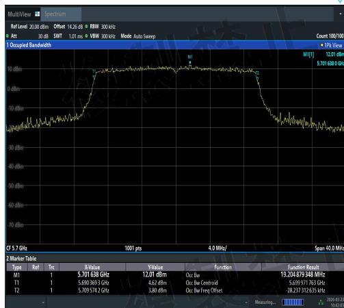
NTNV-11AX20SISO-Ant1-5700-PASS
