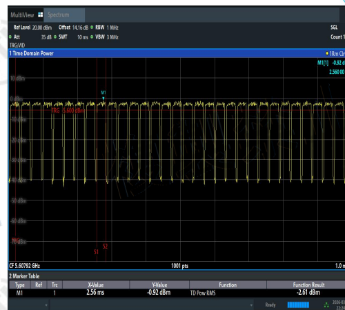
NTNV-11AX80MIMO-Ant2-5610-TPC_H-PASS
