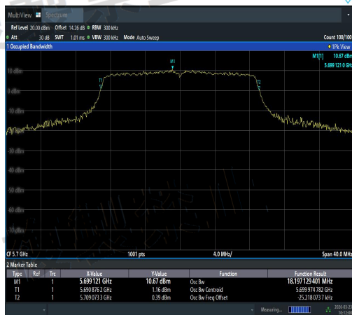
NTNV-11AC20SISO-Ant1-5700-PASS
