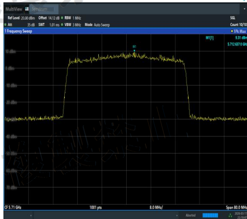
NTVN-11AX40MIMO-Ant1-5710-TPC_H-PASS
