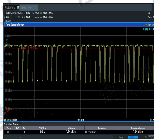
NTNV-11AX80MIMO-Ant3-5610-TPC_H-PASS
