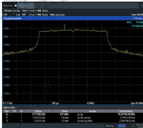
NTNV-11AX20SISO-Ant2-5720-PASS
