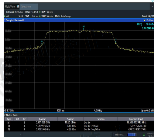
NTNV-11AC20SISO-Ant2-5700-PASS
