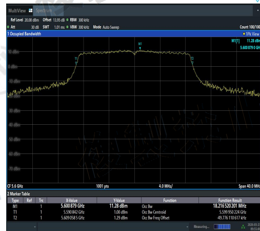
NTVN-11N20SISO-Ant1-5600-PASS
