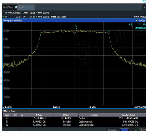
NTNV-11AX20SISO-Ant3-5500-PASS
