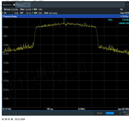
NTNV-11AX40SISO-Ant1-5670-TPC_H-PASS
