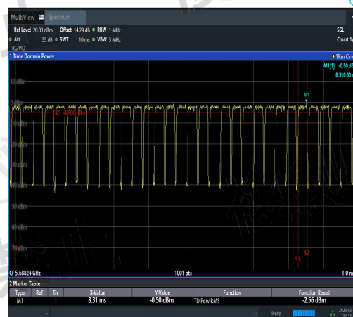
NTVN-11AX80MIMO-Ant3-5690-TPC_H-PASS
