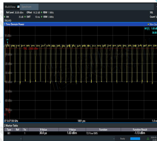
NTNV-11AX40MIMO-Ant2-5670-TPC_H-PASS
