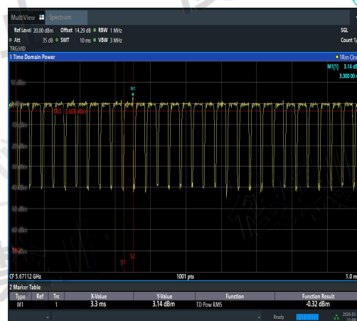
NTNV-11AX40MIMO-Ant3-5670-TPC_H-PASS
