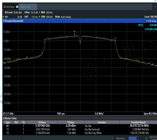
NTNV-11N40SISO-Ant2-5710-PASS
