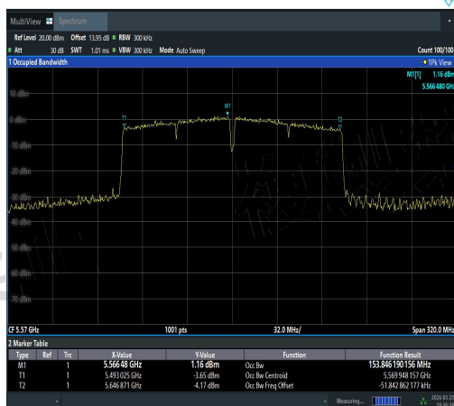
NTNV-11AC160SISO-Ant1-5570-PASS
