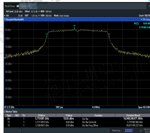
NTNV-11A-Ant1-5720-PASS
