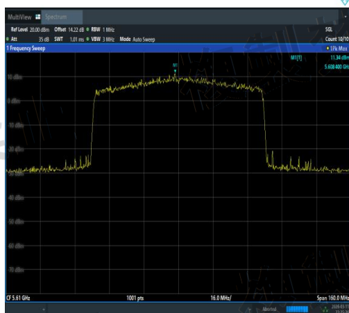
NTNV-11AX80MIMO-Ant3-5610-TPC_H-PASS
