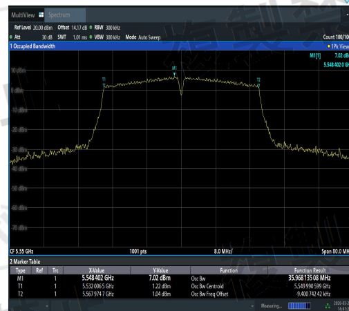
NTNV-11N40SISO-Ant3-5550-PASS
