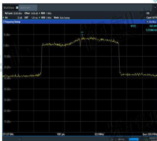
NTVN-11AX160MIMO-Ant3-5570-TPC_H-PASS
