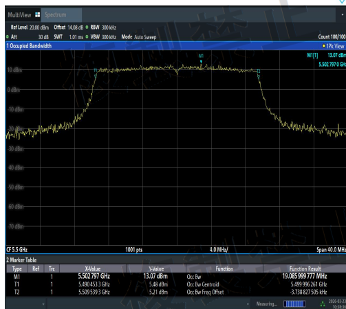
NTNV-11AX20SISO-Ant1-5500-PASS
