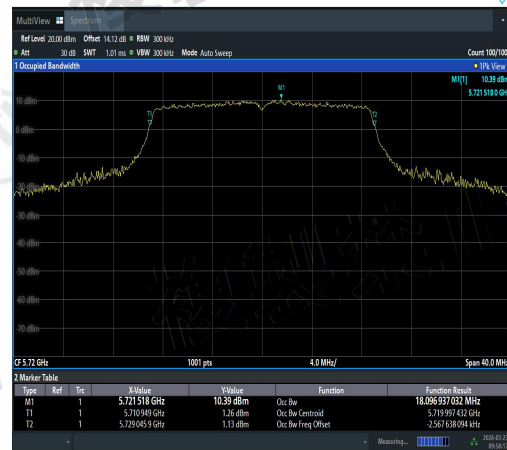
NTNV-11N20SISO-Ant1-5720-PASS
