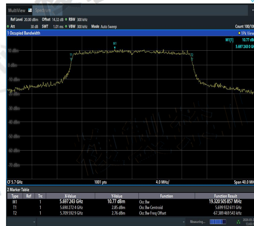
NTNV-11AX20SISO-Ant2-5700-PASS
