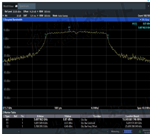
NTNV-11A-Ant3-5700-PASS
