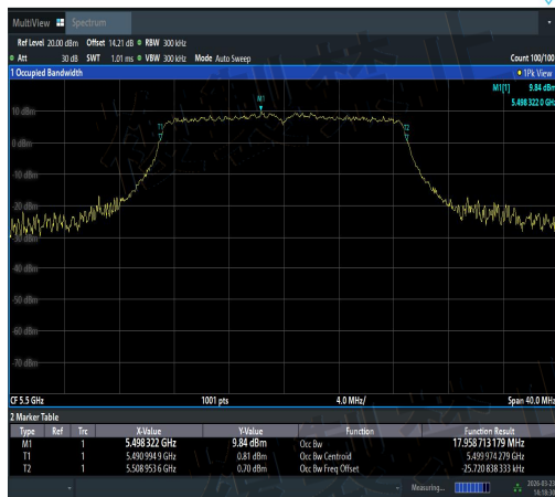
NTVN-11N20SISO-Ant3-5500-PASS
