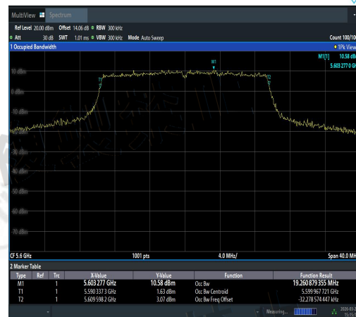
NTNV-11AX20SISO-Ant3-5600-PASS
