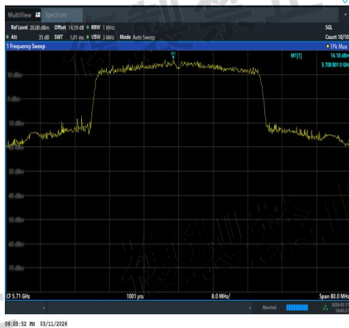
NTNV-11AX40SISO-Ant2-5710-TPC_H-PASS
