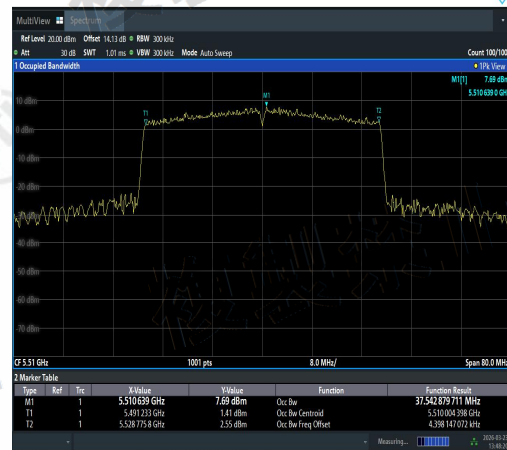
NTNV-11AX40SISO-Ant2-5510-PASS
