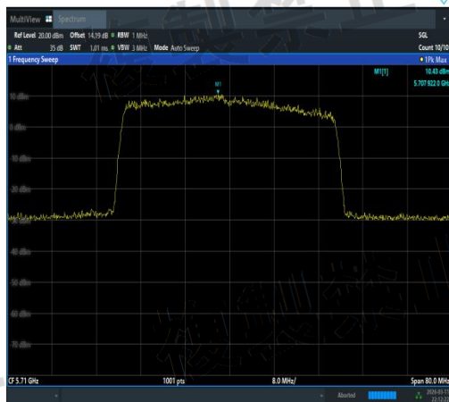
NTVN-11AX40MIMO-Ant2-5710-TPC_H-PASS
