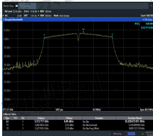
NTNV-11AC40SISO-Ant1-5510-PASS
