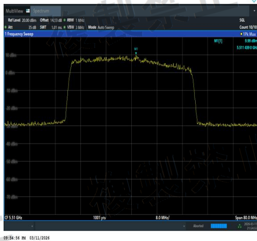
NTVN-11AX40MIMO-Ant2-5510-TPC_H-PASS
