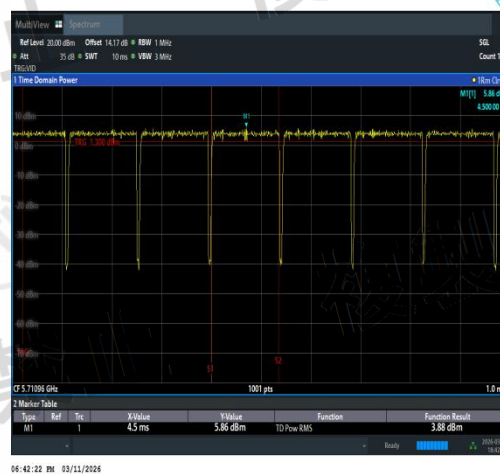
NTNV-11AX40SISO-Ant3-5710-TPC_H-PASS
