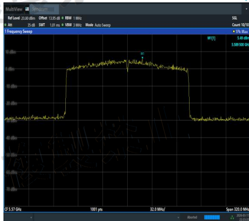
NTVN-11AX160MIMO-Ant1-5570-TPC_H-PASS
