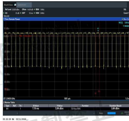
NTNV-11AX40SISO-Ant1-5550-TPC_H-PASS
