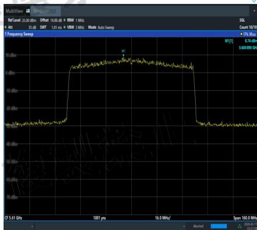
NTNV-11AX80MIMO-Ant1-5610-TPC_H-PASS
