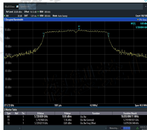
NTNV-11AC20SISO-Ant1-5720-PASS
