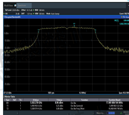
NTNV-11AC20SISO-Ant2-5500-PASS
