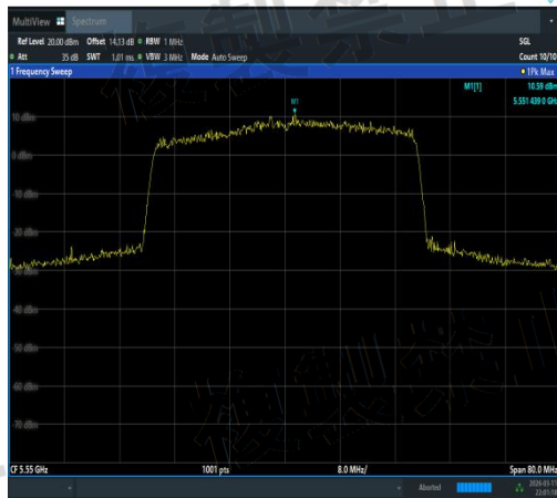
NTVN-11AX40MIMO-Ant2-5550-TPC_H-PASS
