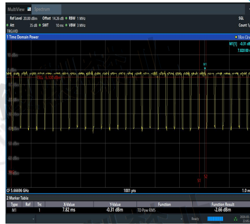
NTNV-11AX40MIMO-Ant1-5670-TPC_H-PASS
