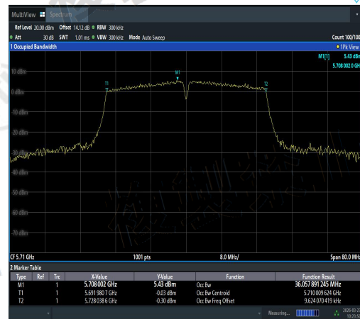
NTNV-11AC40SISO-Ant1-5710-PASS
