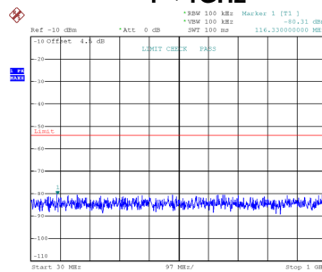
CH43 f < 1GHz
