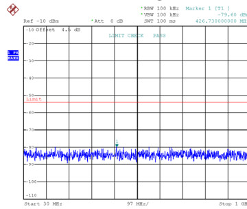
CH39 f < 1GHz
