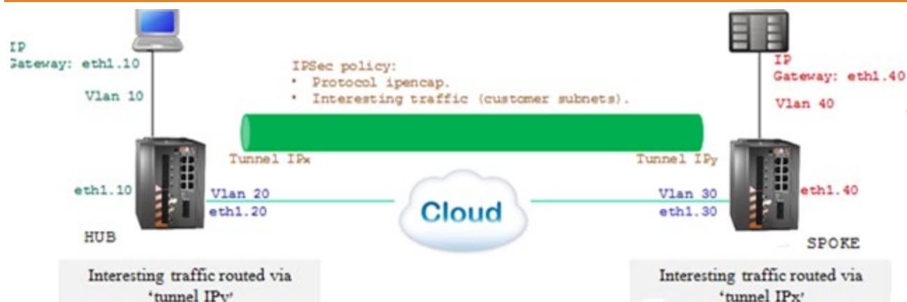
Figure 34 - Route Based IPsec-VPN
