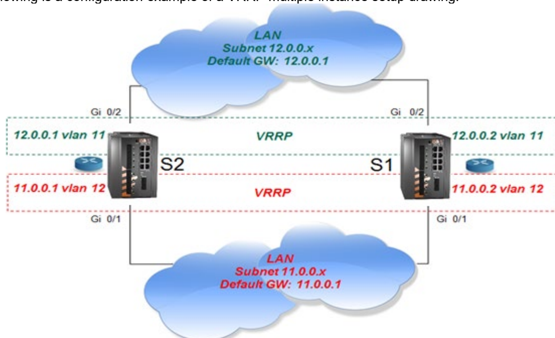
Figure 7 - Configuration Example of VRRP Multiple Instance Setup
