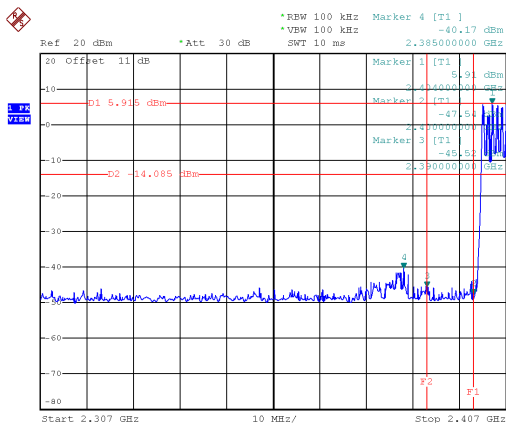
Hopping on mode (Lower)
