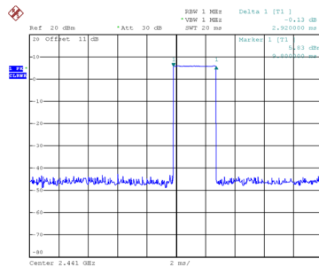
CH39-DH5
