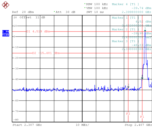
Bandedge CH00 (Lower)
