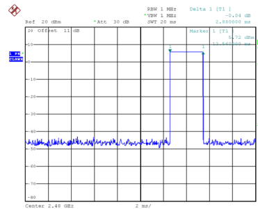
CH78-DH5
