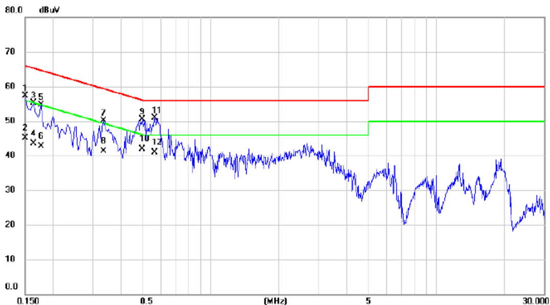
Phase: Line
