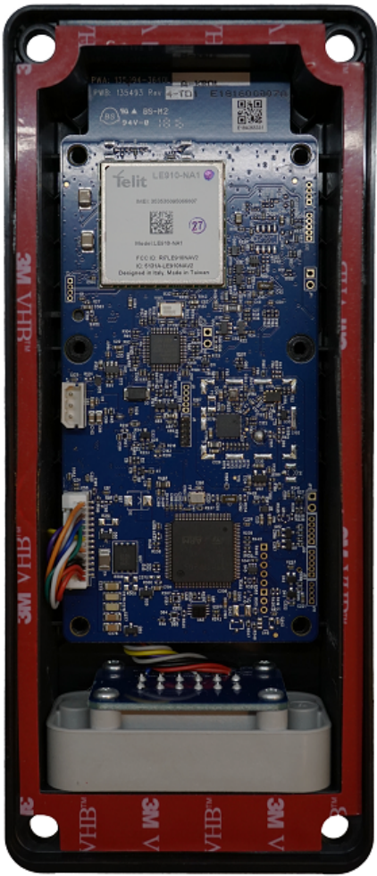
HMU-3640™ LTE PCBA Bottom
