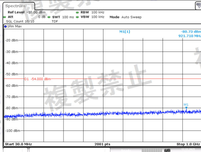
NTNV_BLE_1M_Ant1_2480_30~1000
