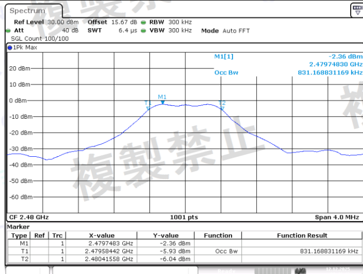
NTNV_BLE_1M_Ant1_2480
