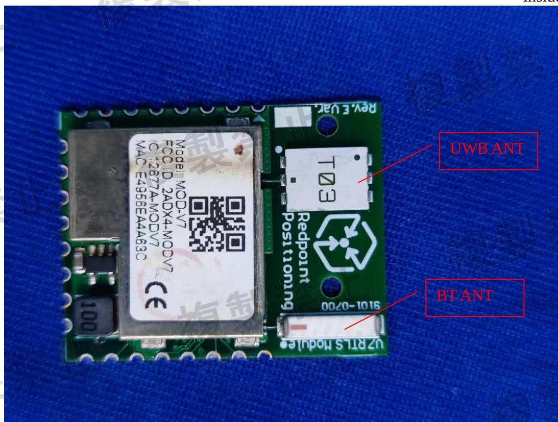
Figure 2 Inside of the EUT
