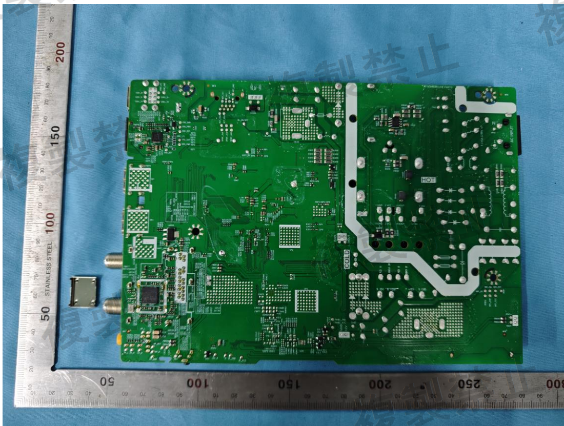
Internal Photo 3
