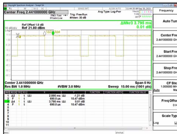
Dwell Time_8DPSK_3M_DH5_2441MHz
