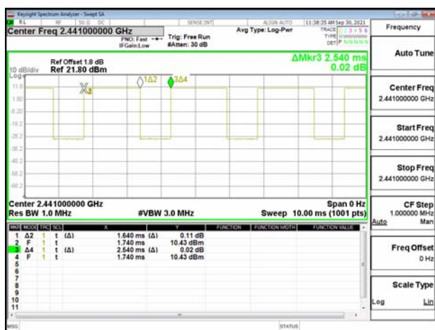
Dwell Time_GFSK_1M_DH5_2441MHz
