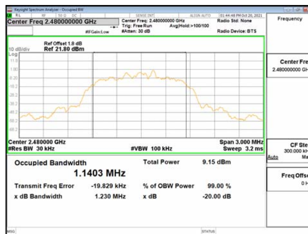
OBW 20dB_π/4DQPSK_2M_DH5_2480MHz
