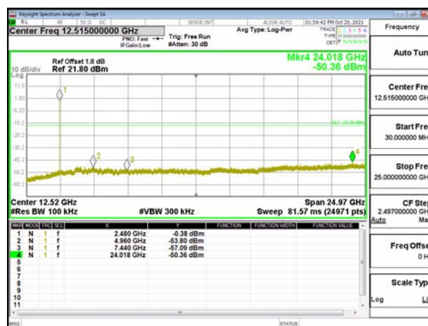
Spurious Emission_8DPSK_3M_DH5_2480MHz
