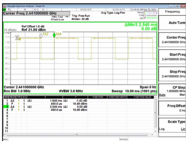
Dwell Time_8DPSK_3M_DH3_2441MHz
