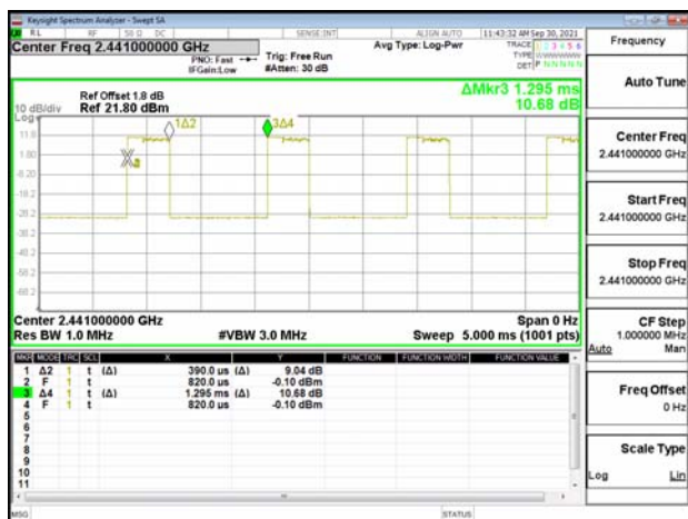
Dwell Time_8DPSK_3M_DH3_2441MHz
