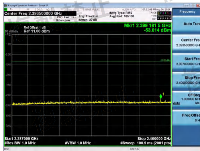
NTNV-11B-Ant1-2442-2387~2400-PASS
