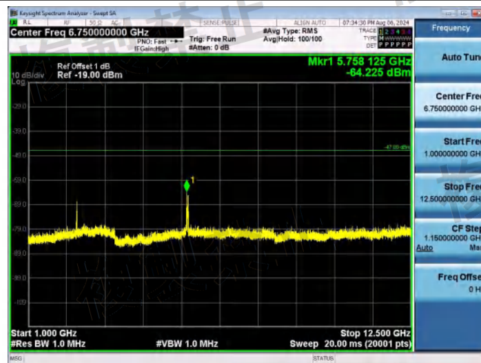
NTNV-11N20SISO-Ant1-2412-1000~12500-PASS
