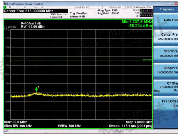
NTNV-11G-Ant1-2442-30~1000-PASS
