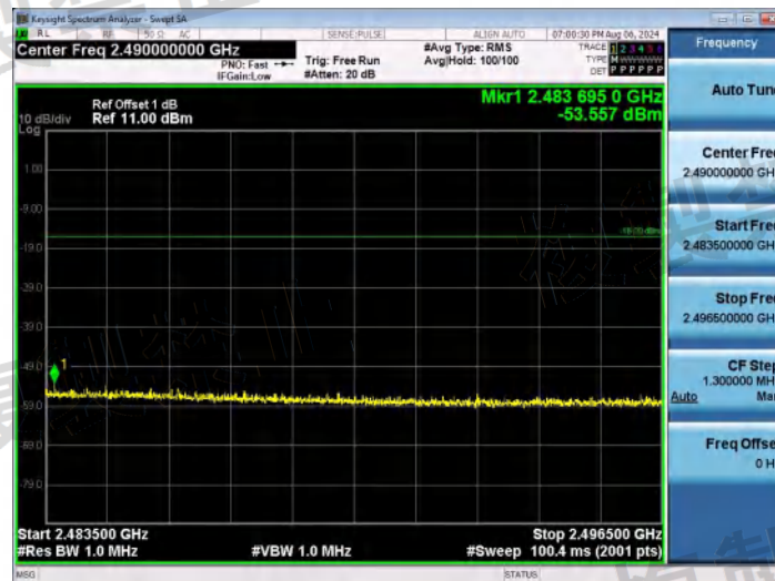
NTNV-11B-Ant1-2412-2483.5~2496.5-PASS
