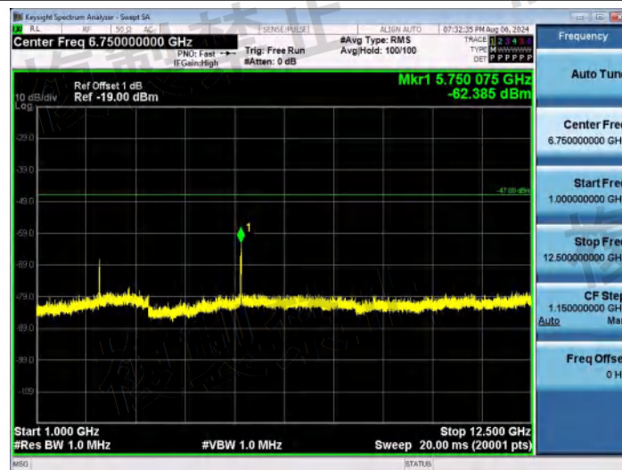
NTVN-11G-Ant1-2412-1000~12500-PASS
