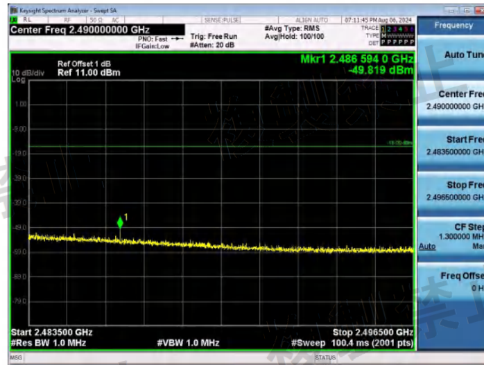
NTNV-11G-Ant1-2442-2483.5~2496.5-PASS
