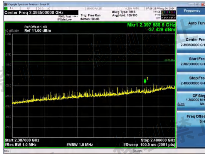
NTNV-11G-Ant1-2412-2387~2400-PASS
