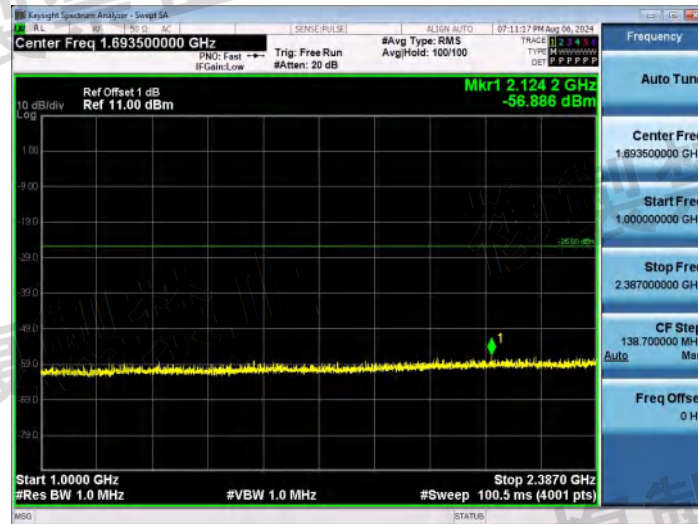
NTNV-11G-Ant1-2442-1000~2387-PASS
