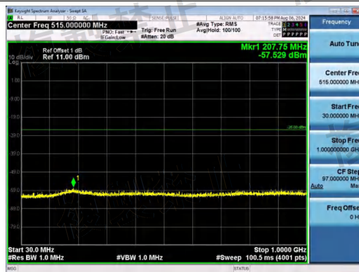
NTNV-11G-Ant1-2472-30~1000-PASS
