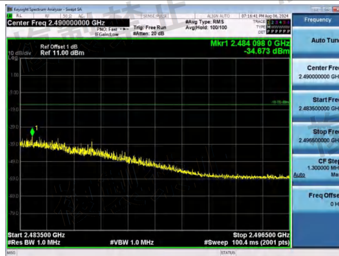
NTNV-11G-Ant1-2472-2483.5~2496.5-PASS
