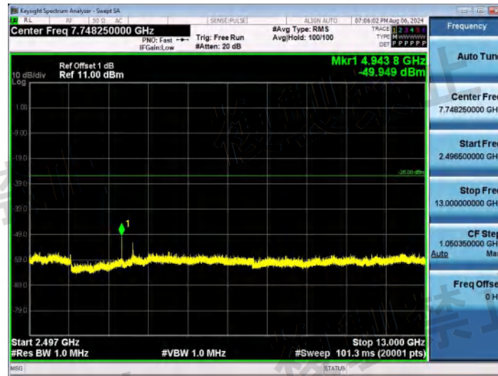
NTNV-11B-Ant1-2472-2496.5~13000-PASS
