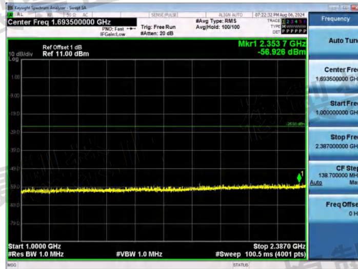
NTNV-11N20SISO-Ant1-2442-1000~2387-PASS
