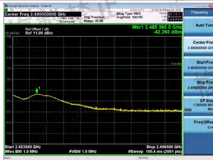
NTNV-11B-Ant1-2472-2483.5~2496.5-PASS
