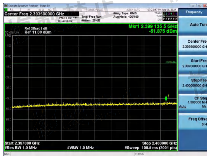
NTNV-11N20SISO-Ant1-2442-2387~2400-PASS
