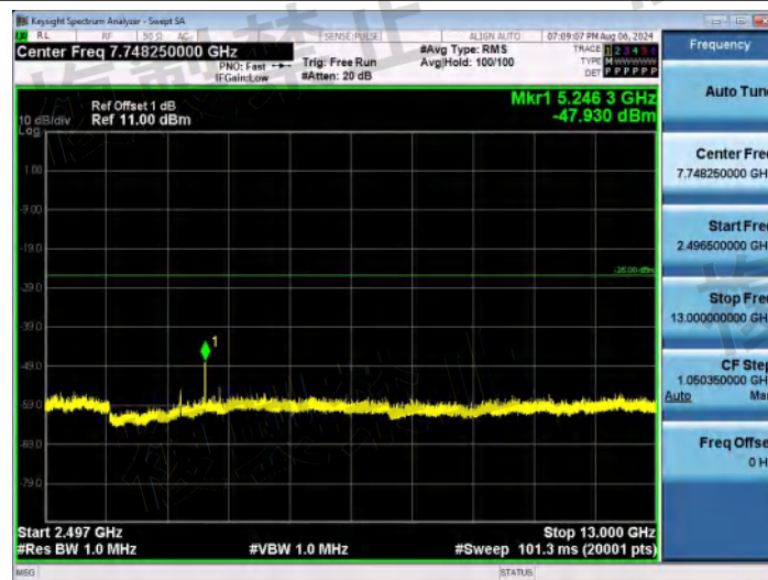
NTNV-11G-Ant1-2412-2496.5~13000-PASS
