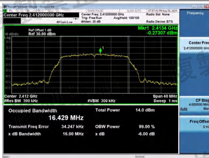
NTNV-11G-Ant1-2412-PASS
