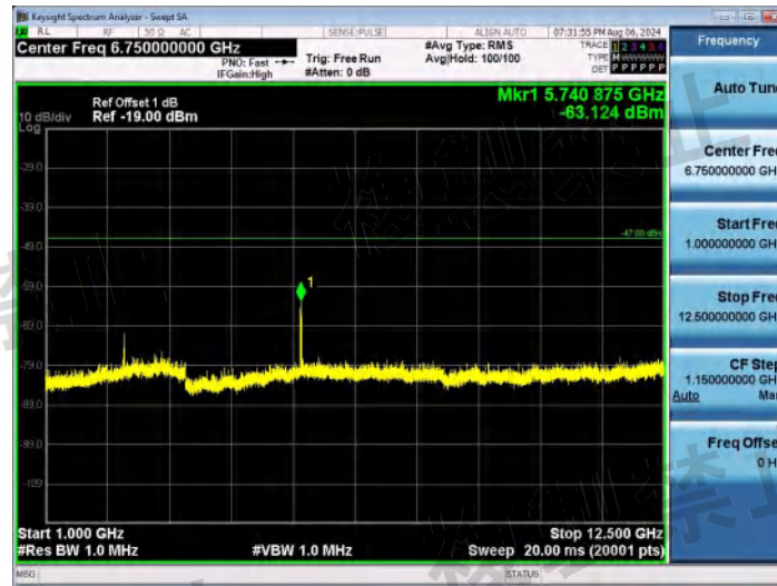
NTVN-11B-Ant1-2472-1000~12500-PASS
