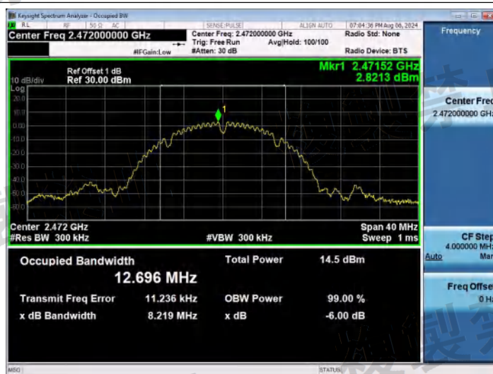
NTNV-11B-Ant1-2472-PASS
