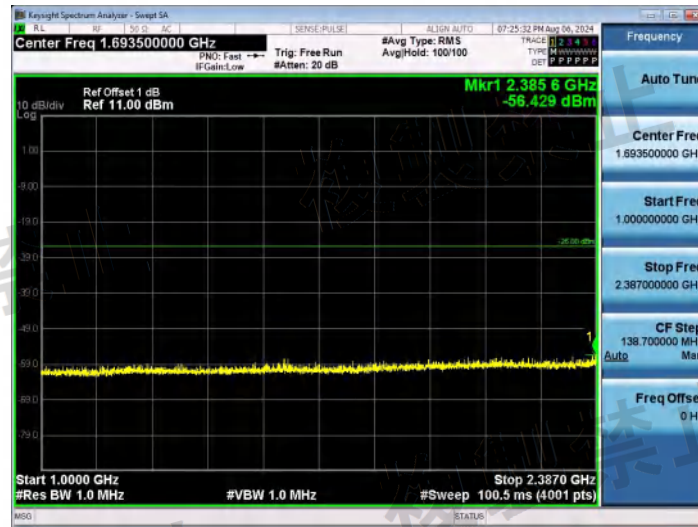
NTNV-11N20SISO-Ant1-2472-1000~2387-PASS
