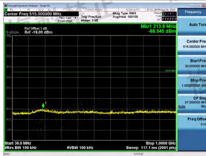
NTNV-11B-Ant1-2472-30~1000-PASS
