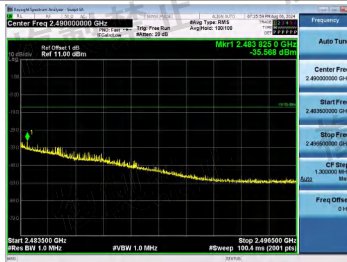
NTNV-11N20SISO-Ant1-2472-2483.5~2496.5-PASS
