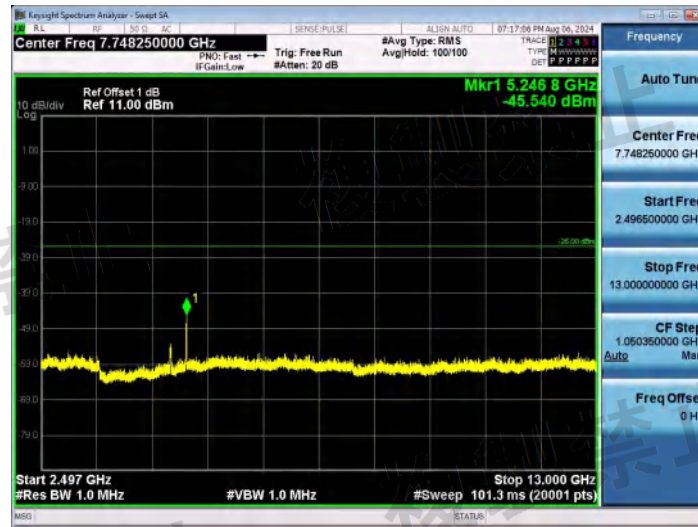
NTNV-11G-Ant1-2472-2496.5~13000-PASS
