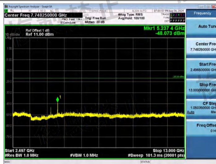
NTNV-11B-Ant1-2412-2496.5~13000-PASS
