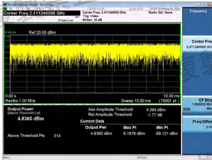
NTNV-11G-Ant1-2412-PASS
