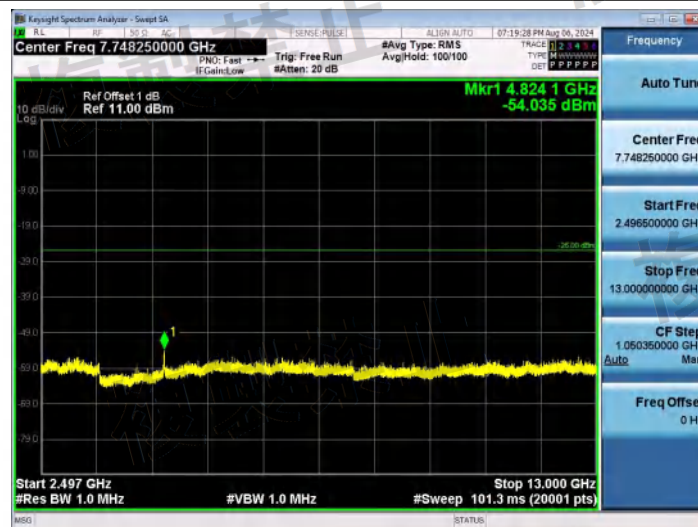
NTNV-11N20SISO-Ant1-2412-2496.5~13000-PASS
