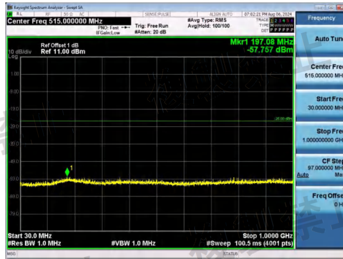
NTNV-11B-Ant1-2442-30~1000-PASS
