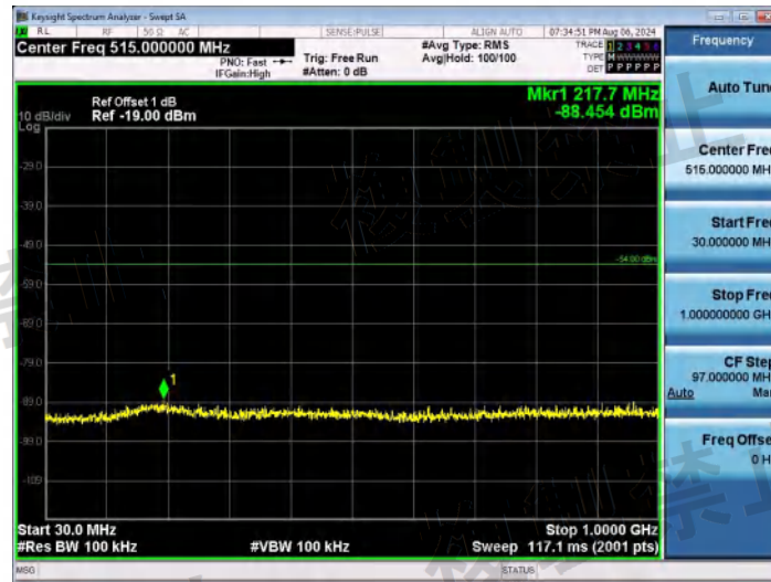
NTNV-11N20SISO-Ant1-2442-30~1000-PASS
