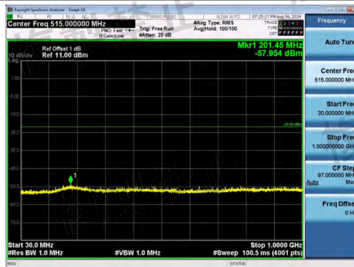
NTNV-11N20SISO-Ant1-2472-30~1000-PASS
