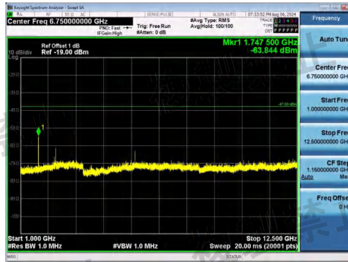
NTNV-11G-Ant1-2472-1000~12500-PASS
