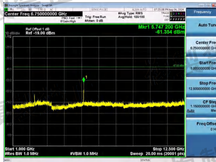
NTNV-11N20SISO-Ant1-2442-1000~12500-PASS
