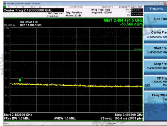
NTNV-11B-Ant1-2442-2483.5~2496.5-PASS
