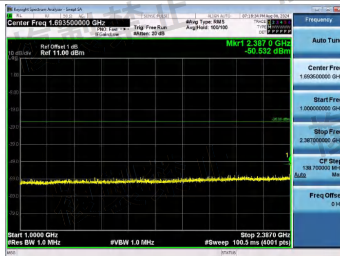
NTNV-11N20SISO-Ant1-2412-1000~2387-PASS
