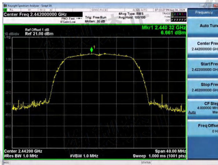
NTNV-11G-Ant1-2442-PASS
