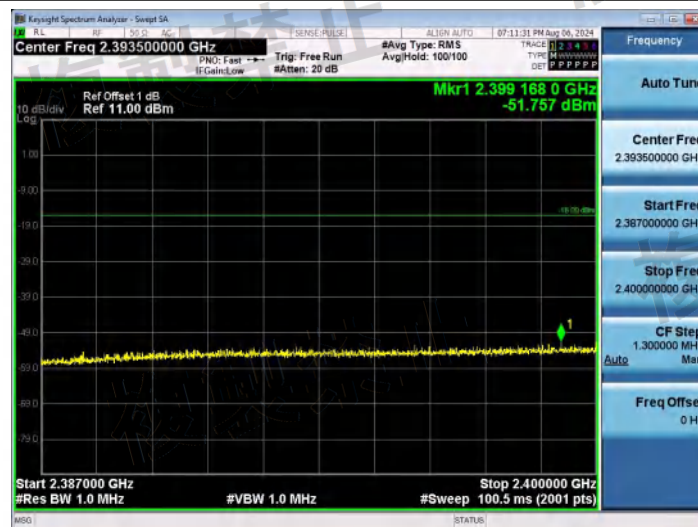
NTNV-11G-Ant1-2442-2387~2400-PASS
