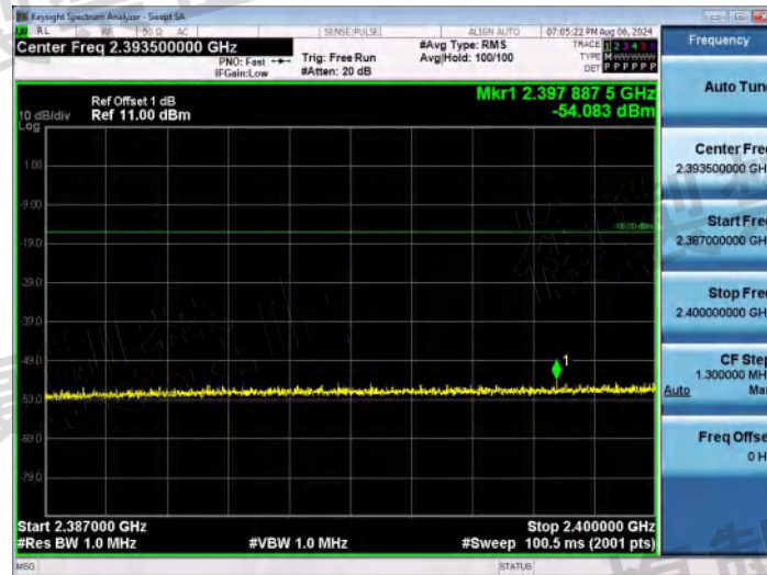
NTNV-11B-Ant1-2472-2387~2400-PASS
