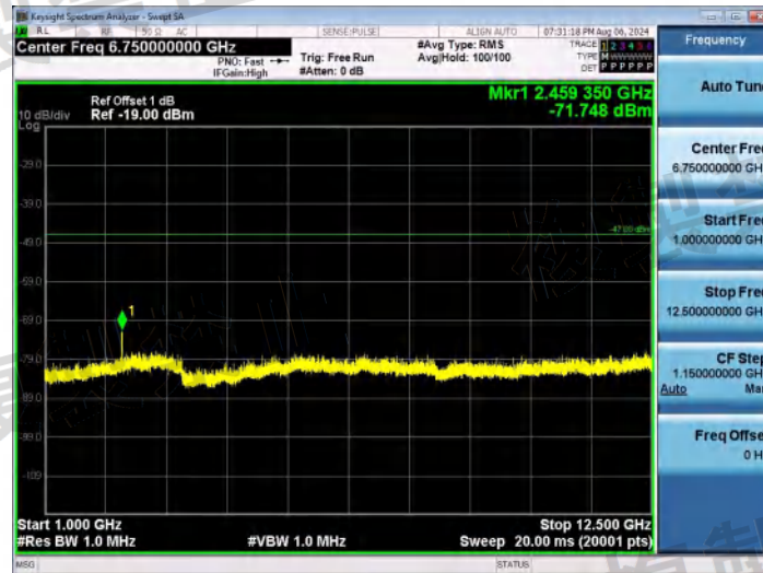
NTNV-11B-Ant1-2442-1000~12500-PASS
