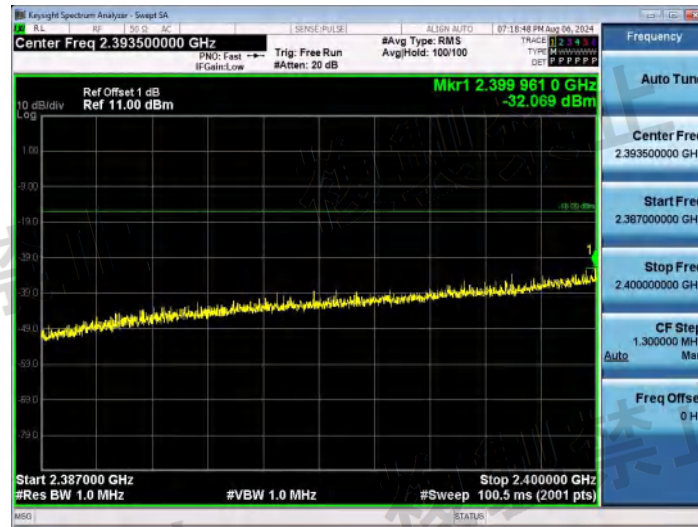
NTNV-11N20SISO-Ant1-2412-2387~2400-PASS
