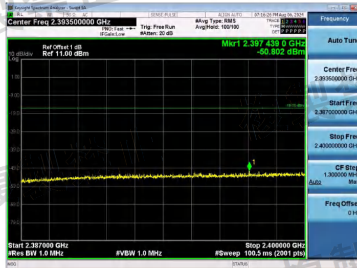
NTNV-11G-Ant1-2472-2387~2400-PASS
