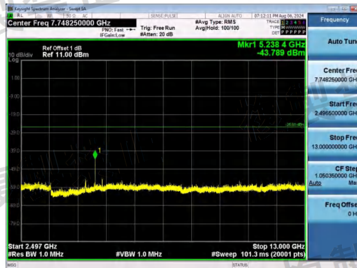
NTNV-11G-Ant1-2442-2496.5~13000-PASS
