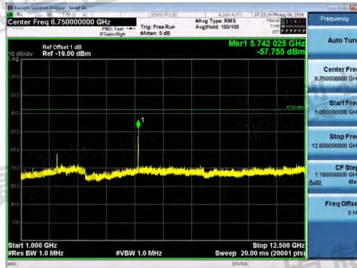
NTNV-11G-Ant1-2442-1000~12500-PASS
