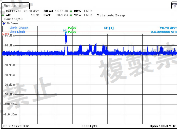
NTNV-11AC20MIMO-Ant2-5320-30~5233.3-PASS
