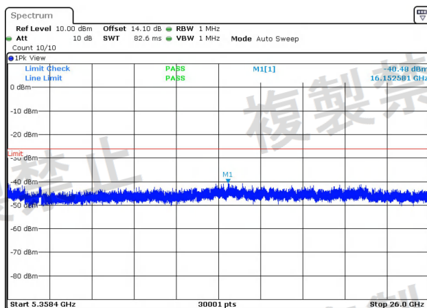
NTNV-11AC40MIMO-Ant1-5270-5358.4~26000-PASS
