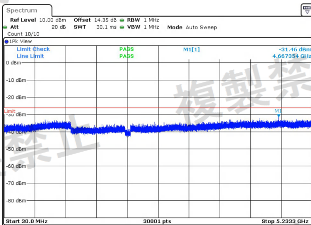
NTNV-11AC20MIMO-Ant1-5320-30~5233.3-PASS
