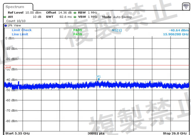
NTNV-11N20MIMO-Ant2-5320-5350~26000-PASS
