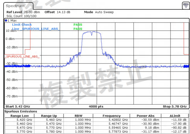
NTNV-11AC40MIMO-Ant2-5710-5420~5460-PASS
