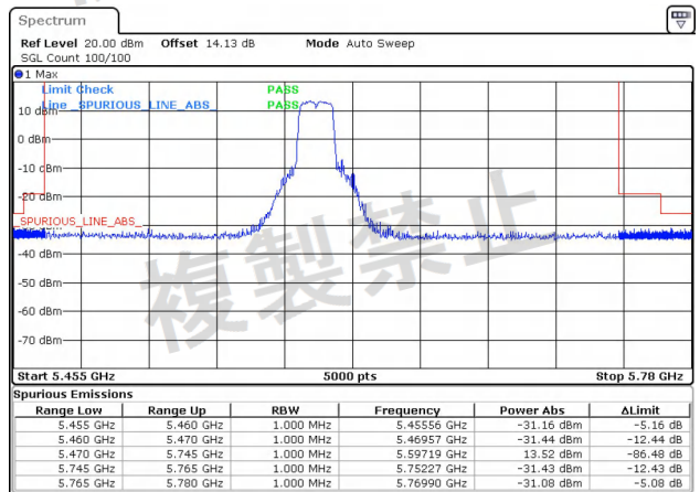
NTNV-11A-Ant2-5720-5455~5460-PASS
