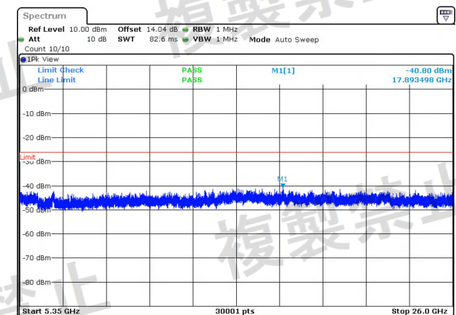
NTNV-11AC20MIMO-Ant2-5260-5350~26000-PASS
