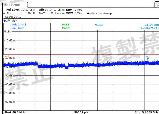
NTNV-11AC80MIMO-Ant1-5290-30~5203.3-PASS
