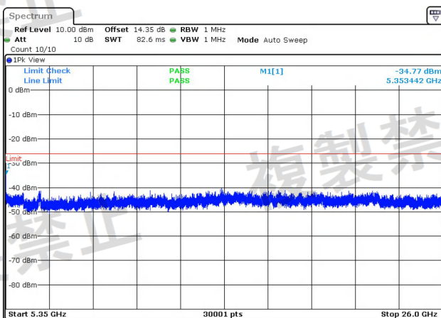
NTNV-11N20MIMO-Ant1-5320-5350~26000-PASS
