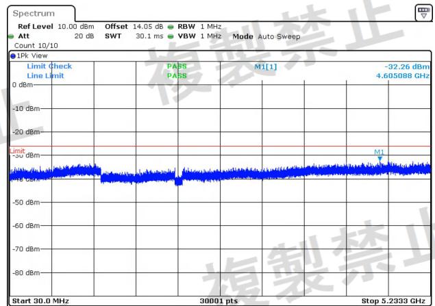
NTNV-11N20MIMO-Ant2-5300-30~5233.3-PASS
