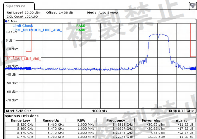
NTNV-11AC40MIMO-Ant2-5710-5420~5460-PASS
