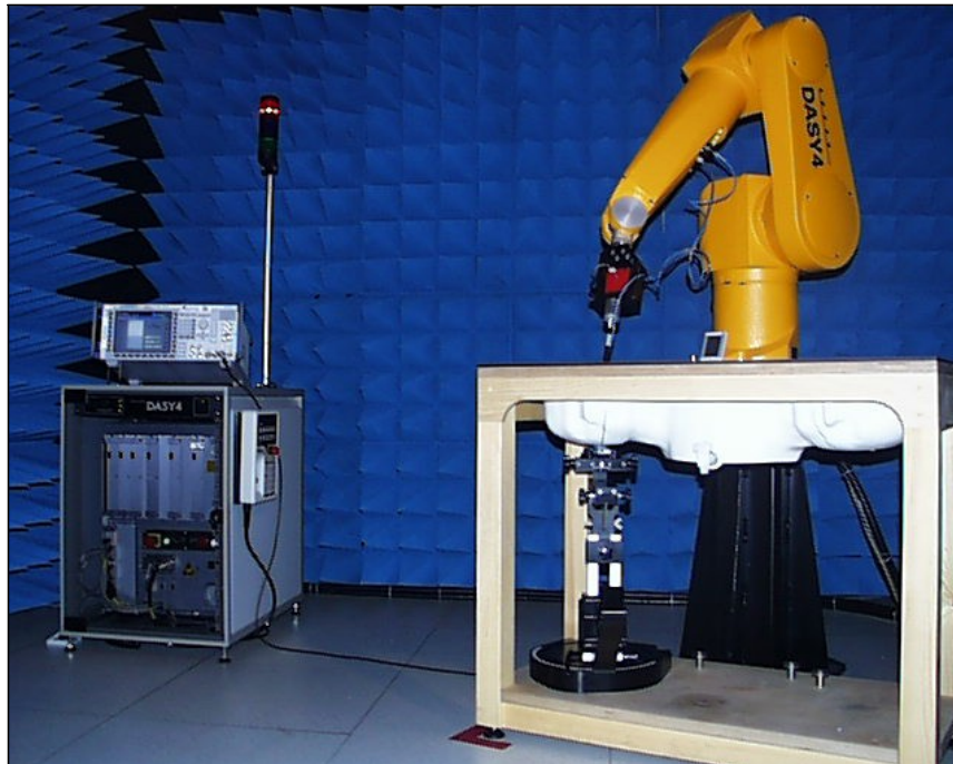
Fig. 7: The measurement setup with equipment under test
