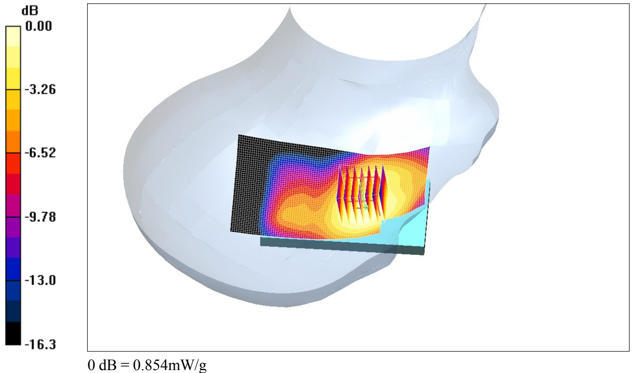
Fig. 4: SAR distribution for GSM1800 of the mobile phone alone: channel 699 (1747.6MHz), cheek position, right side
