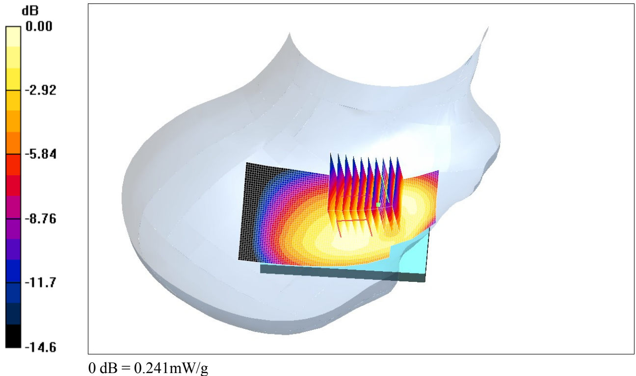
Fig. 3: SAR distribution for GSM900 of the mobile phone with FAZUP: channel 38 (897.6 MHz), cheek position, right side
