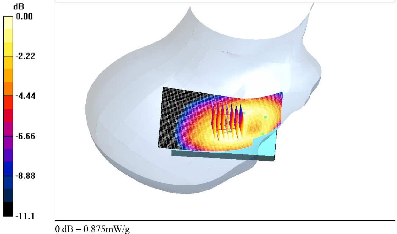
Fig. 2: SAR distribution for GSM900 of the mobile phone alone: channel 38 (897.6 MHz), cheek position, right side
