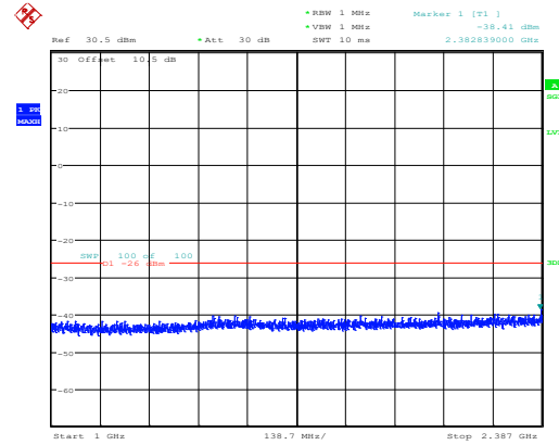
BLE 1Mbps_Low Channel(1GHz~2.387GHz)
