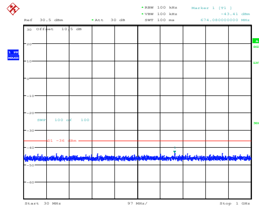
BLE 1Mbps_Middle Channel(30MHz~1GHz)
