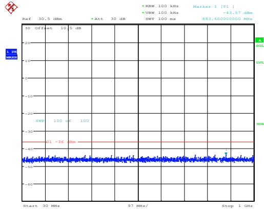
BLE 1Mbps_Low Channel(30MHz~1GHz)
