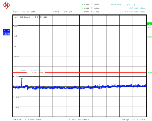
BLE 1Mbps_Low Channel(2.4965GHz~12.5GHz)
