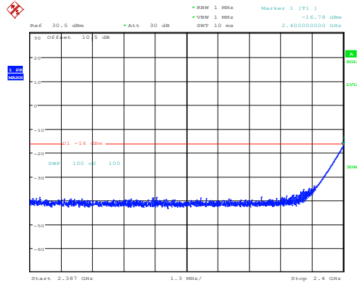
BLE 1Mbps_Low Channel(2.387GHz~2.4GHz)
