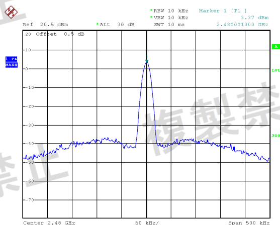
Channel 2480MHz
