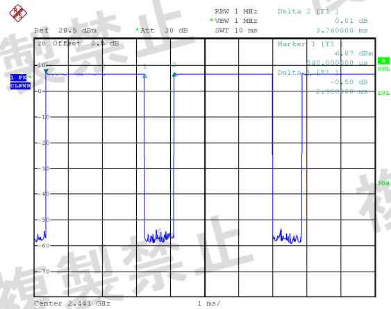
Channel 2441MHz
