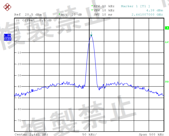
Channel 2441MHz
