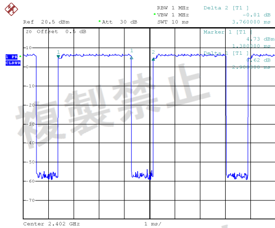
Channel 2402MHz
