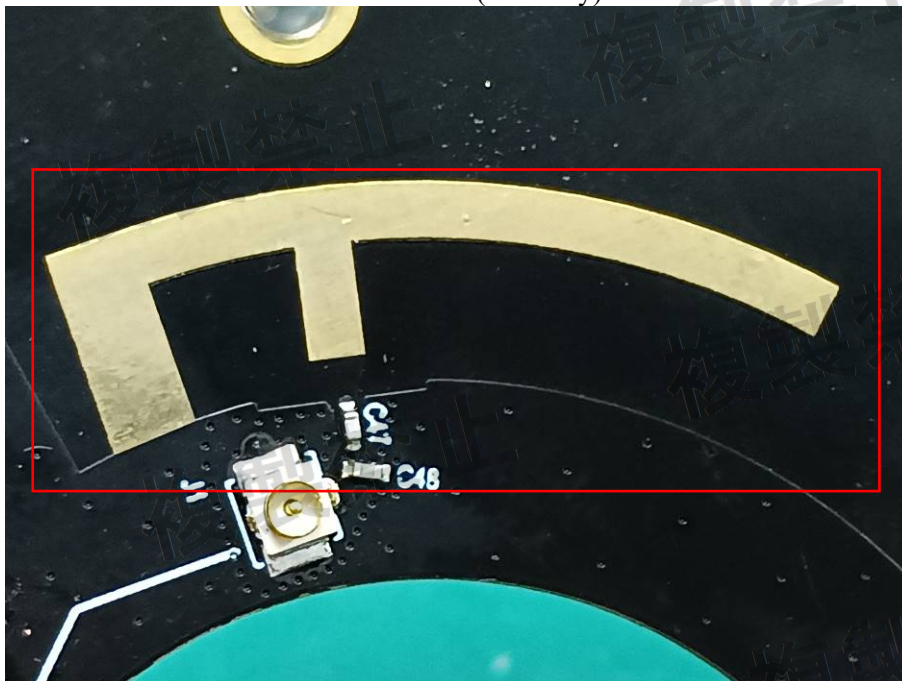
CMRX ANT (RX Only)
