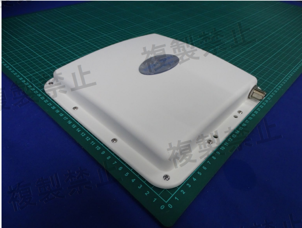
(73) EUT Photo_ Antenna: MOXA / ANT-WSB-PNF-12-02
