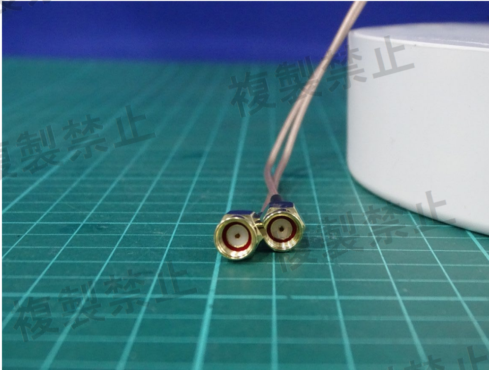
(57) EUT Photo_ Antenna: MOXA / MAT-WDB-CA-RM-2-0205
