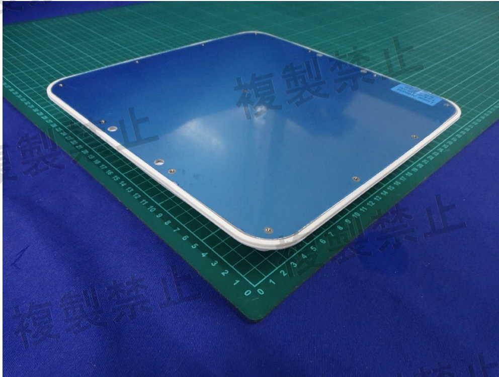
(65) EUT Photo_ Antenna: MOXA / ANT-WDB-PNF-1011
