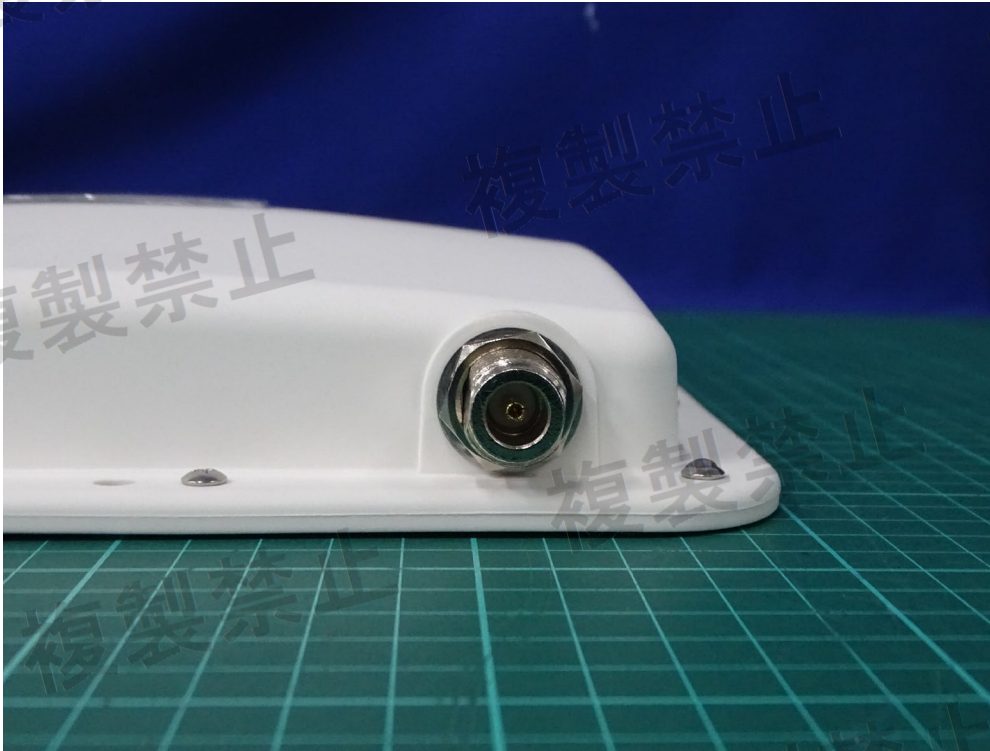
(75) EUT Photo_ Antenna: MOXA / ANT-WSB-PNF-12-02
