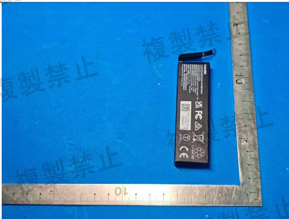
EUT Photo(12) Battery (Chongqing VDL New Energy Co.,Ltd.)
