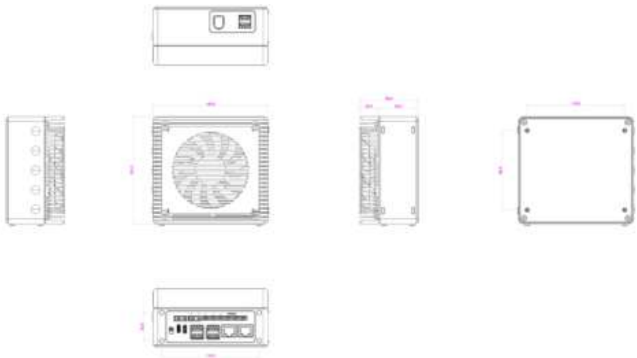
Figure 6. Orthographic view of reComputer Robotics J401 PCBA
