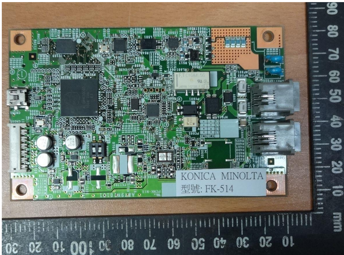
相片一：傳真卡(廠牌/型號：KONICA MINOLTA /FK-514)電路板正面照 (適用機種廠牌：KONICA MINOLTA型號：bizhub C368、bizhub C308,bizhub C258, KONICA MINOLTA bizhub C368, KONICA MINOLTA bizhub C308, KONICA MINOLTA bizhub C258)
