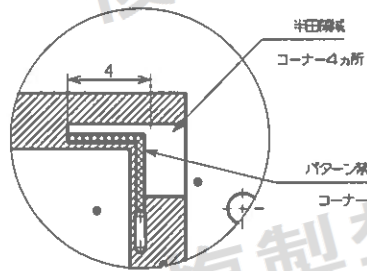
DETAIL A SOL. 4:1
