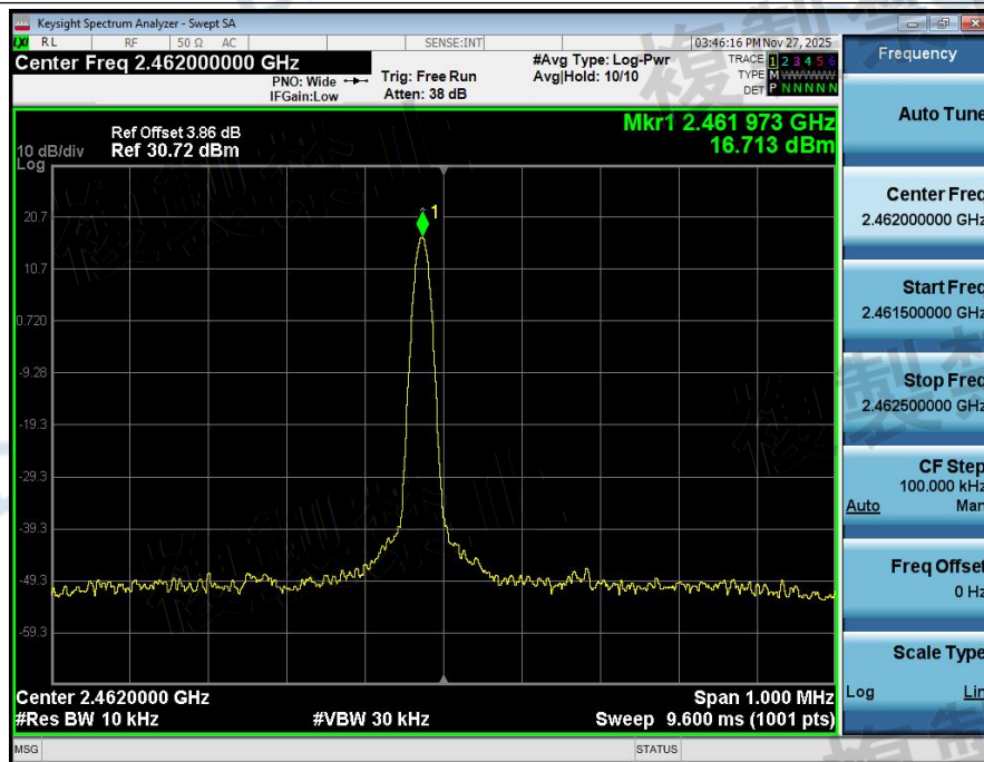
Frequency_Tolerance_NTLV_ANT1_802_11n(HT40)_2462
