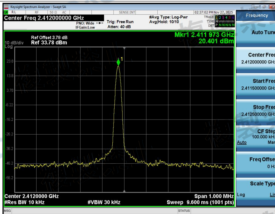
Frequency_Tolerance_NTHV_ANT1_802_11b_2412
