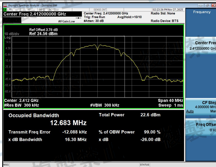
Occupied_Frequency_Bandwidth_NVNT_ANT1_802_11b_2412
