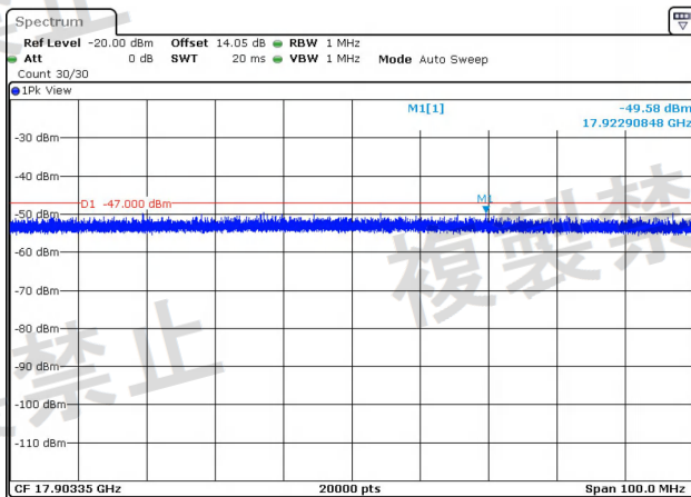
NTNV-11AC80MIMO-Ant2-5290-1000~26000-PASS
