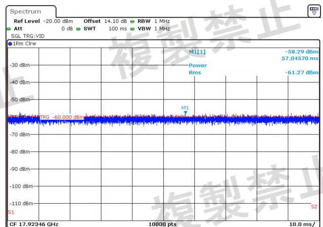
NTNV-11AC80MIMO-Ant1-5290-1000~26000-PASS
