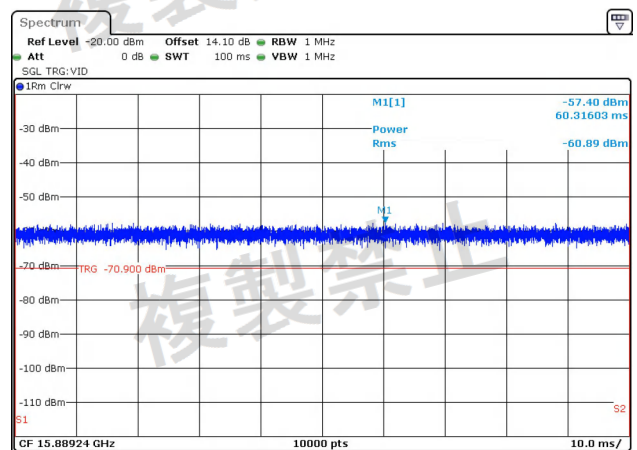
NTNV-11AC40MIMO-Ant2-5310-1000~26000-PASS
