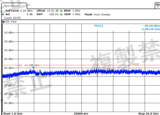
NTNV-11A-Ant1-5720-1000~26000-See table below
