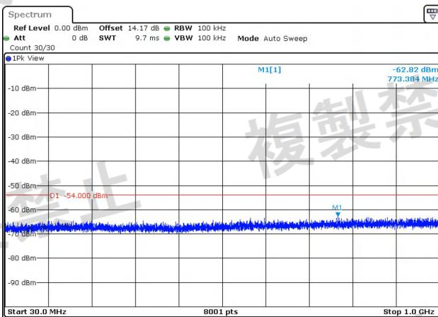
NTNV-11N20MIMO-Ant1-5600-30~1000-See table below
