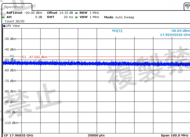
NTNV-11AC80MIMO-Ant1-5290-1000~26000-PASS
