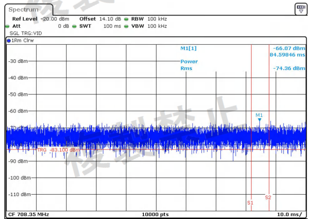
NTNV-11AC40MIMO-Ant2-5310-30~1000-PASS
