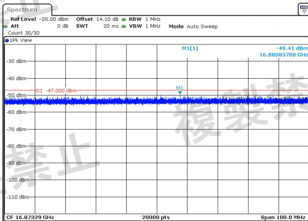
NTNV-11AC40MIMO-Ant1-5270-1000~26000-PASS
