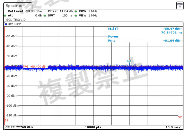
NTNV-11AC40MIMO-Ant1-5270-1000~26000-PASS
