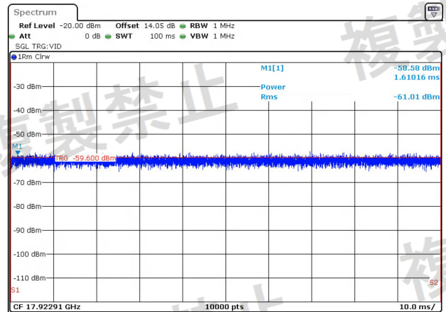
NTNV-11AC80MIMO-Ant1-5290-1000~26000-PASS
