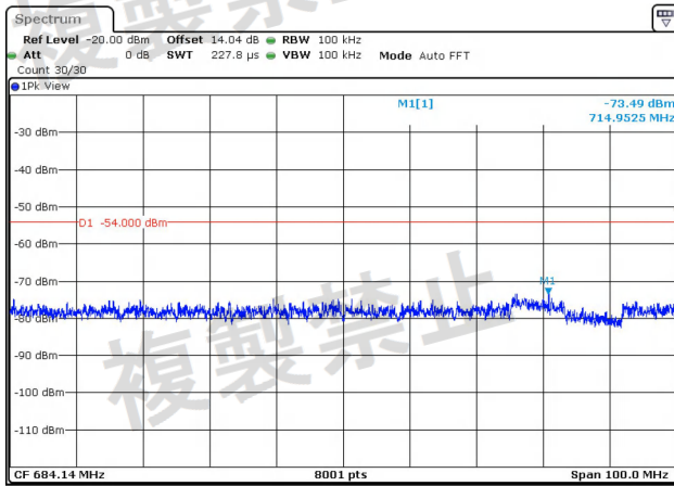
NTNV-11AC40MIMO-Ant1-5270-30~1000-PASS
