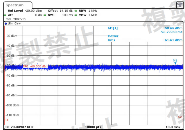
NTNV-11AC40-Ant2-5310-1000~26000-PASS
