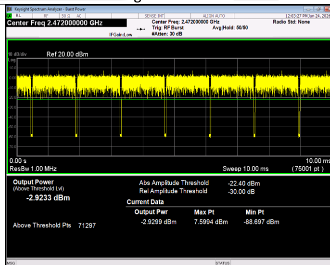
g 2472MHz Zero Span
