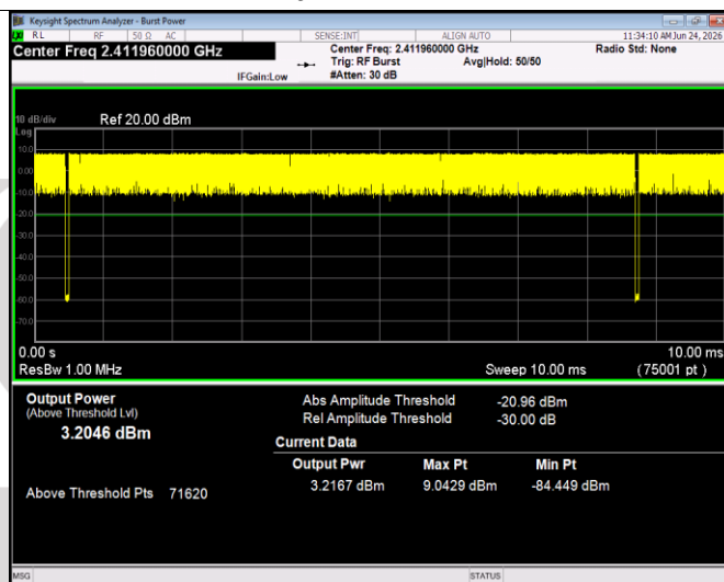
b 2412MHz Zero Span
