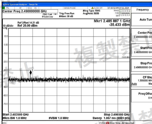
NTHV_3DH5_Ant1_2441_2496.5~13000
