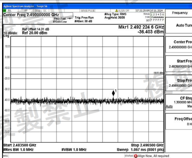
NTLV_3DH5_Ant1_2480_2496.5~13000
