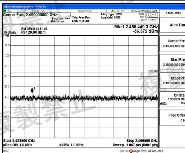
NTNV_3DH5_Ant1_2480_2496.5~13000
