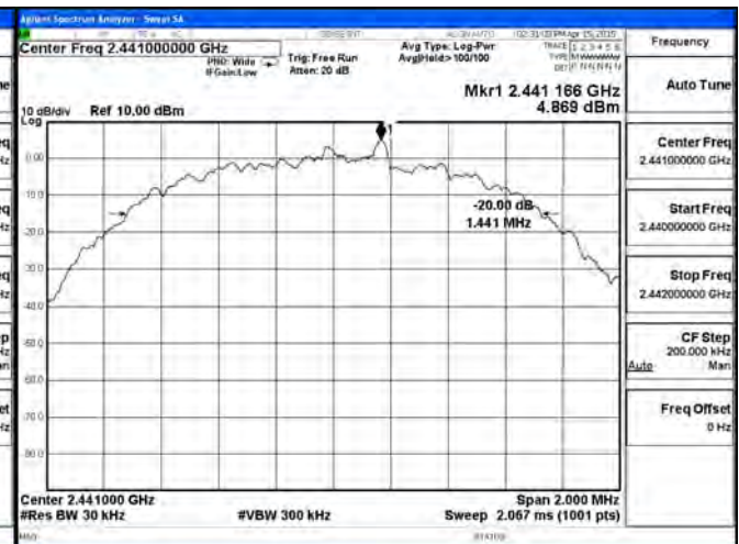
20dB Bandwidth
