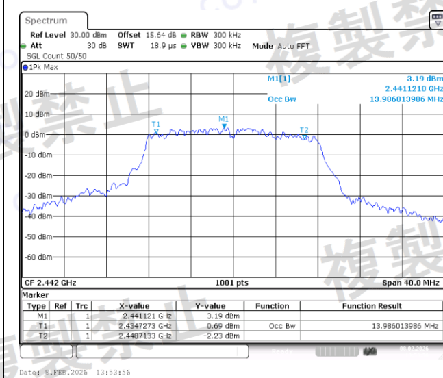
NTNV-11G-Ant1-2442-PASS
