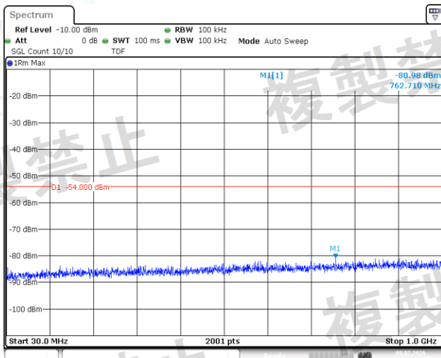
NTNV-11N20SISO-Ant1-2442-30~1000-PASS
