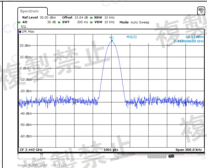
NTNV-Ant1-2442-PASS
