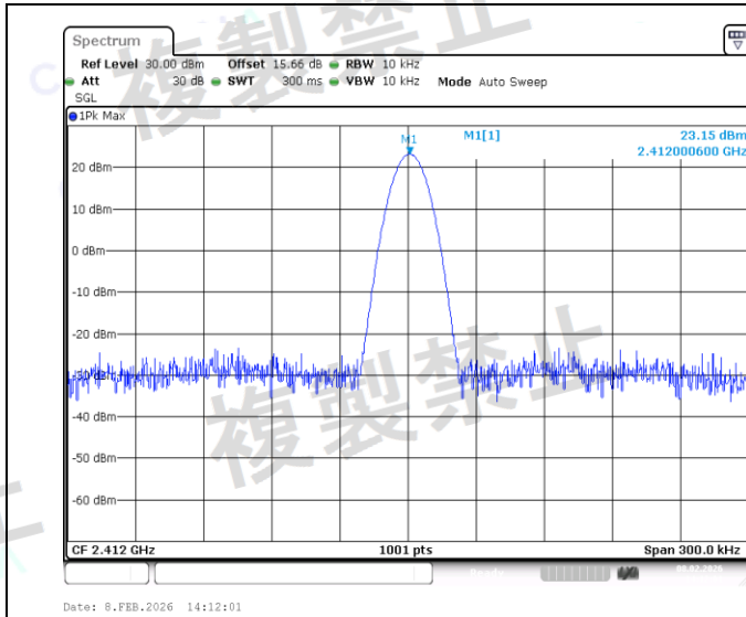
NTNV-Ant1-2412-PASS
