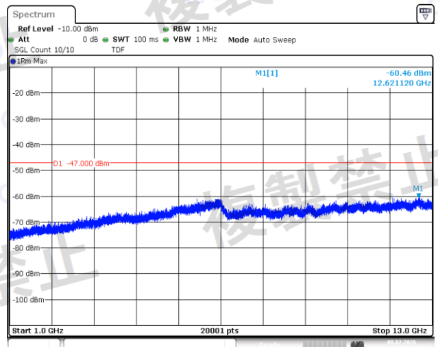
NTNV-11N20SISO-Ant1-2442-1000~13000-PASS
