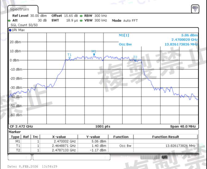
NTNV-11G-Ant1-2472-PASS
