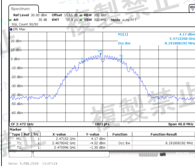
NTNV-11B-Ant1-2472-PASS
