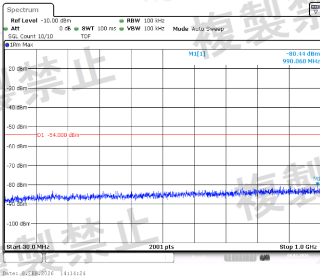
NTNV-11B-Ant1-2472-30~1000-PASS
