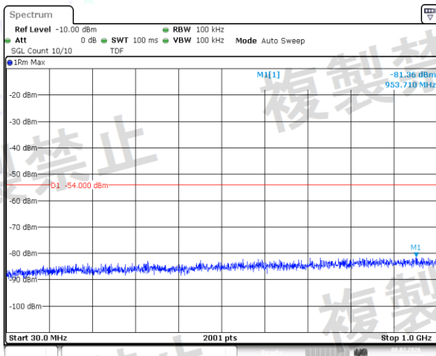
NTNV-11G-Ant1-2442-30~1000-PASS
