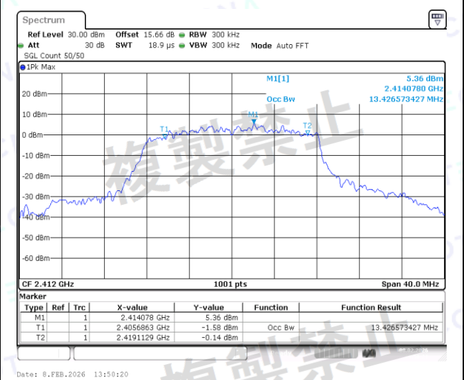
NTNV-11G-Ant1-2412-PASS
