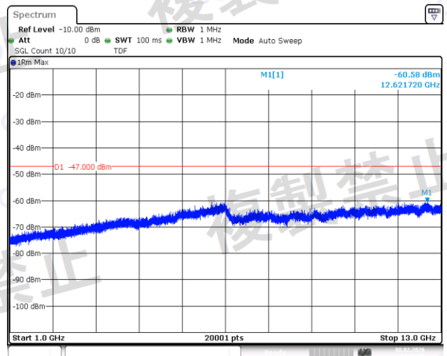
NTNV-11G-Ant1-2442-1000~13000-PASS
