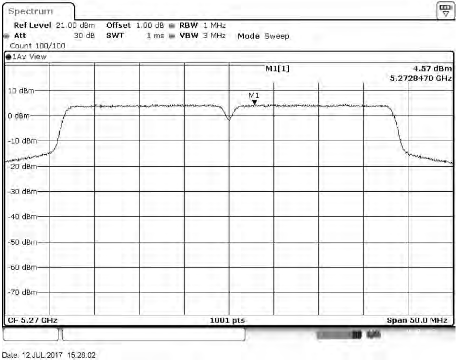
Channel 54: Chain B
