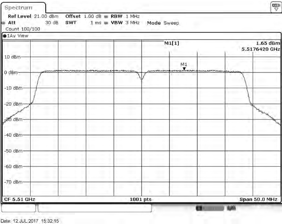
Channel 102: Chain B
