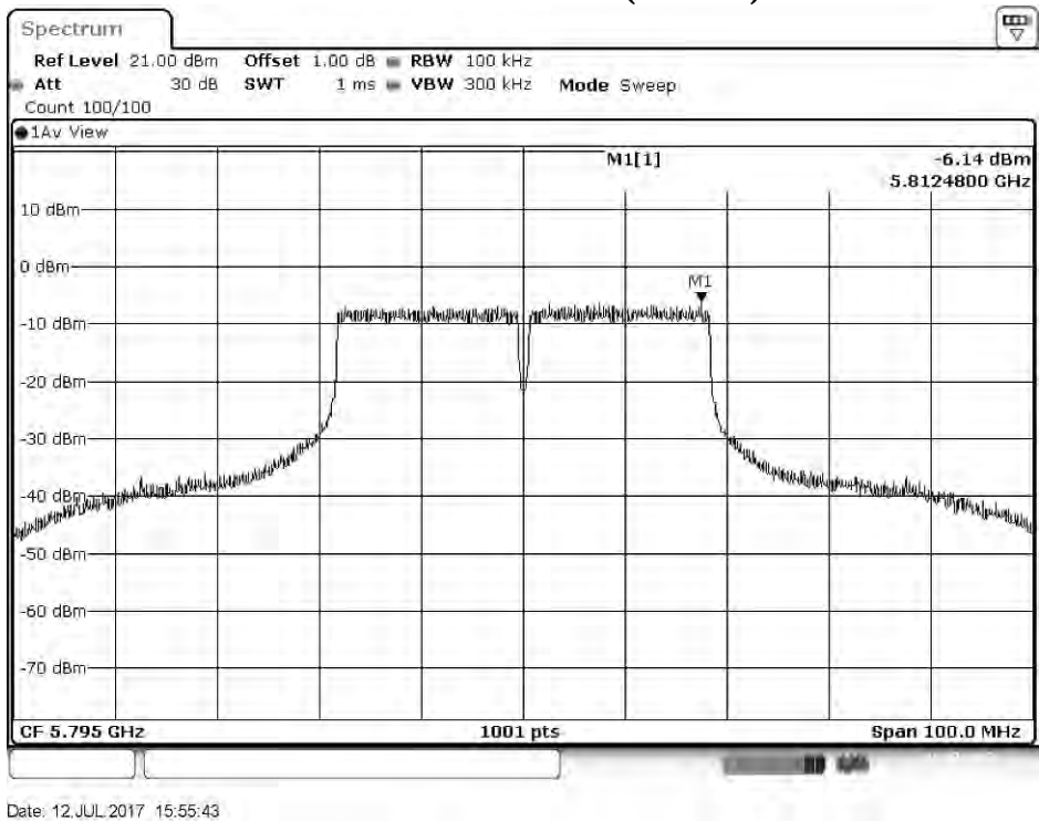
Channel 159: (Chain B)
