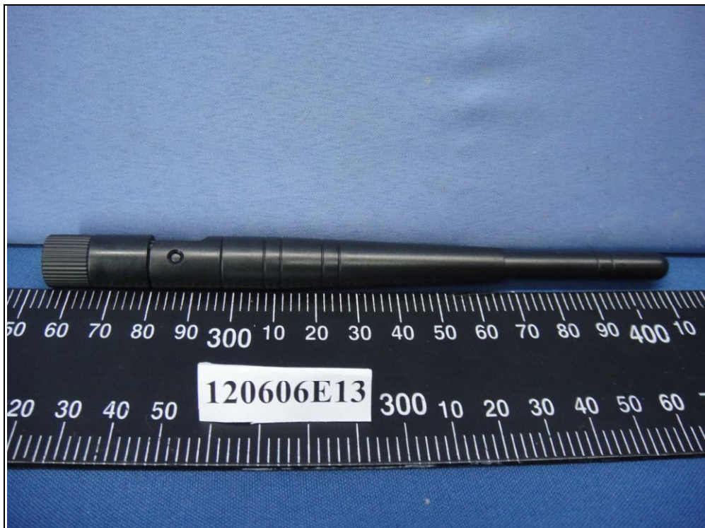
Antenna set 10 Dipole Antenna (Brand name: ARISTOTLE ENTERPRISES., LTD, Model No.: RFA-02-3-C52M3)
