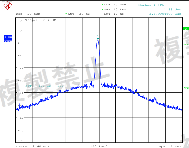
NTNV_2DH5_Ant1_2480
