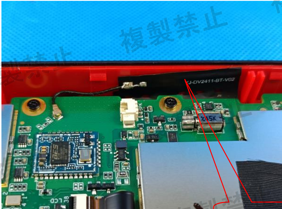
BT FPC Antenna
