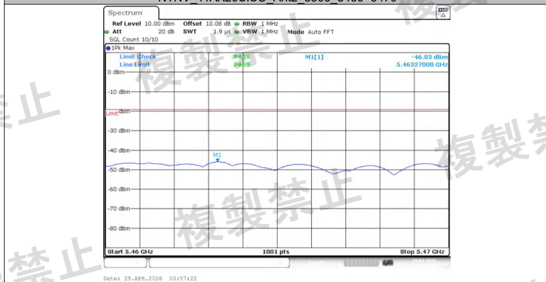
NTNV_11AX20SISO_Ant2_5500_5745~5765
