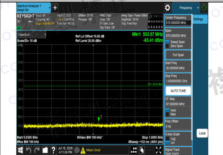
NTNV-BLE 2M-Ant1-2402-30~1000-PASS
