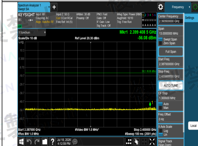
NTNV-BLE_2M-Ant1-2440-2387~2400-PASS
