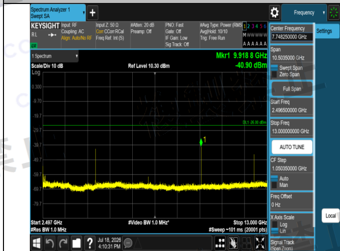
NTNV-BLE 1M-Ant1-2480-2496.5~13000-PASS
