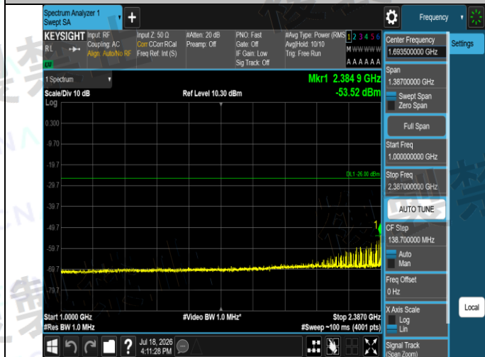
NTNV-BLE 2M-Ant1-2402-1000~2387-PASS
