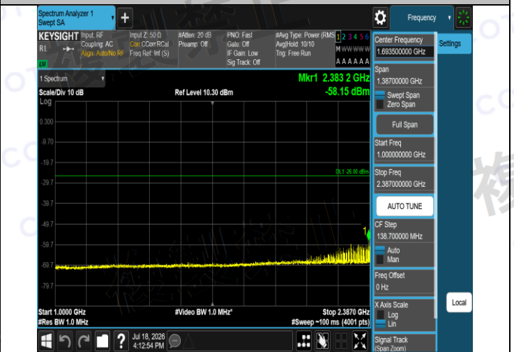
NTNV-BLE_2M-Ant1-2440-1000~2387-PASS
