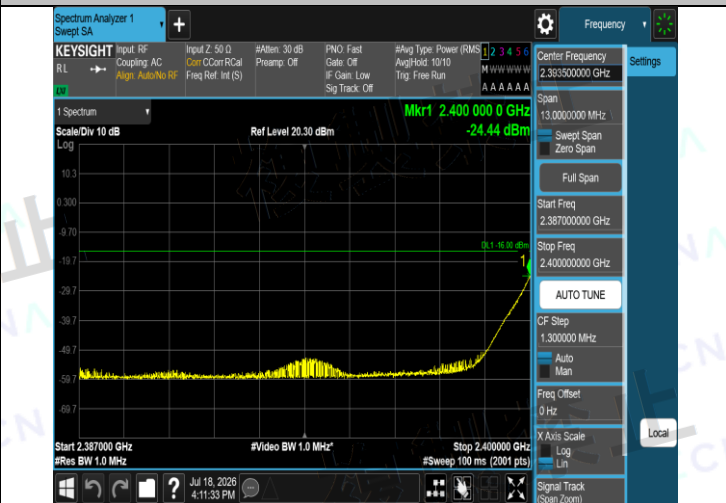
NTNV-BLE 2M-Ant1-2402-2387~2400-PASS
