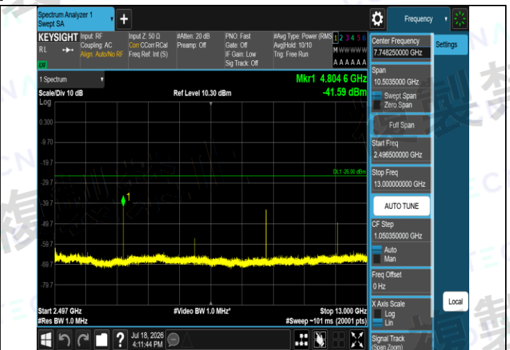
NTNV-BLE_2M-Ant1-2402-2496.5~13000-PASS
