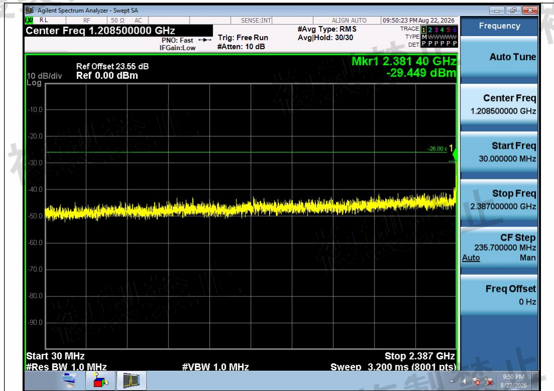
NTNV-11N40SISO-Ant1-2422-30~2387-See table below
