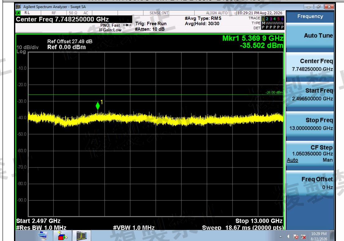
NTNV-11N40SISO-Ant1-2442-2496.5~13000-PASS
