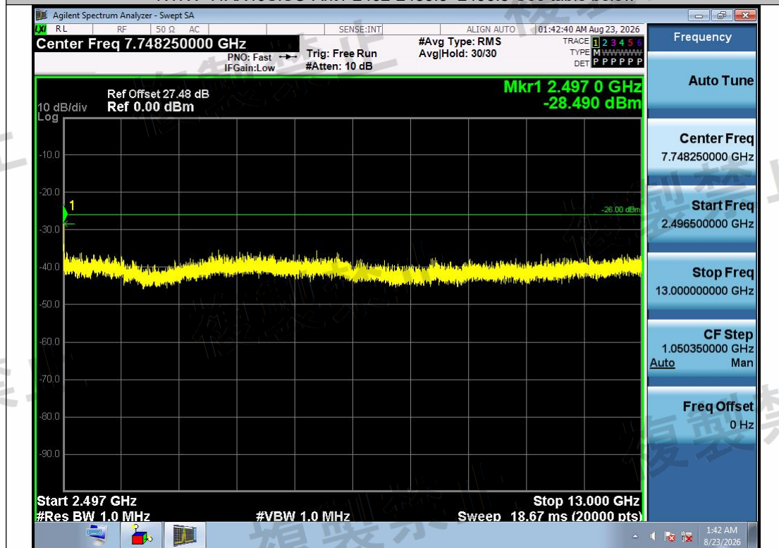
NTNV-11AX40SISO-Ant1-2462-2496.5~13000-See table below
