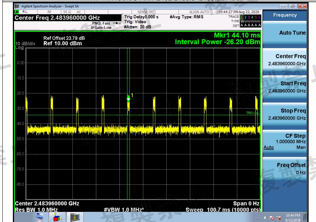
NTNV-11N40SISO-Ant1-2462-2483.5~2496.5-PASS
