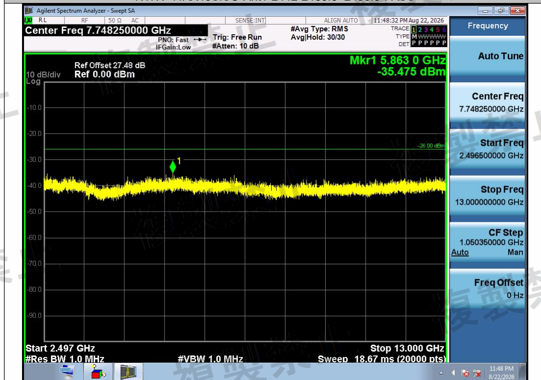
NTNV-11AX40SISO-Ant1-2442-2496.5~13000-PASS
