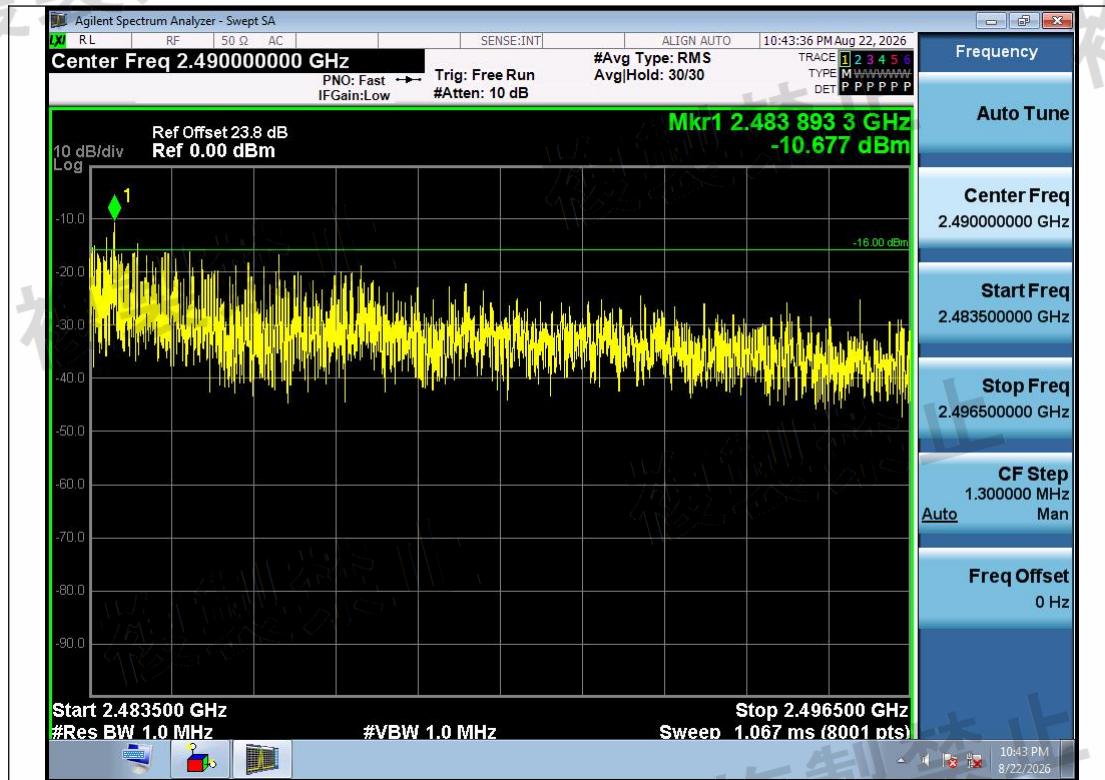
NTNV-11N40SISO-Ant1-2462-2483.5~2496.5-See table below
