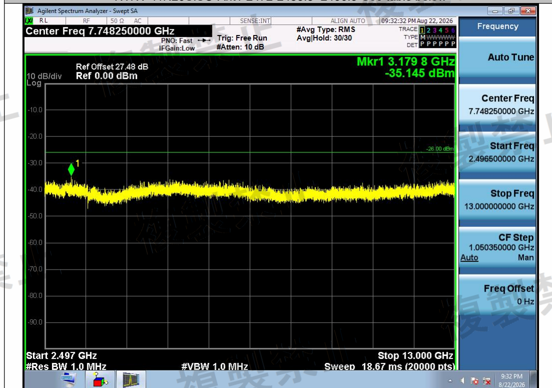
NTNV-11N20SISO-Ant1-2472-2496.5~13000-PASS
