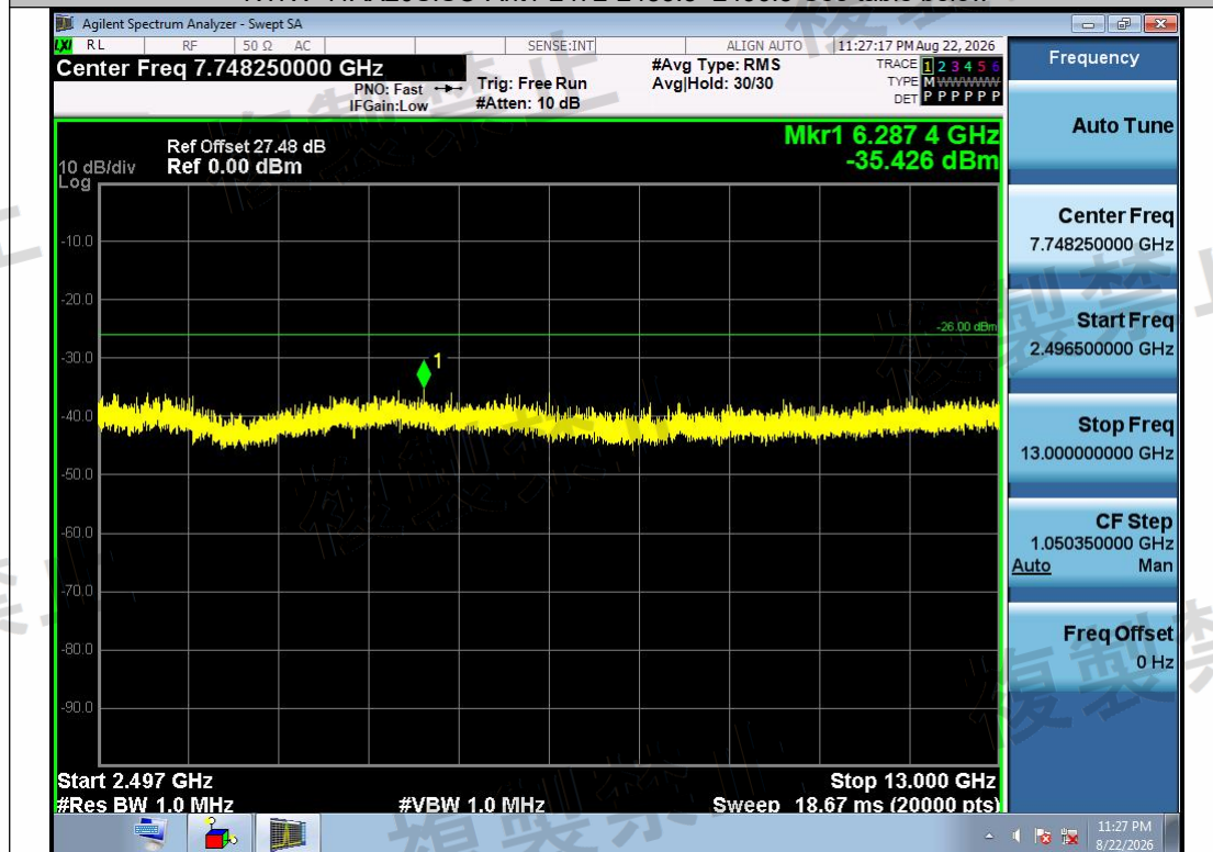
NTNV-11AX20SISO-Ant1-2472-2496.5~13000-PASS
