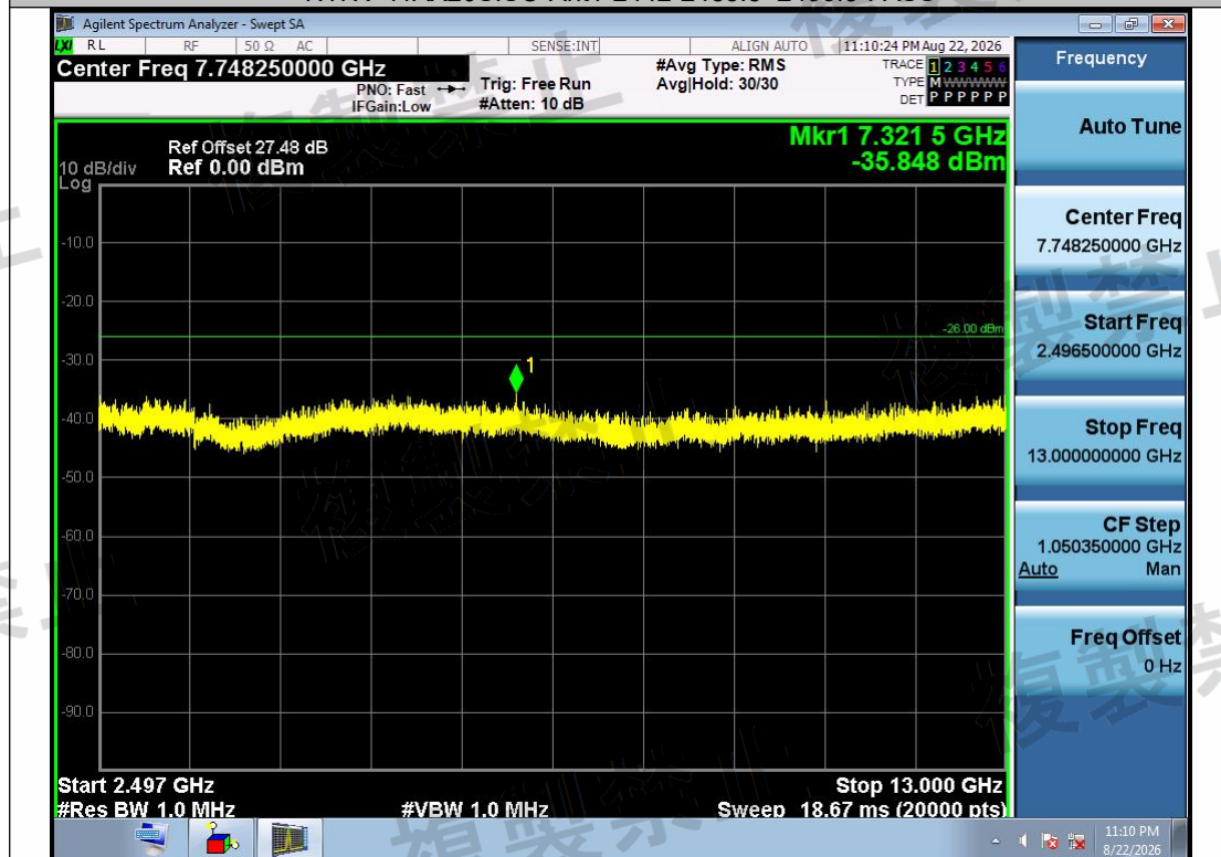
NTNV-11AX20SISO-Ant1-2442-2496.5~13000-PASS
