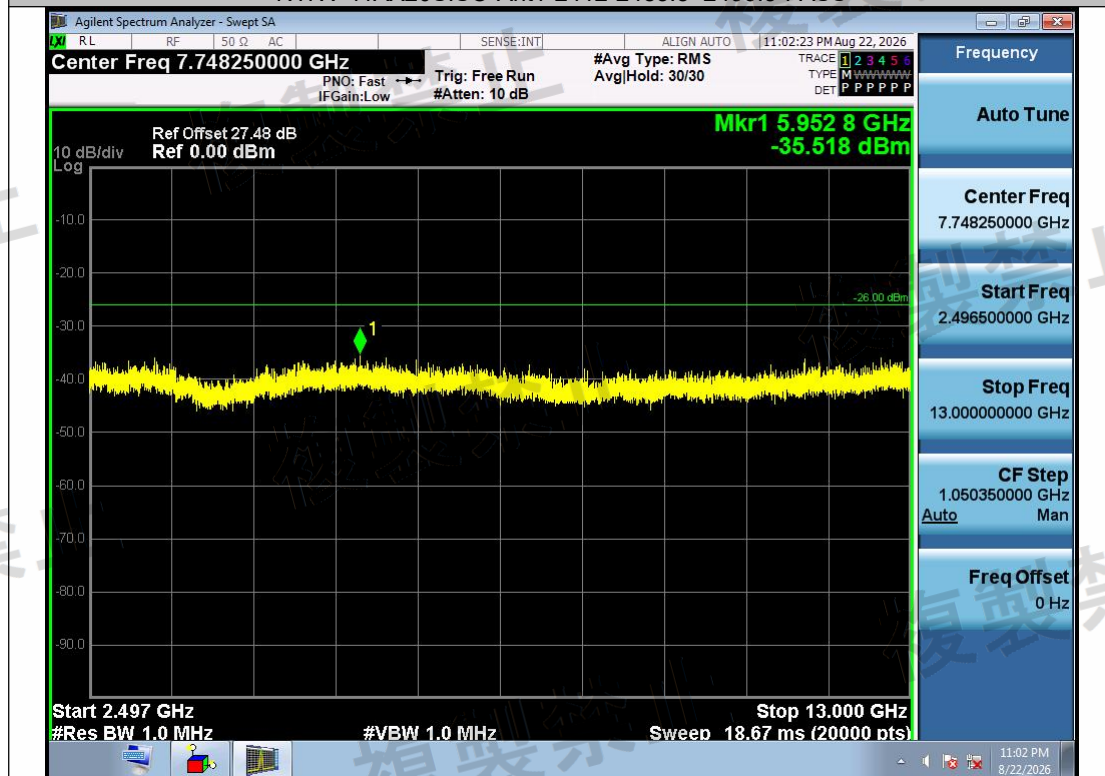
NTNV-11AX20SISO-Ant1-2412-2496.5~13000-PASS
