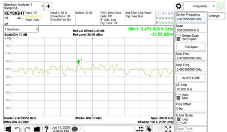
功率密度_BLE_2M_HighCH39-2480
