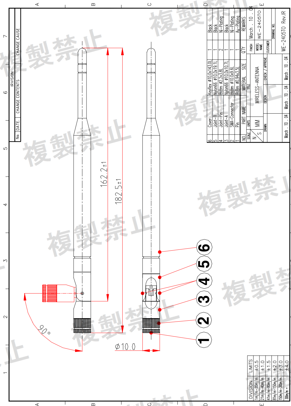
Fig 7. Antenna Mechanical
