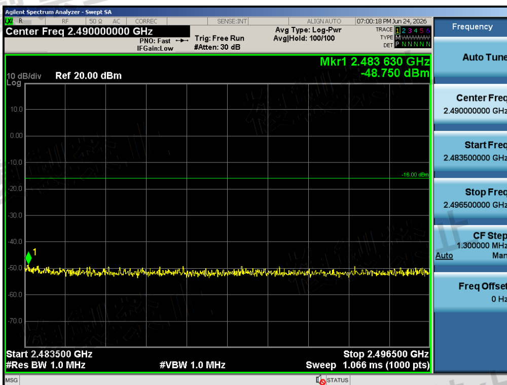
Test Graph BR ANT1 2480 1Mbps 2483.5 2496.5MHz LV
