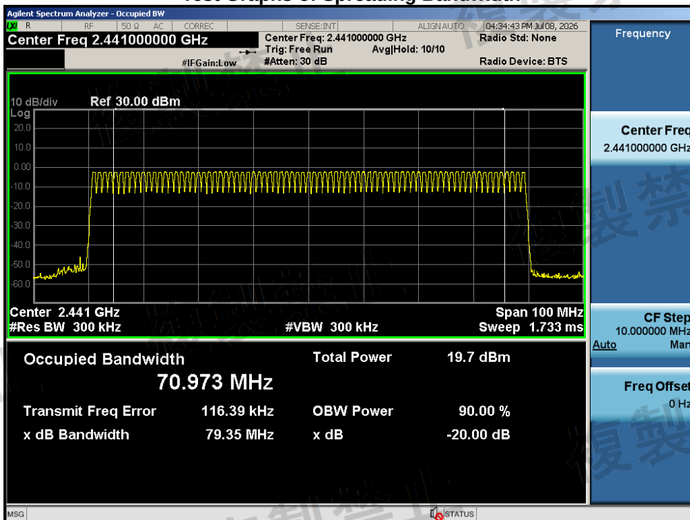
Test_Graph_BR_HOP_ANT1_NA_1Mbps_Spreading Bandwidth_HV
