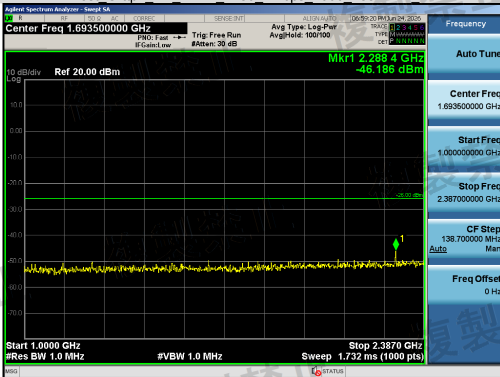
Test_Graph_BR_ANT1_2480_1Mbps_1000_2387MHz_NV
