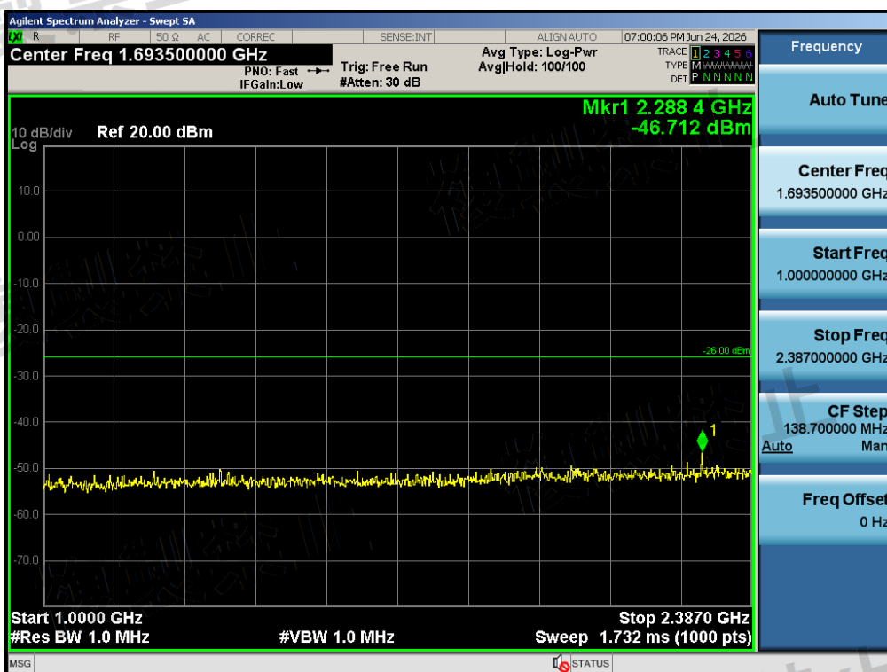
Test Graph BR ANT1 2480 1Mbps 1000 2387MHz LV
