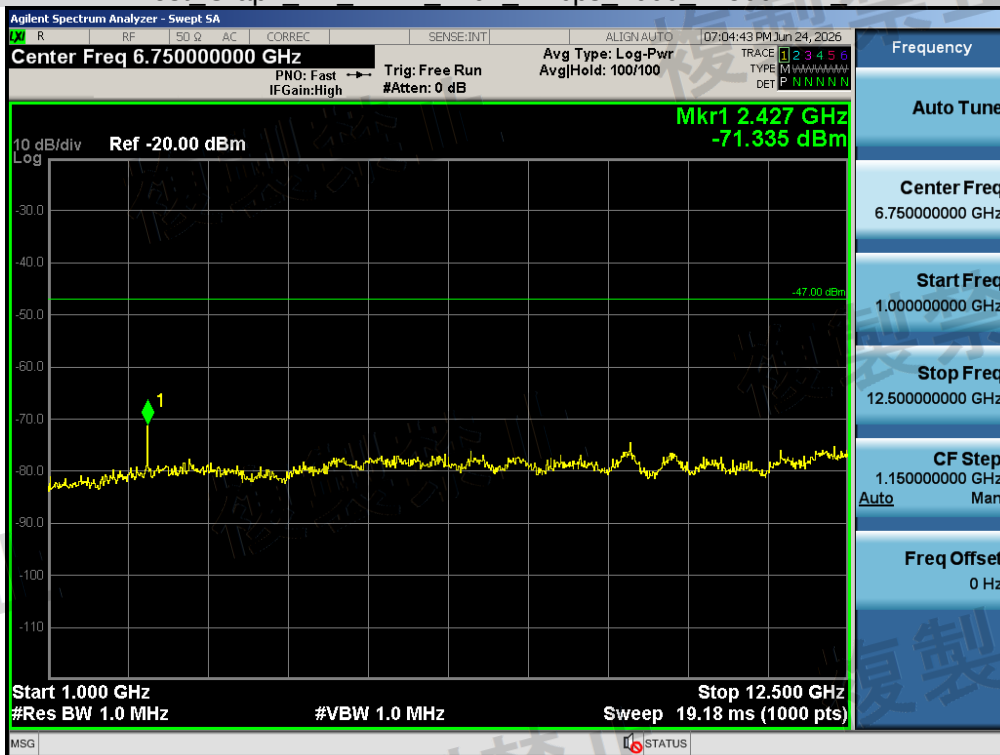
Test_Graph_RX_ANT1_2402_1Mbps_1000_12500MHz_NV
