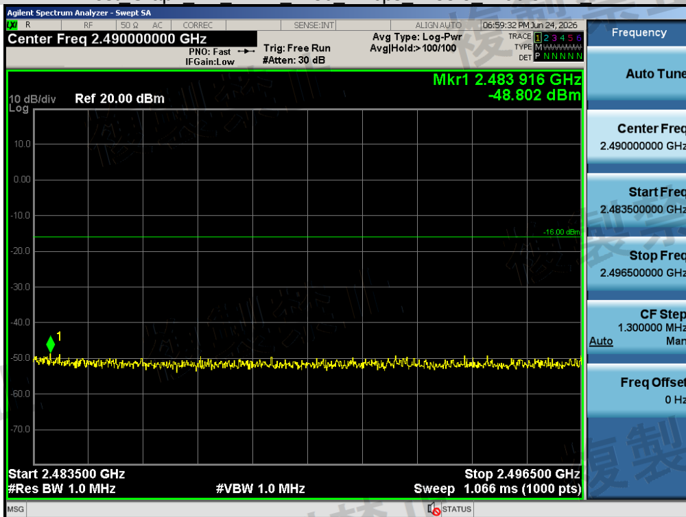
Test_Graph_BR_ANT1_2480_1Mbps_2483.5_2496.5MHz_NV
