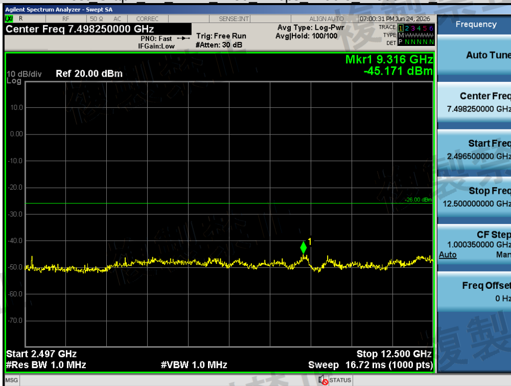
Test Graph BR ANT1 2480 1Mbps 2496.5 12500MHz LV
