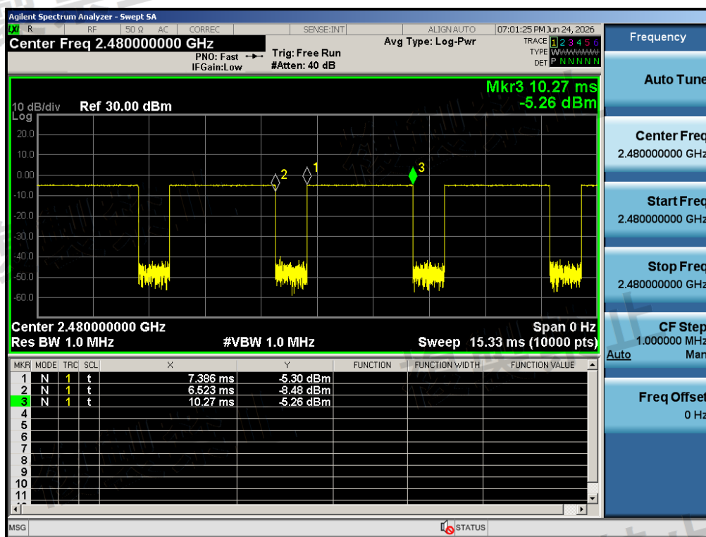
Test_Graph_BR_ANT1_2480_1Mbps_2480_DT
