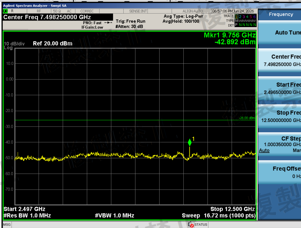
Test Graph BR ANT1 2441 1Mbps 2496.5 12500MHz NV
