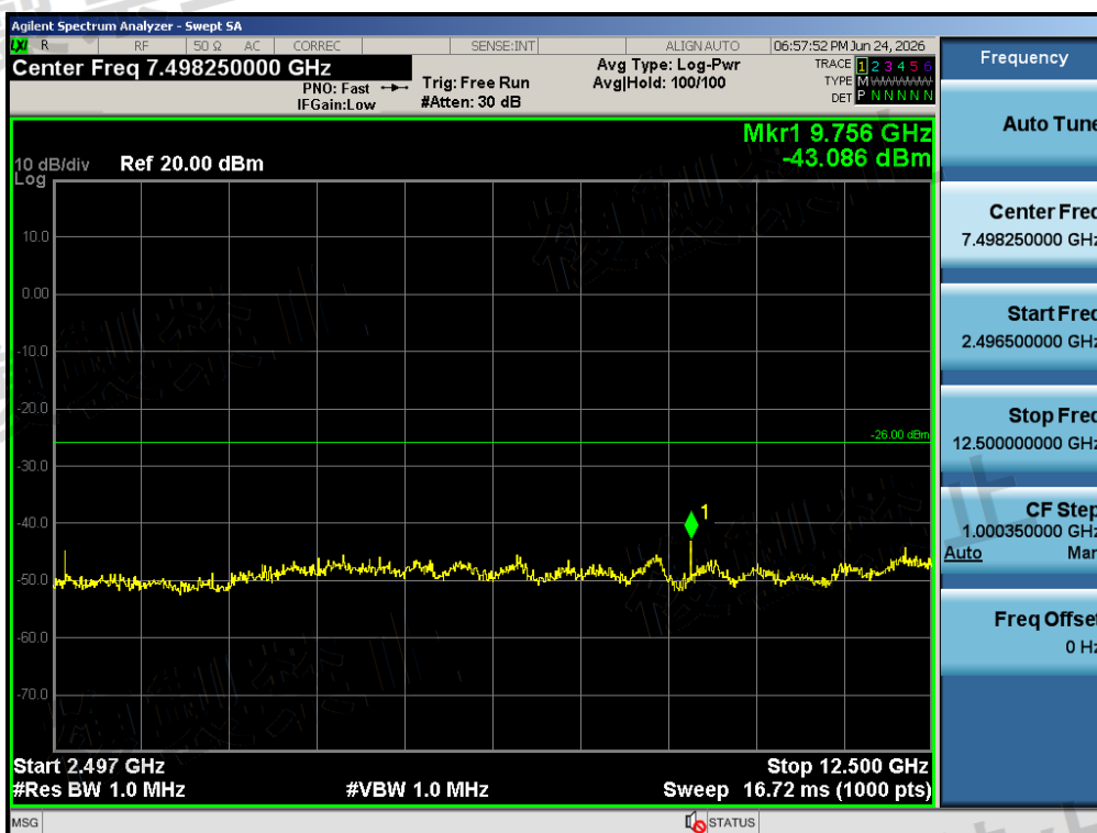
Test Graph BR ANT1 2441 1Mbps 2496.5 12500MHz LV
