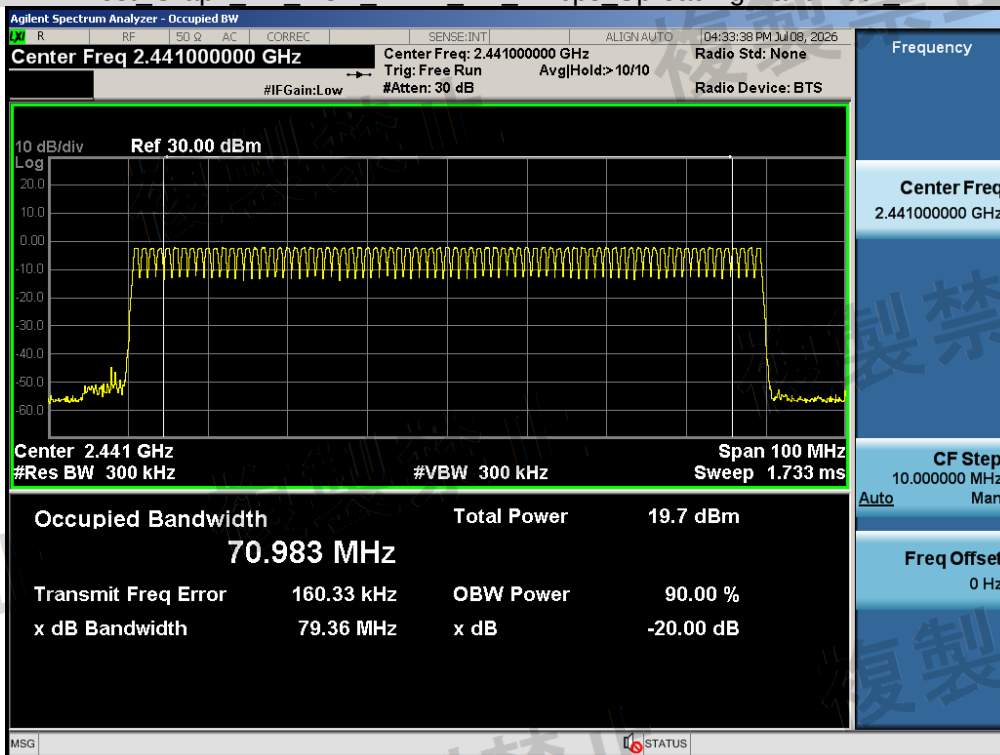
Test_Graph_BR_HOP_ANT1_NA_1Mbps_Spreading Bandwidth_NV
