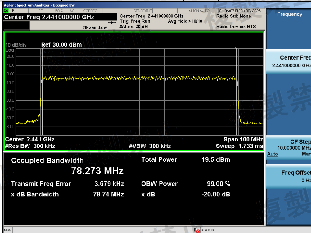
Test Graph EDR HOP ANT1 NA 2Mbps Occupied Bandwidth NV
