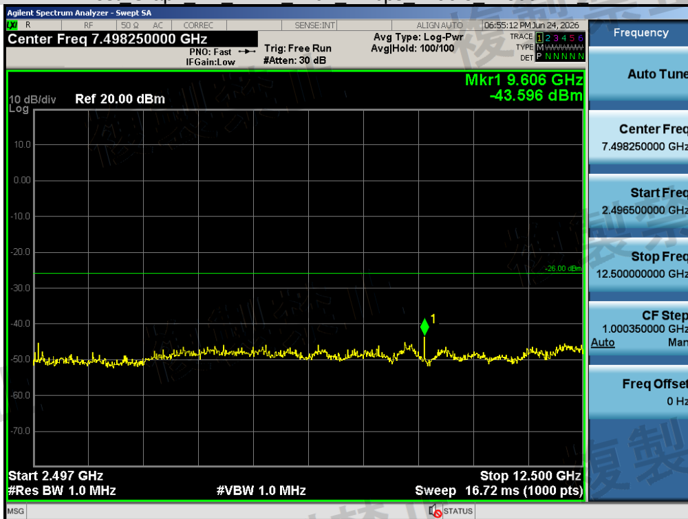
Test Graph BR ANT1 2402 1Mbps 2496.5 12500MHz LV
