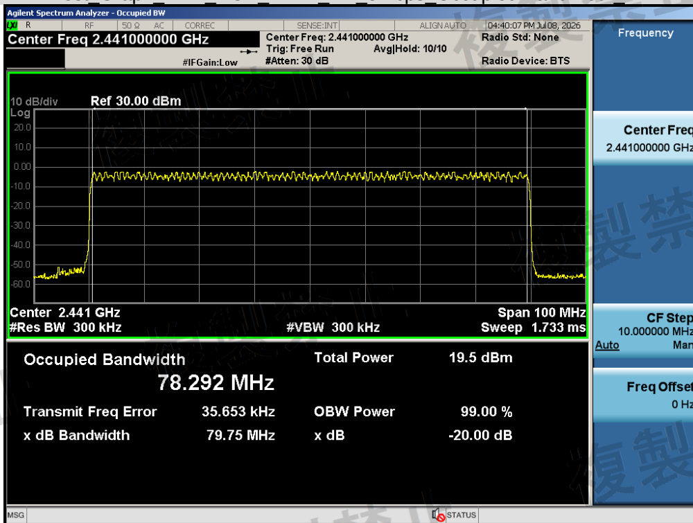
Test_Graph_EDR_HOP_ANT1_NA_3Mbps_Occupied Bandwidth_LV
