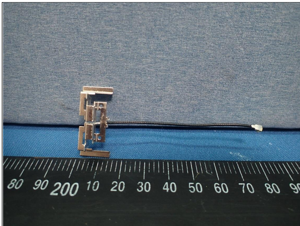
Antenna No.: 1
